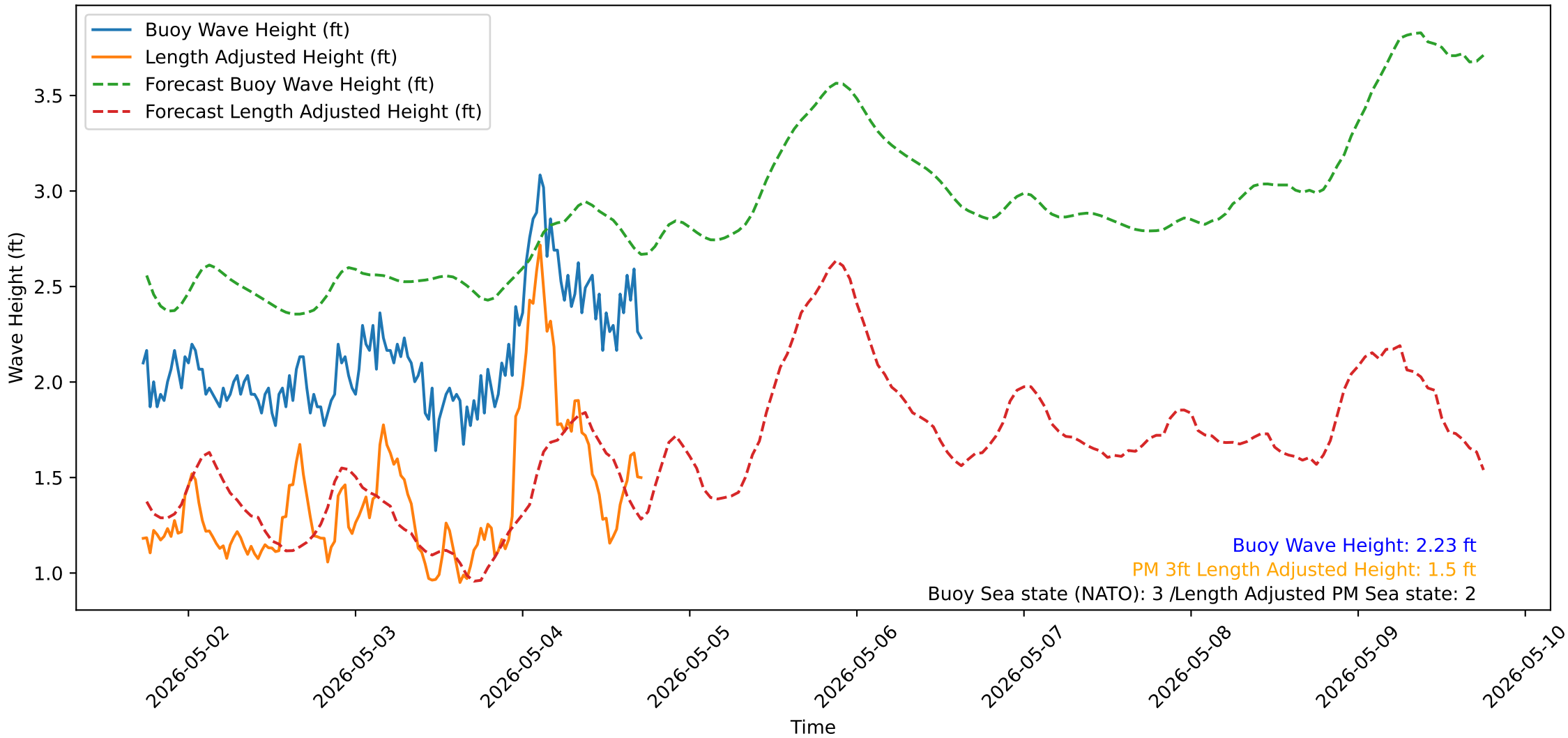
Wave Heights over Time for Oceanside Harbor at 2026-05-04 17:40:32
