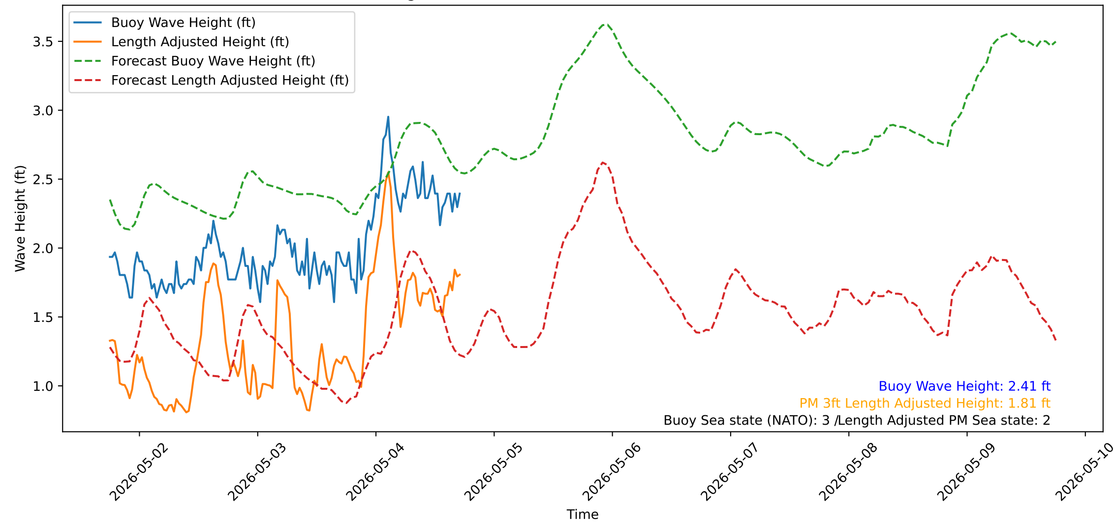
Wave Heights over Time for Red Beach at 2026-05-04 17:40:51
