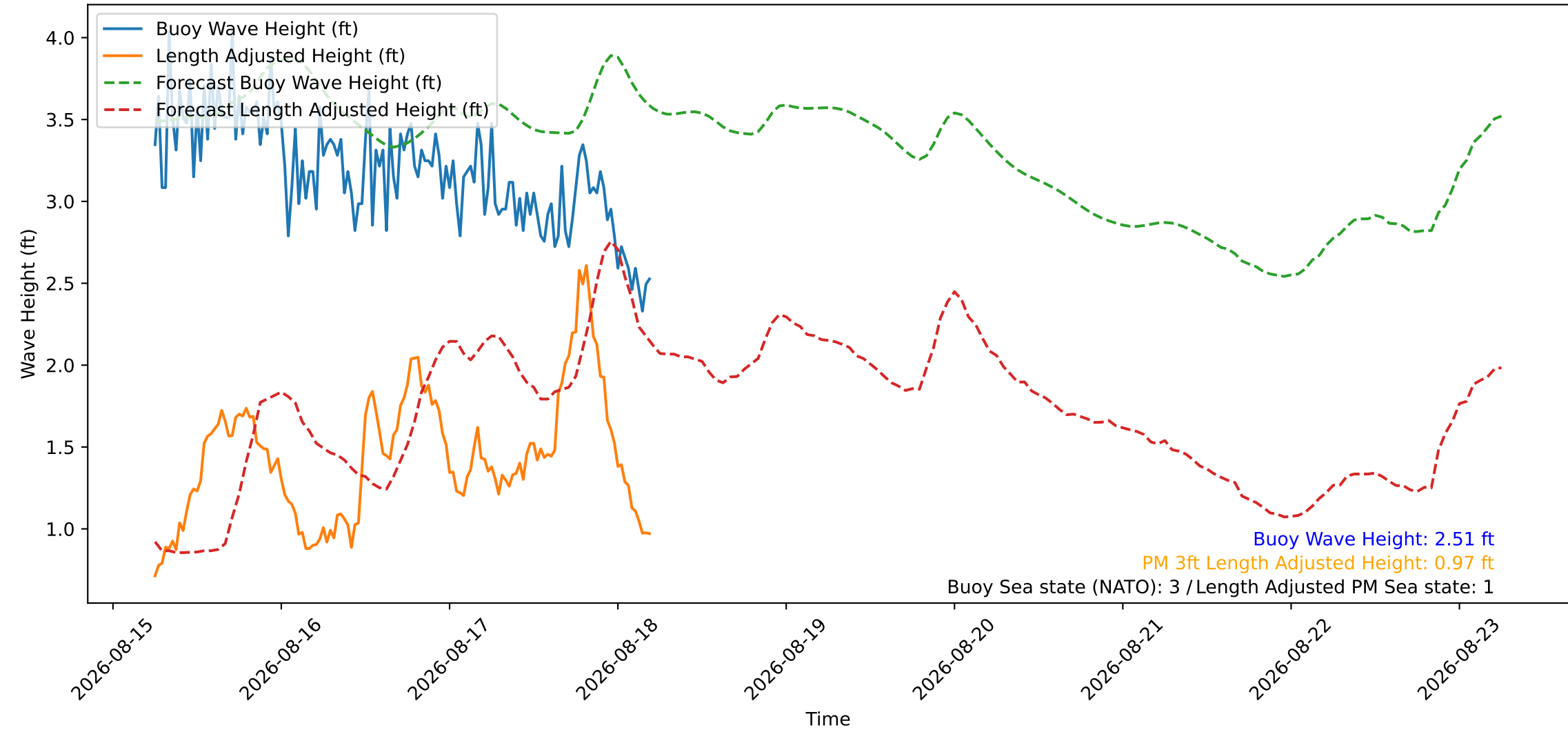
Wave Heights over Time for Red Beach at 2026-08-18 05:30:46
