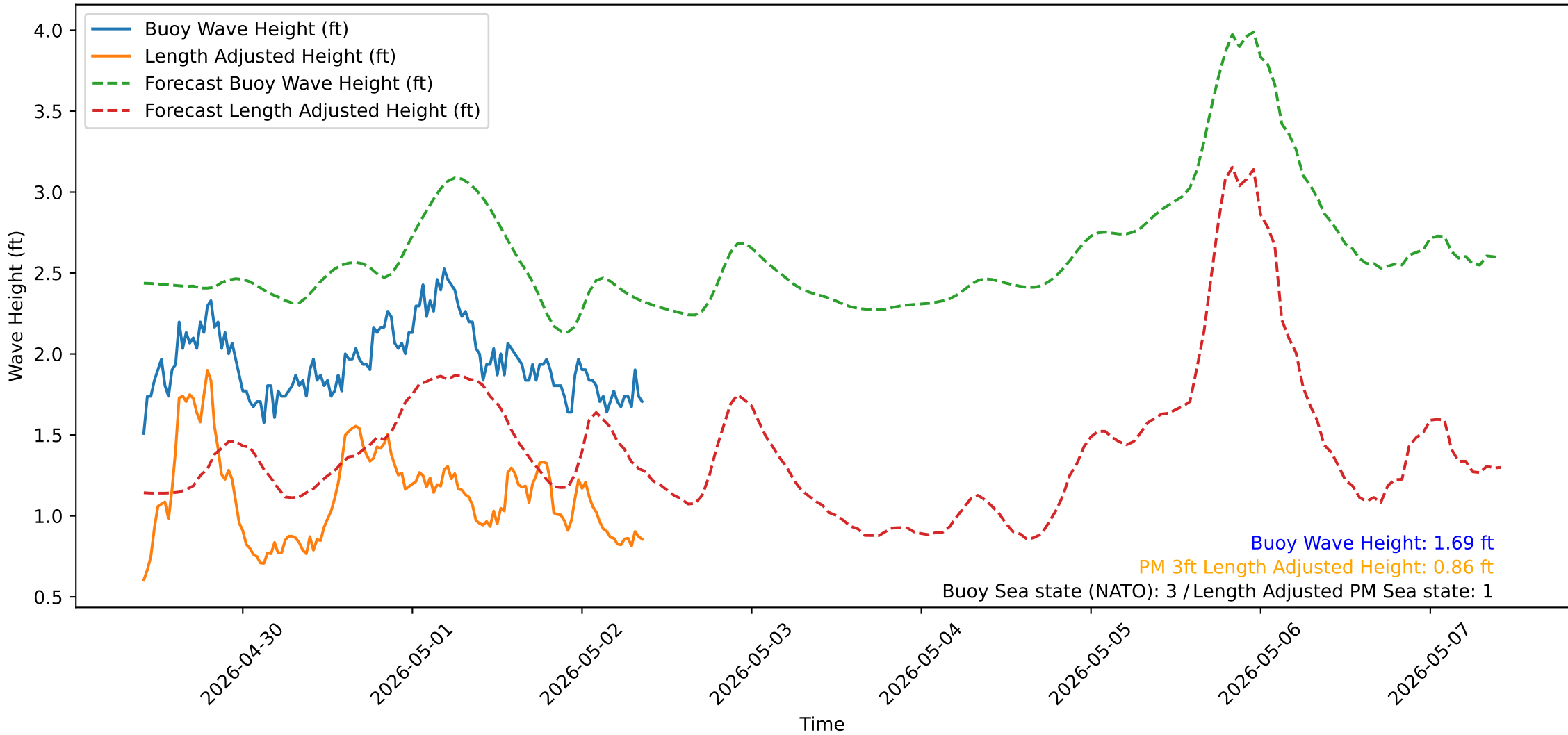
Wave Heights over Time for Red Beach at 2026-05-02 09:30:51
