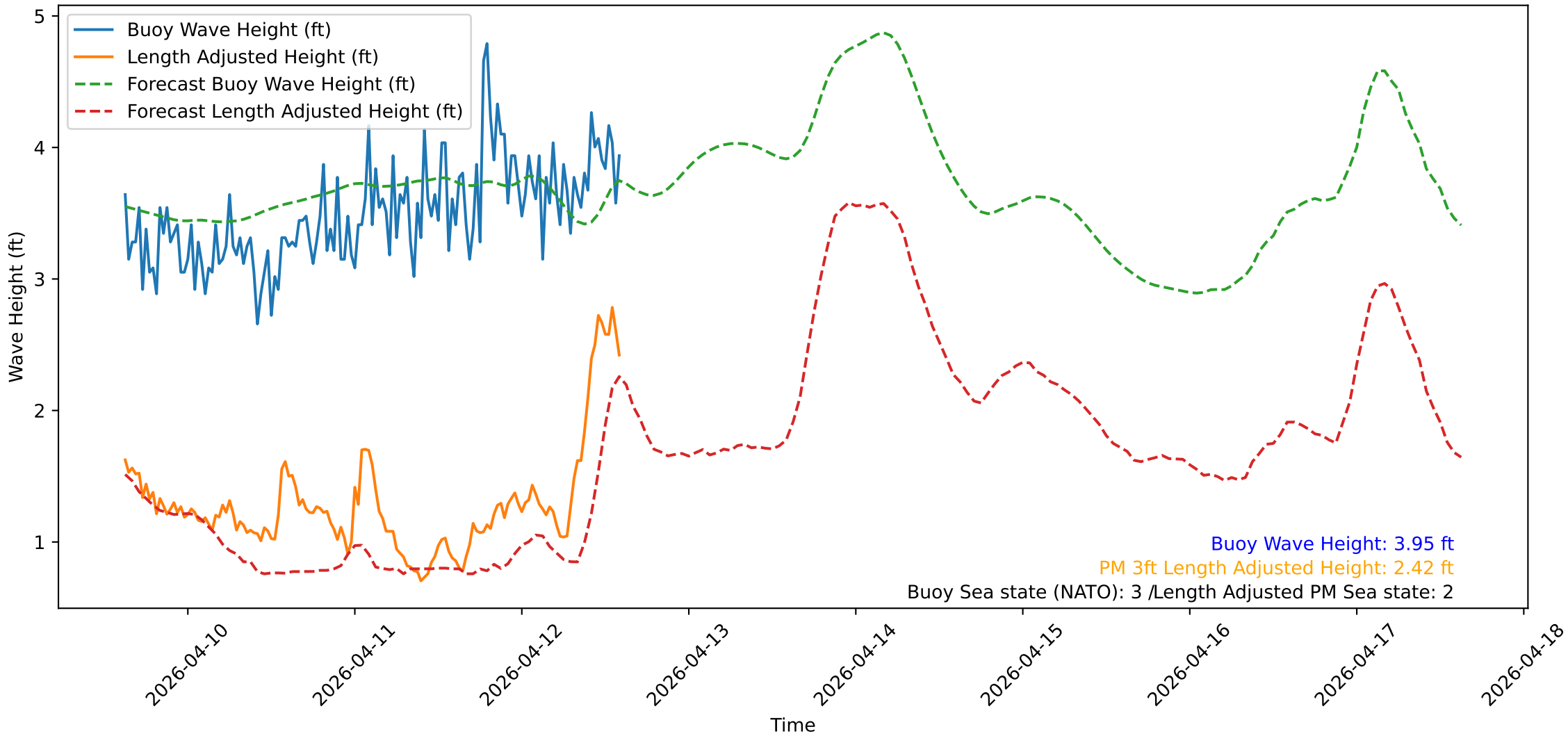
Wave Heights over Time for Oceanside Harbor at 2026-04-12 15:00:31
