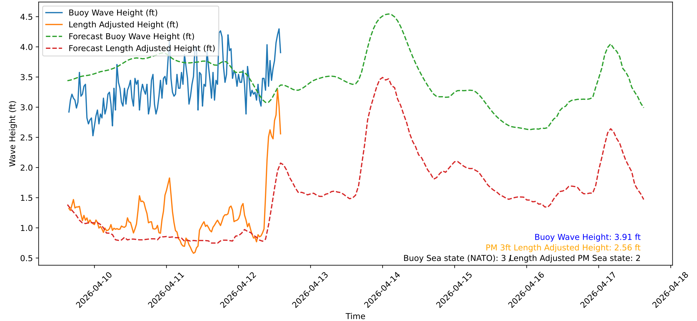
Wave Heights over Time for Red Beach at 2026-04-12 15:00:50
