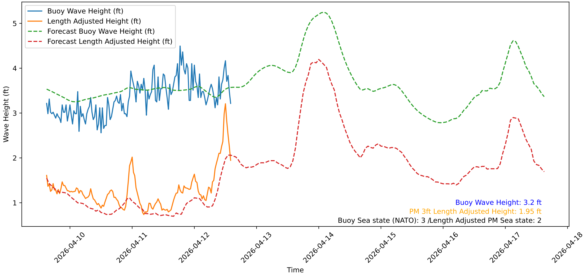
Wave Heights over Time for Green Beach at 2026-04-12 15:01:13
