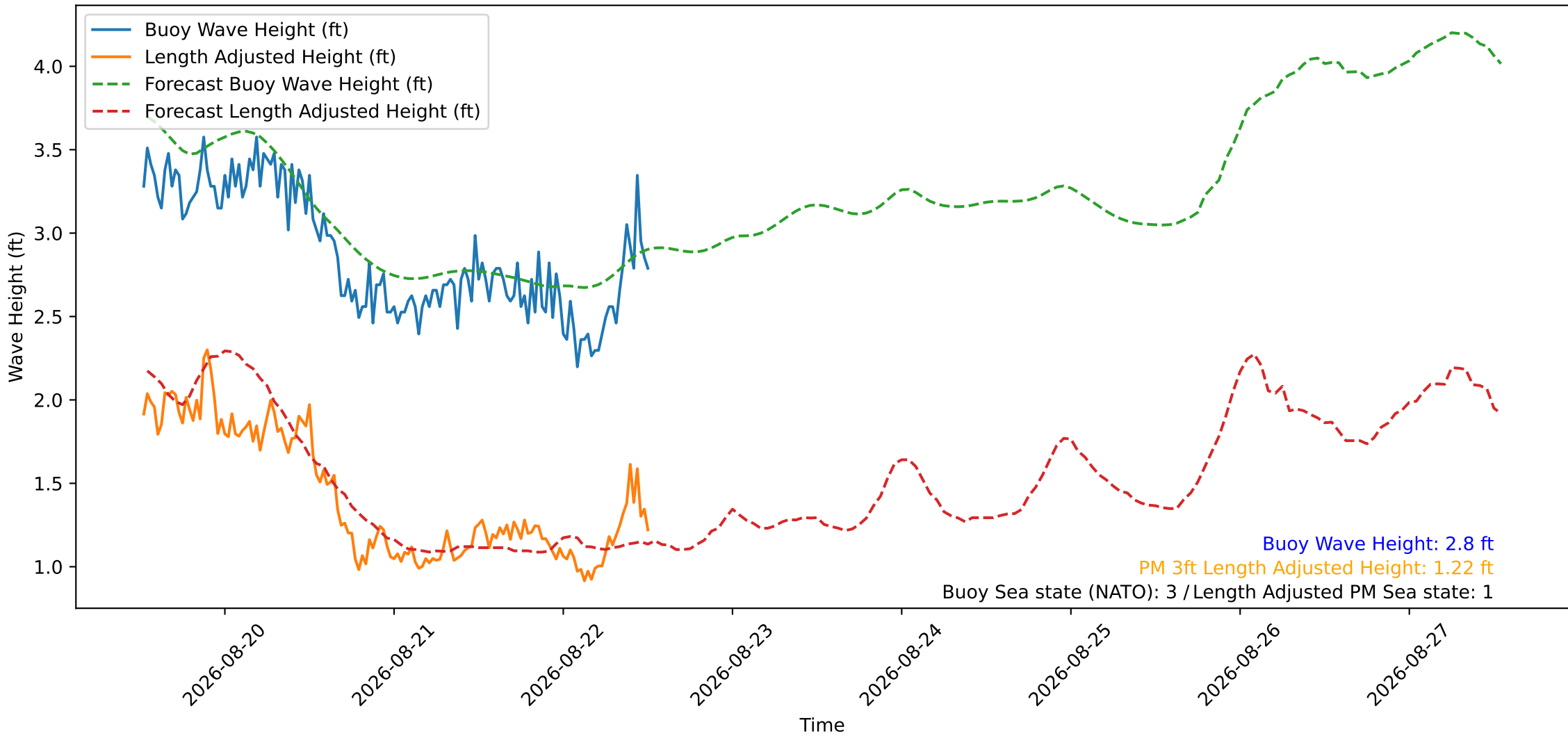
Wave Heights over Time for Oceanside Harbor at 2026-08-22 12:30:29
