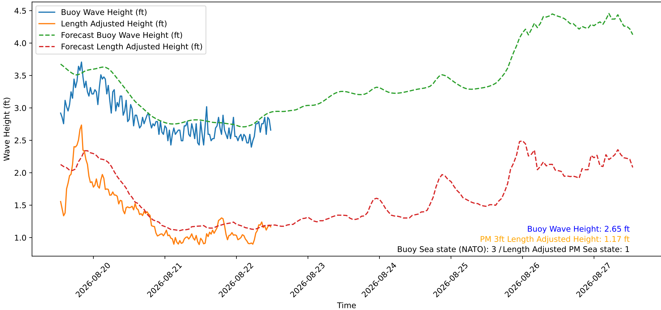
Wave Heights over Time for Green Beach at 2026-08-22 12:31:11
