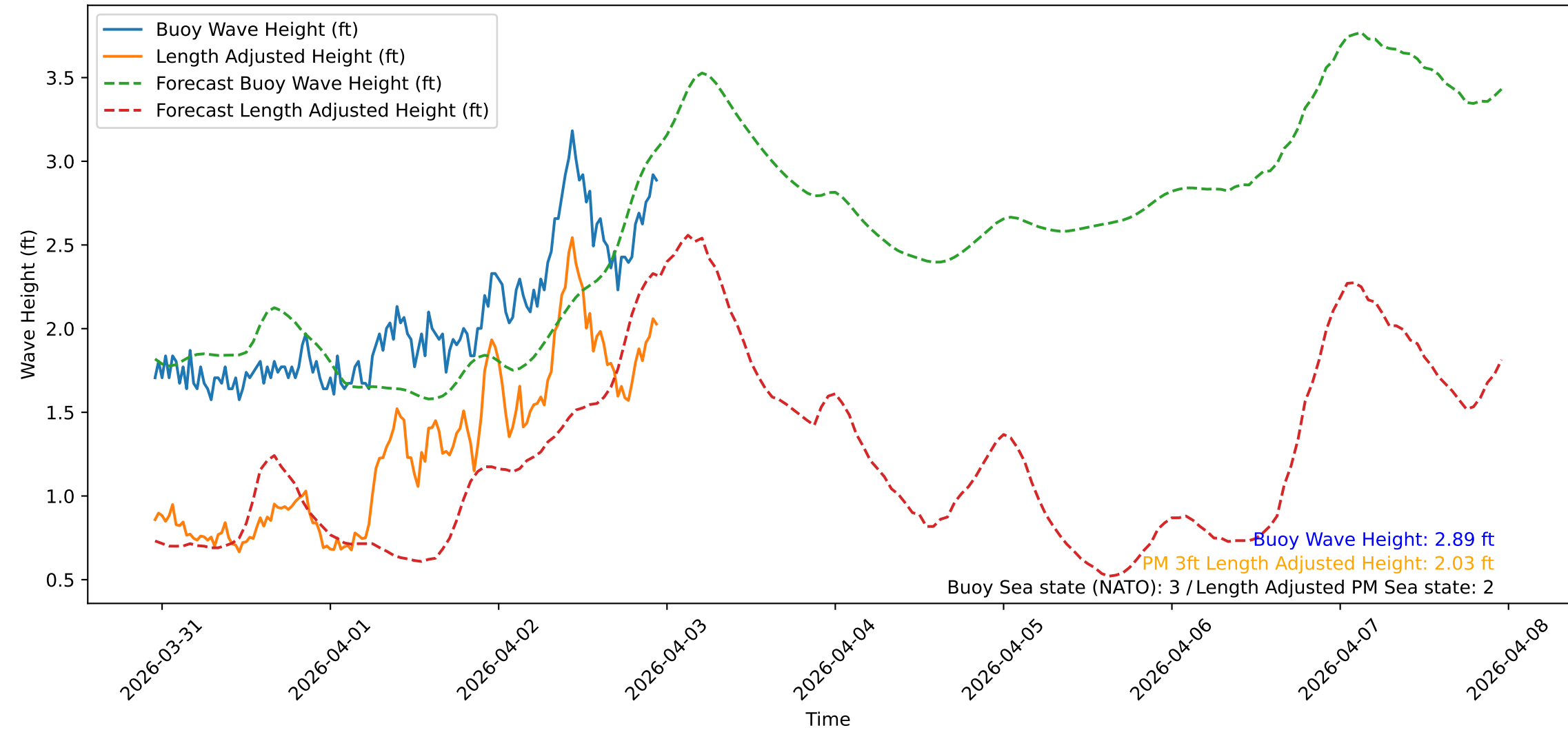
Wave Heights over Time for Oceanside Harbor at 2026-04-02 23:10:31
