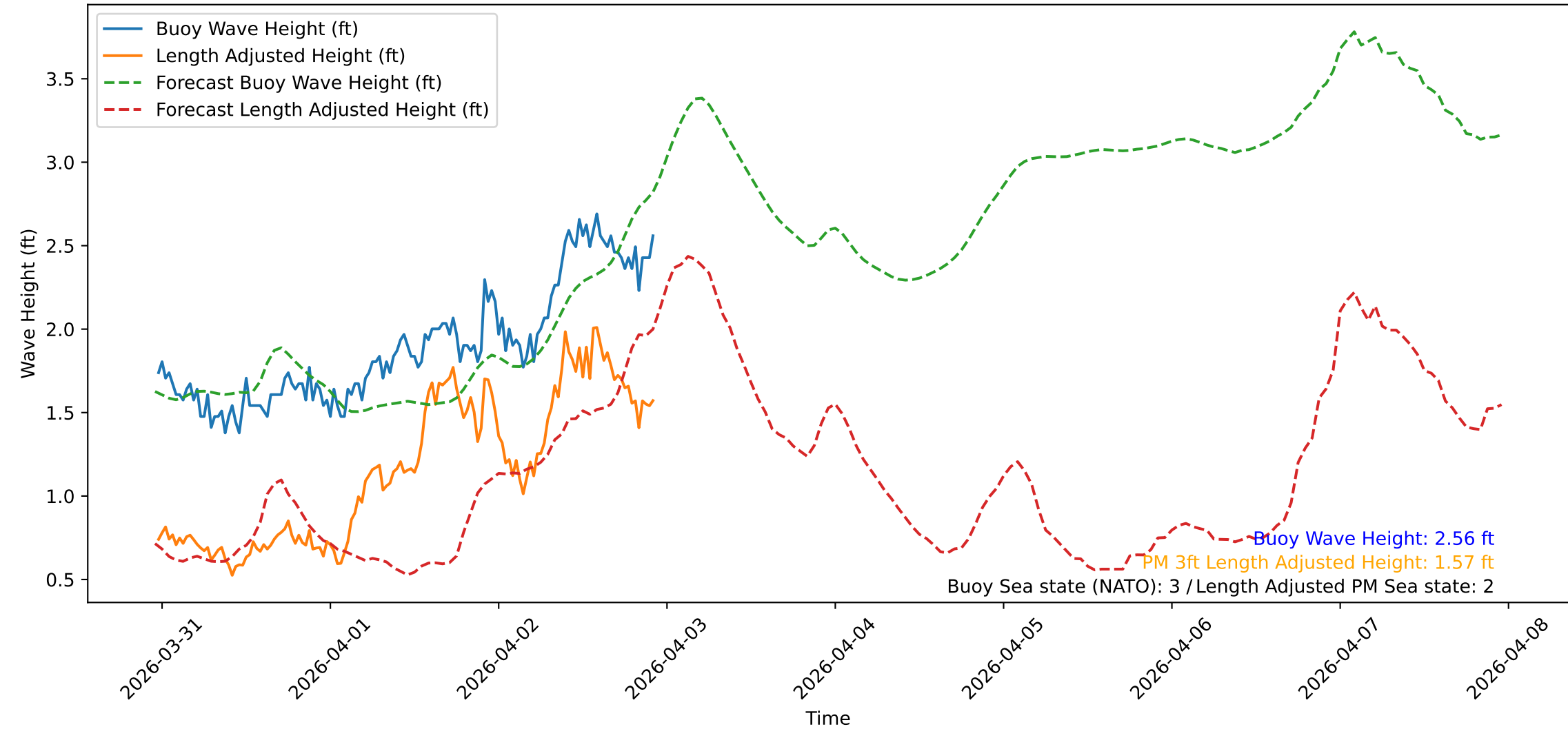
Wave Heights over Time for Red Beach at 2026-04-02 23:10:47
