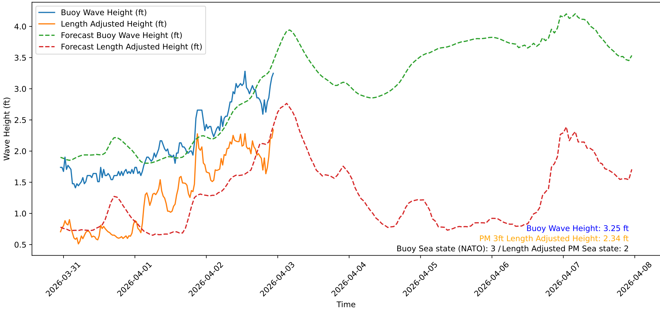
Wave Heights over Time for Green Beach at 2026-04-02 23:11:10
