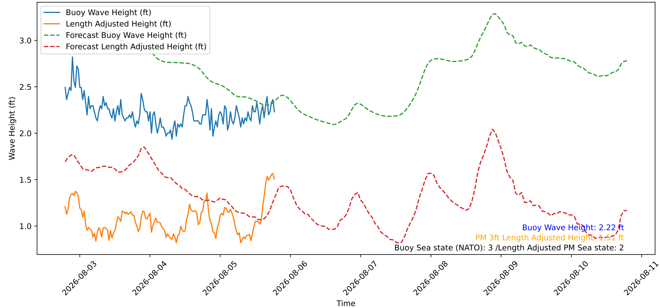
Wave Heights over Time for Green Beach at 2026-08-05 19:11:09
