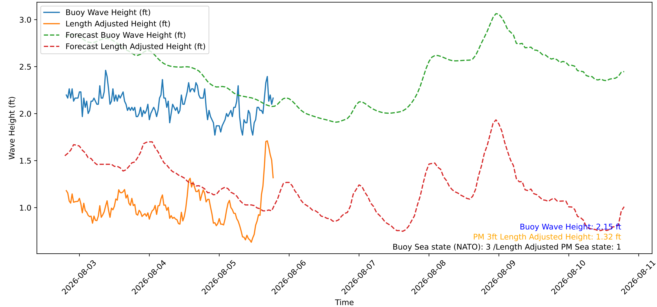
Wave Heights over Time for Red Beach at 2026-08-05 19:10:46
