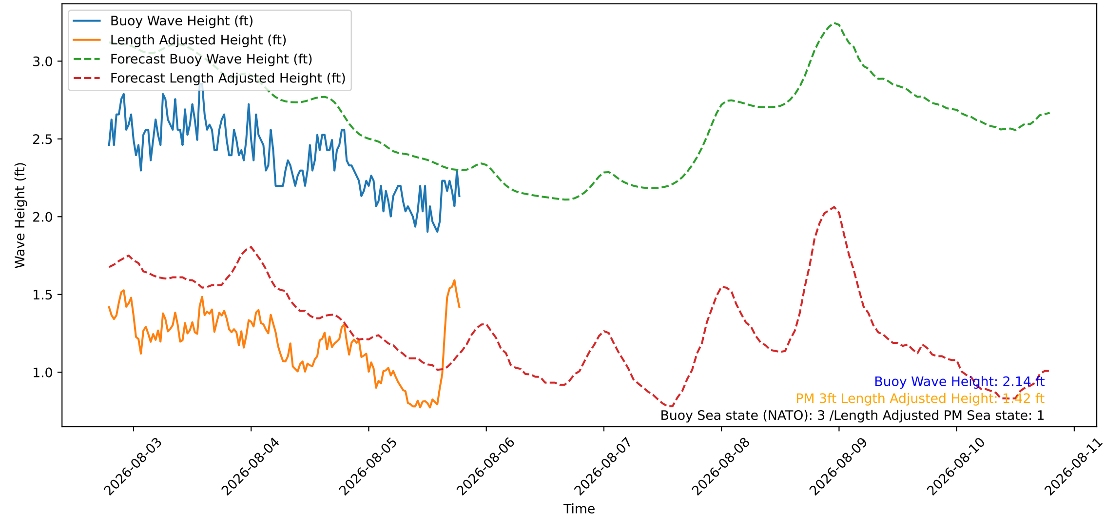
Wave Heights over Time for Oceanside Harbor at 2026-08-05 19:10:27
