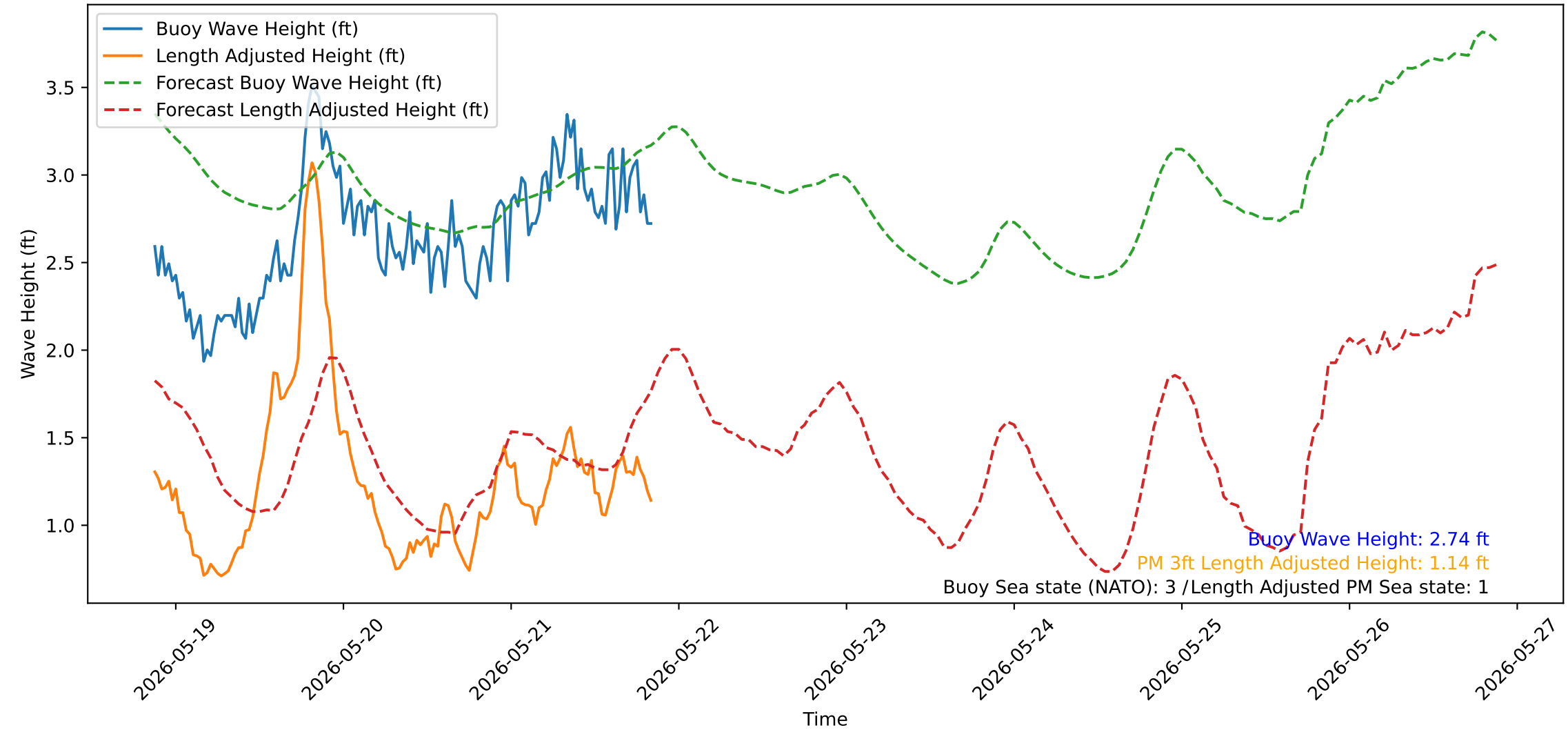
Wave Heights over Time for Red Beach at 2026-05-21 20:50:51
