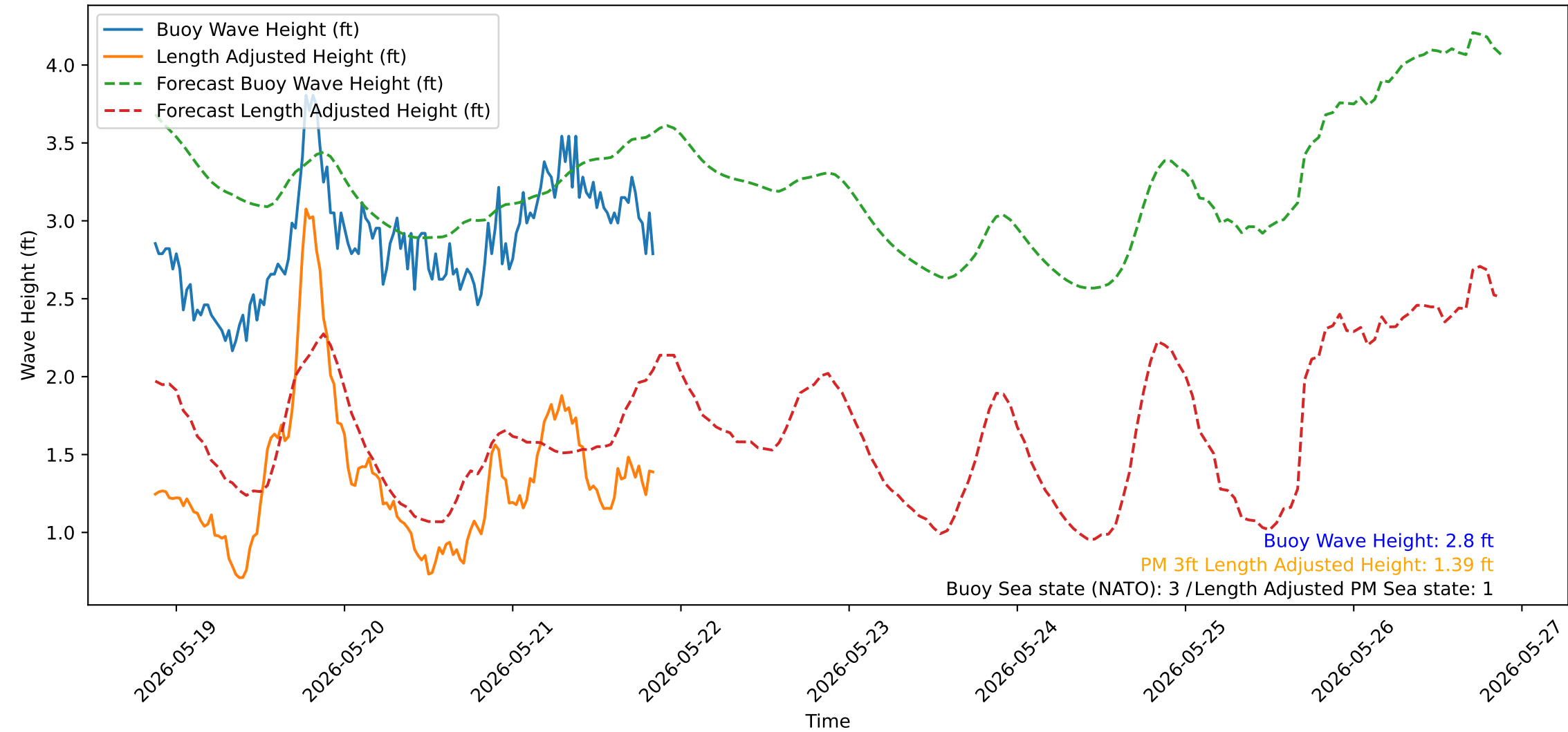
Wave Heights over Time for Green Beach at 2026-05-21 20:51:14
