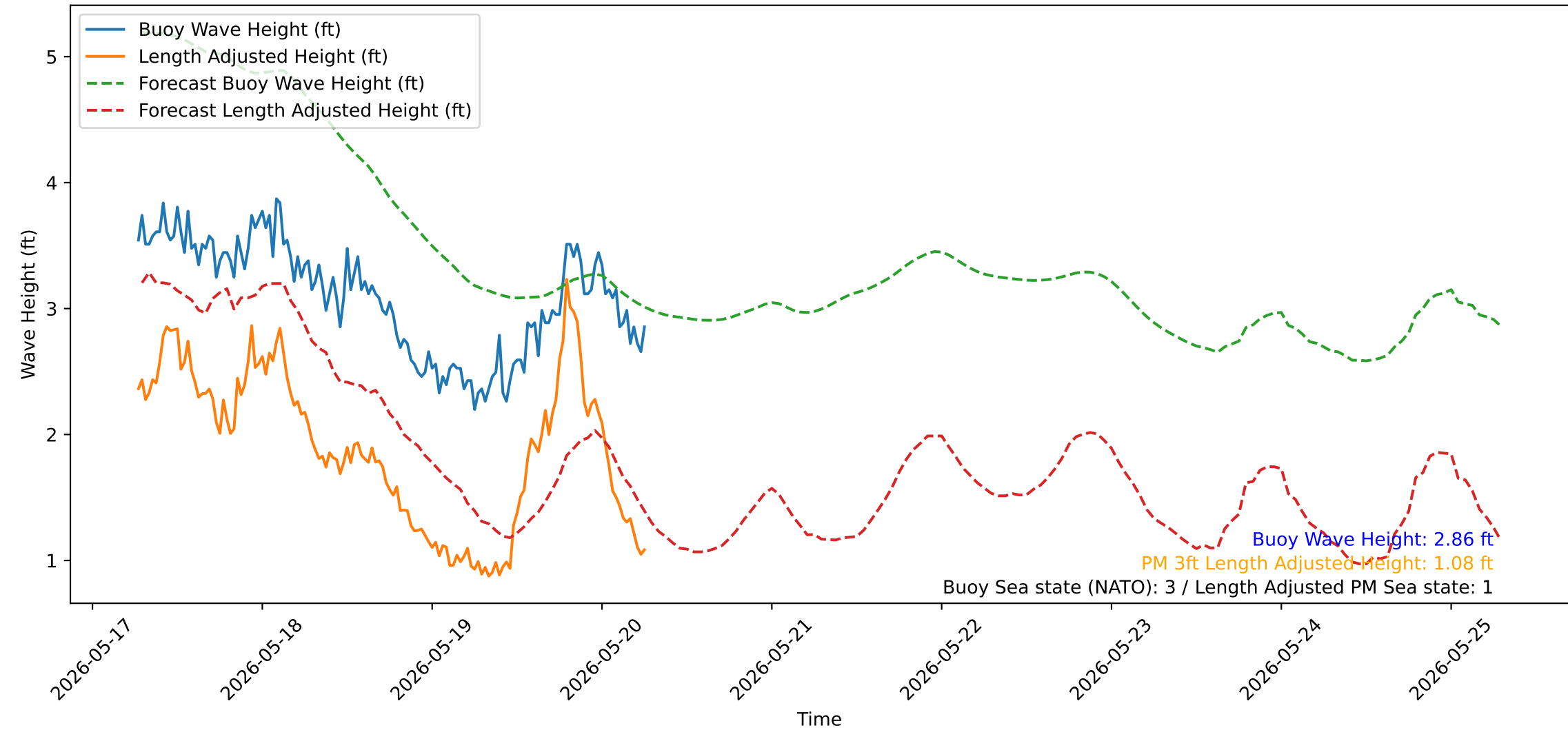
Wave Heights over Time for Oceanside Harbor at 2026-05-20 06:40:30
