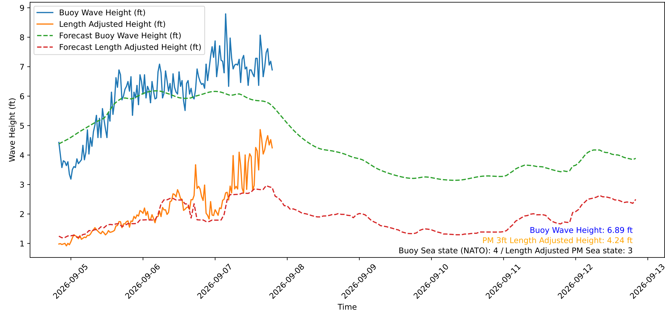
Wave Heights over Time for Green Beach at 2026-09-07 19:51:13
