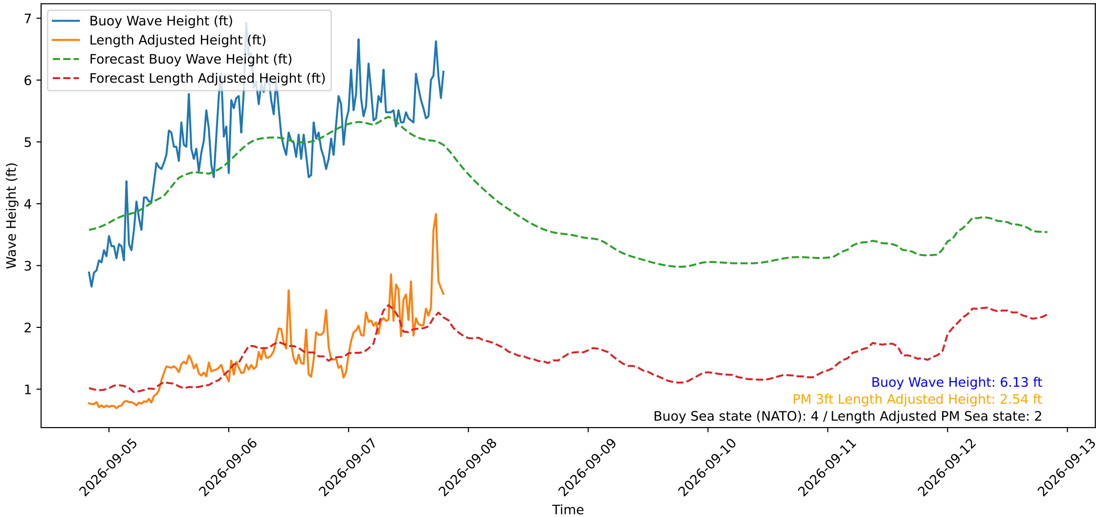
Wave Heights over Time for Red Beach at 2026-09-07 19:50:49
