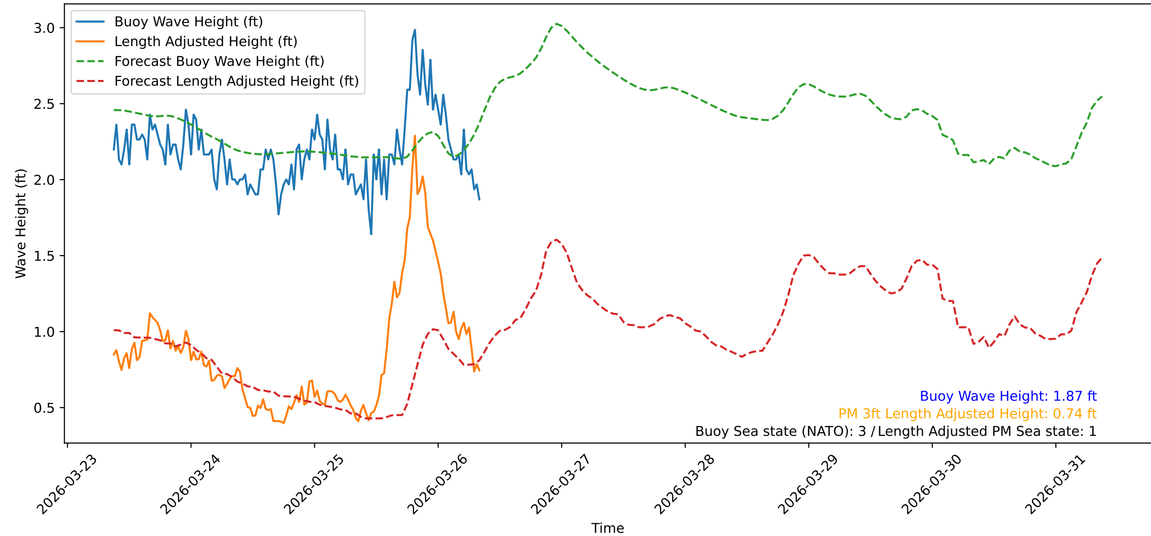
Wave Heights over Time for Green Beach at 2026-03-26 09:01:10
