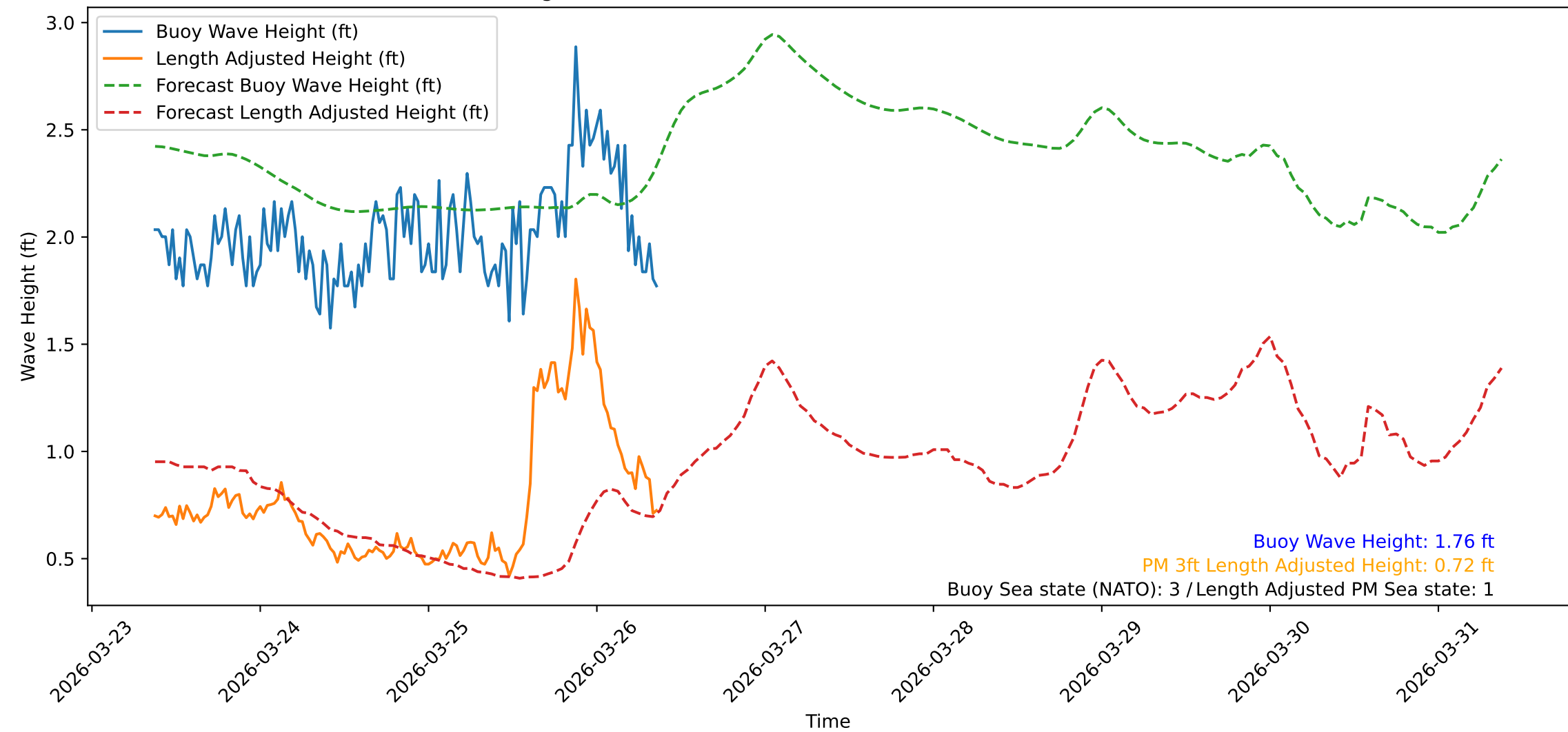
Wave Heights over Time for Oceanside Harbor at 2026-03-26 09:00:32
