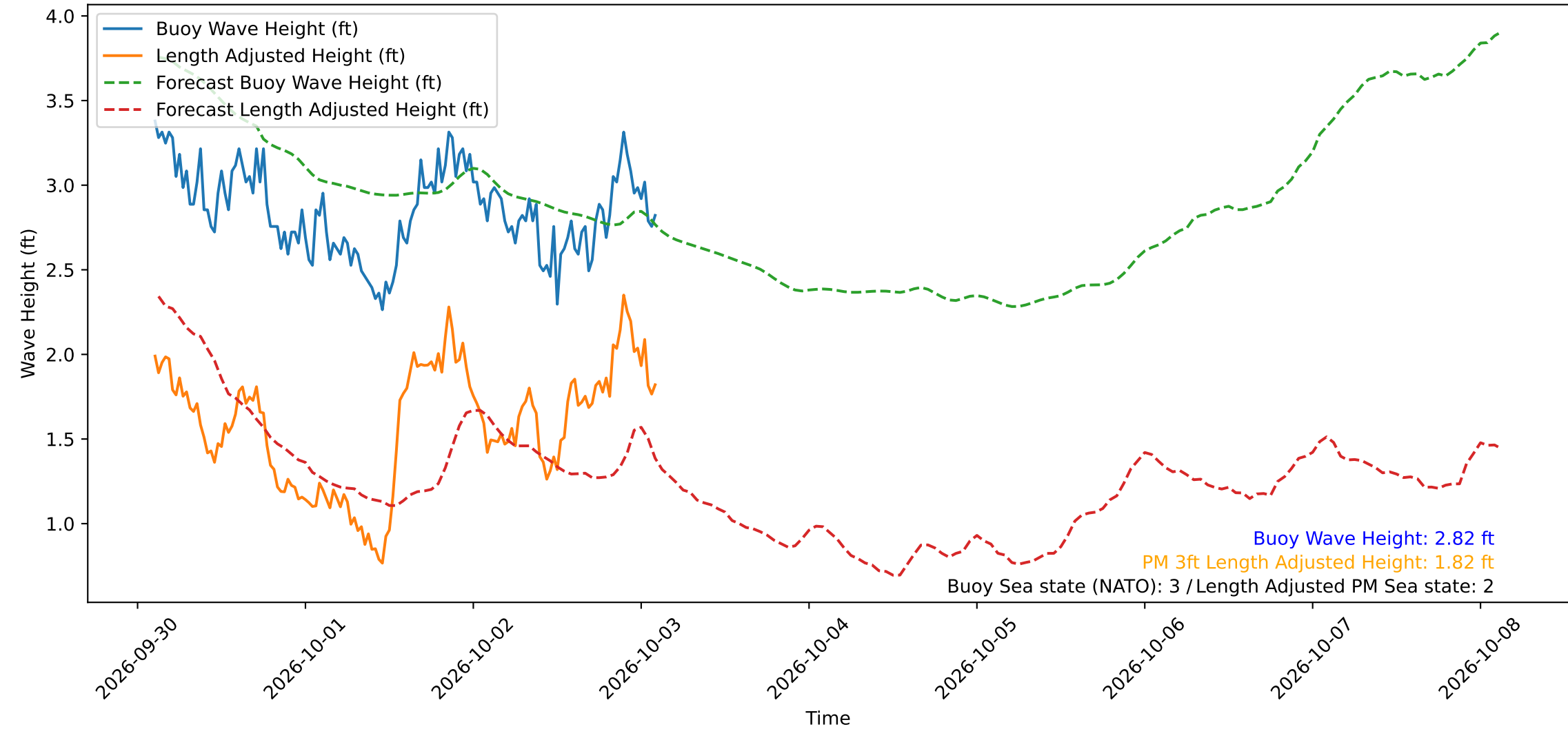
Wave Heights over Time for Oceanside Harbor at 2026-10-03 02:40:29
