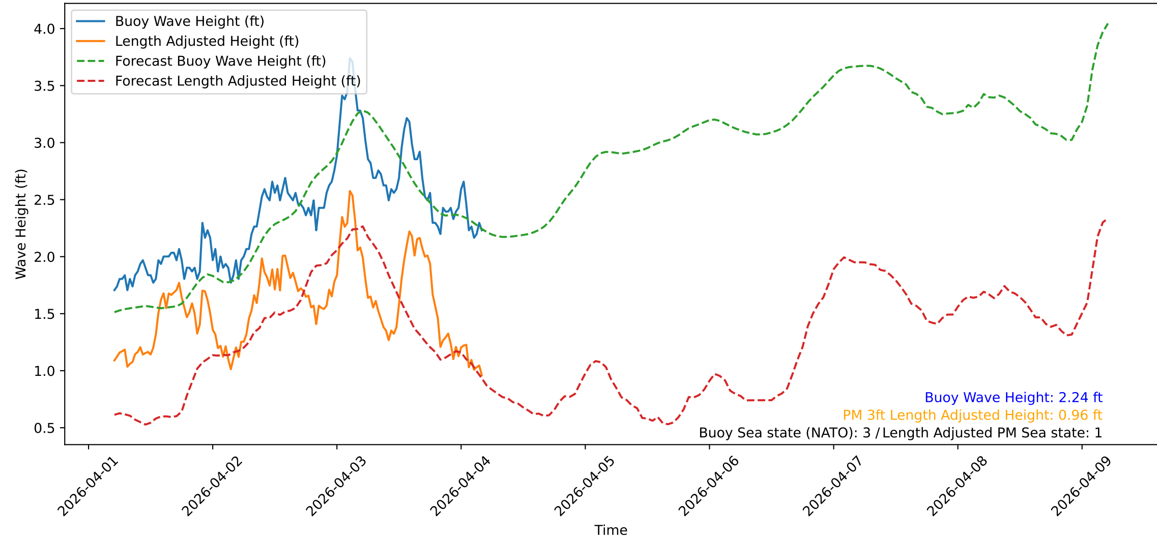
Wave Heights over Time for Red Beach at 2026-04-04 04:40:48
