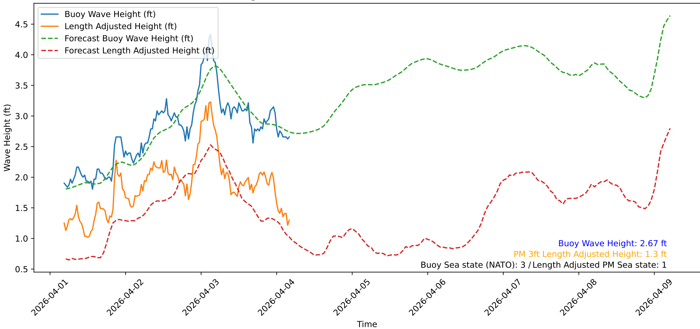
Wave Heights over Time for Green Beach at 2026-04-04 04:41:11
