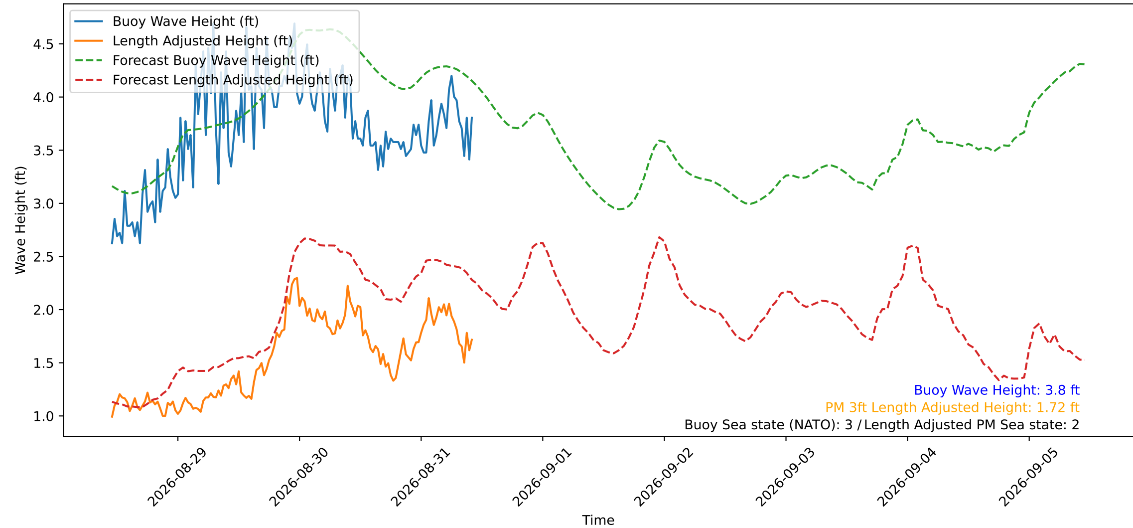
Wave Heights over Time for Red Beach at 2026-08-31 10:50:49
