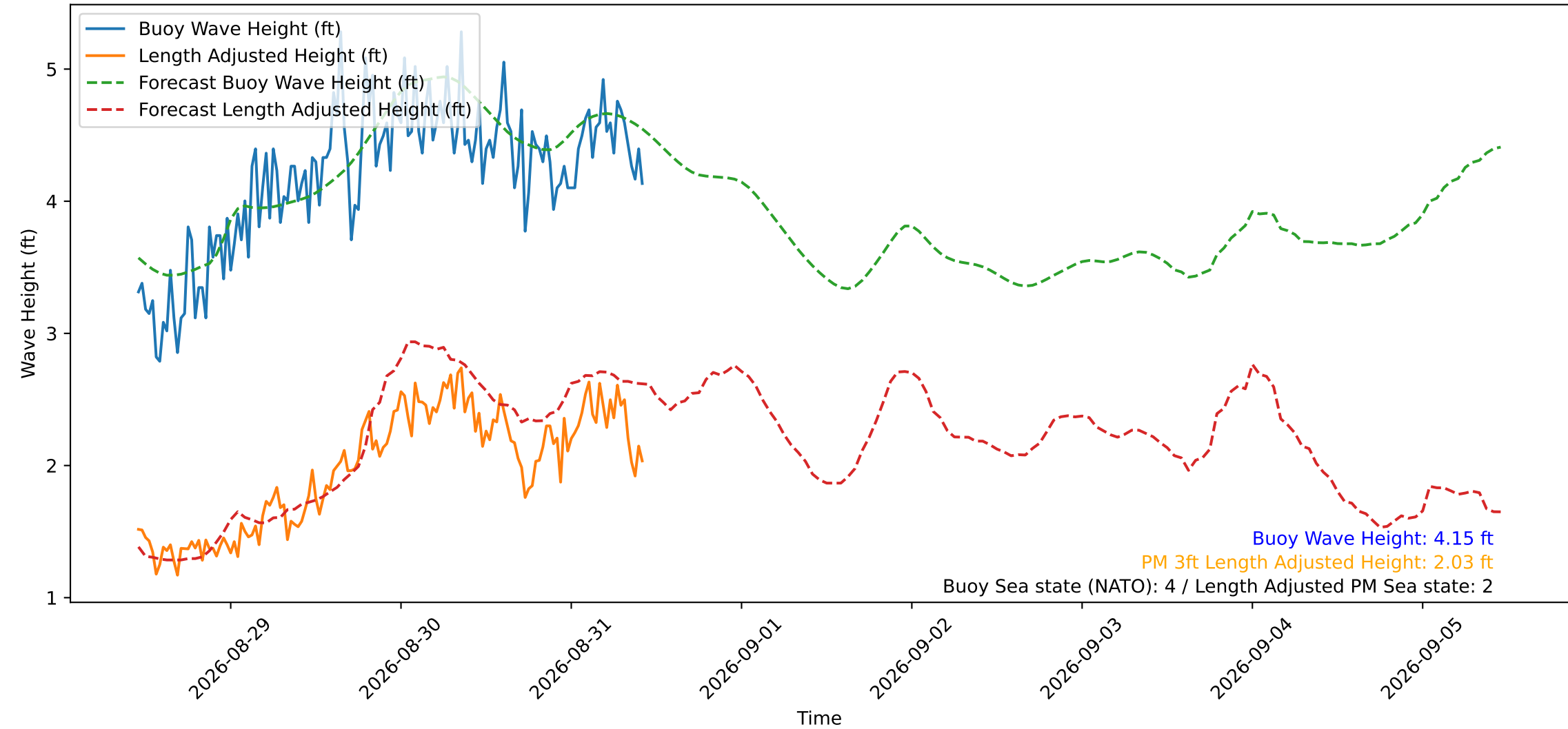
Wave Heights over Time for Oceanside Harbor at 2026-08-31 10:50:29
