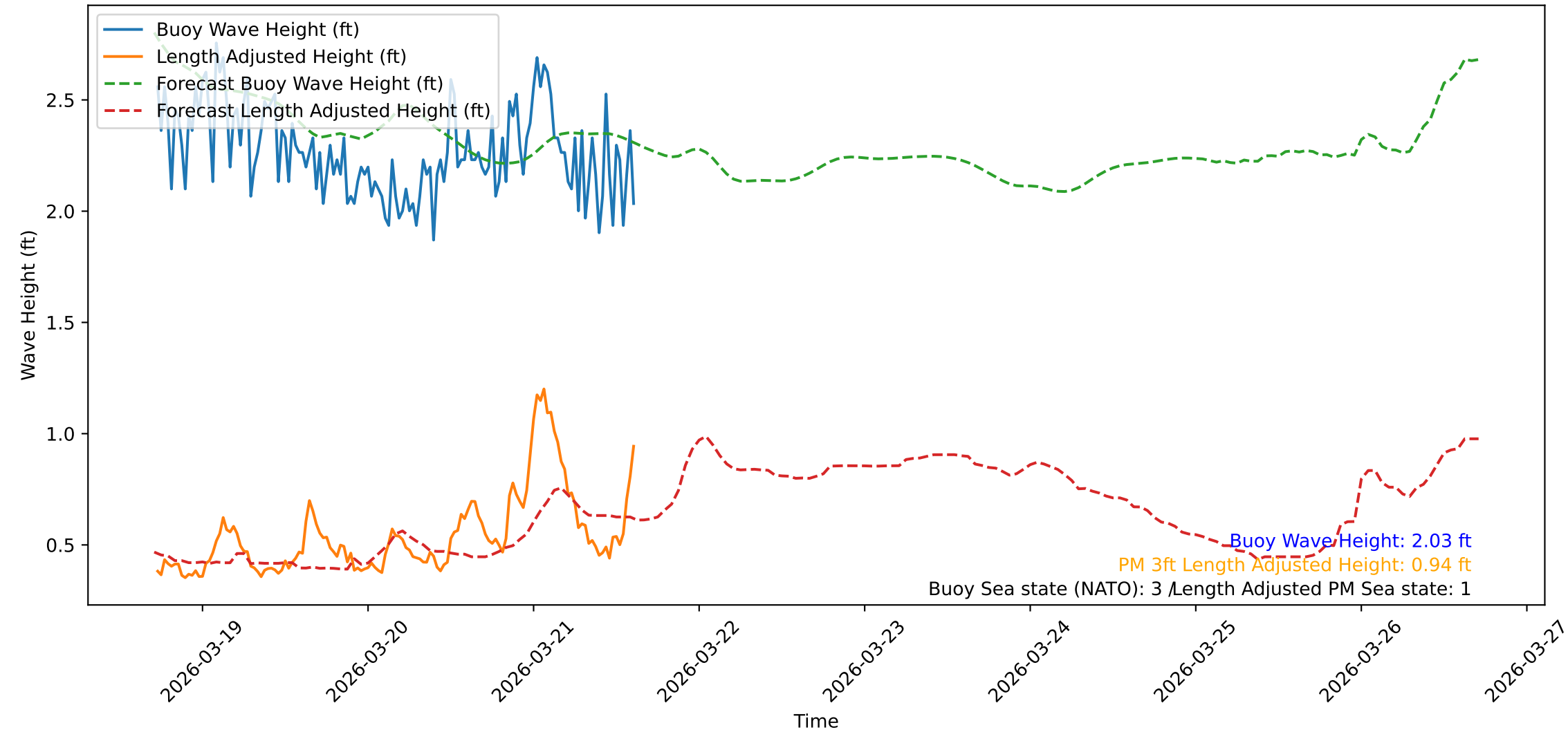
Wave Heights over Time for Red Beach at 2026-03-21 17:10:47
