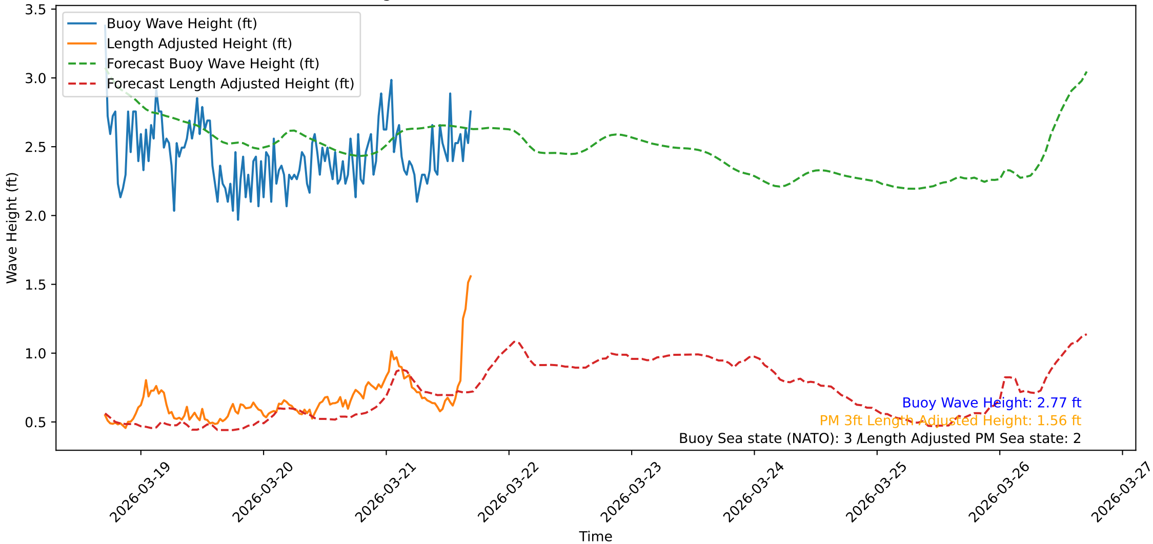
Wave Heights over Time for Oceanside Harbor at 2026-03-21 17:10:31
