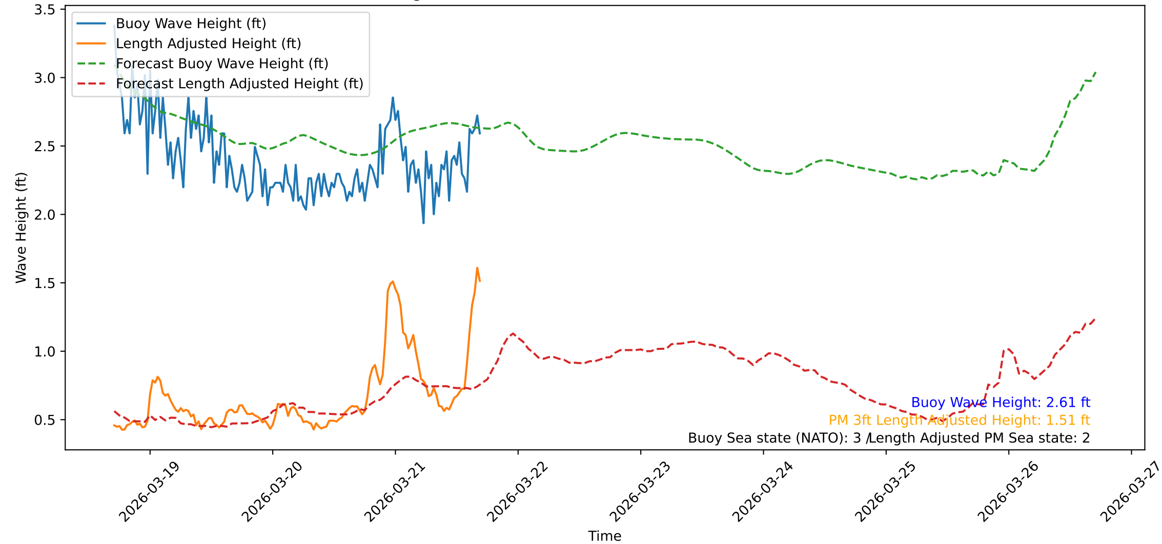
Wave Heights over Time for Green Beach at 2026-03-21 17:11:10
