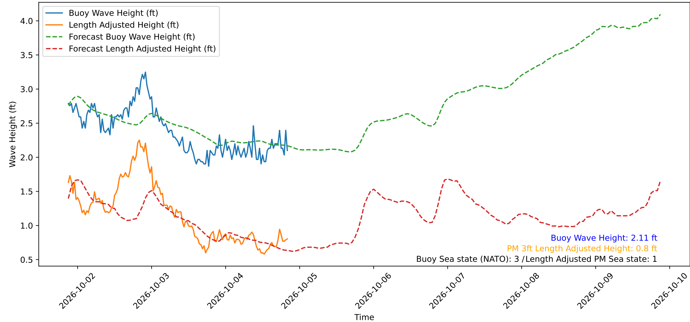
Wave Heights over Time for Red Beach at 2026-10-04 20:40:49
