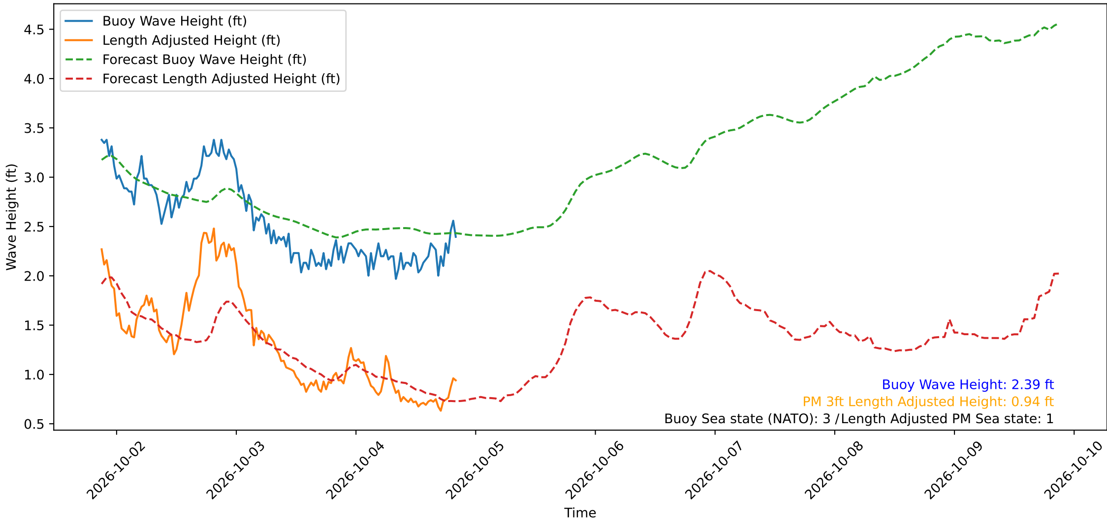
Wave Heights over Time for Green Beach at 2026-10-04 20:41:11
