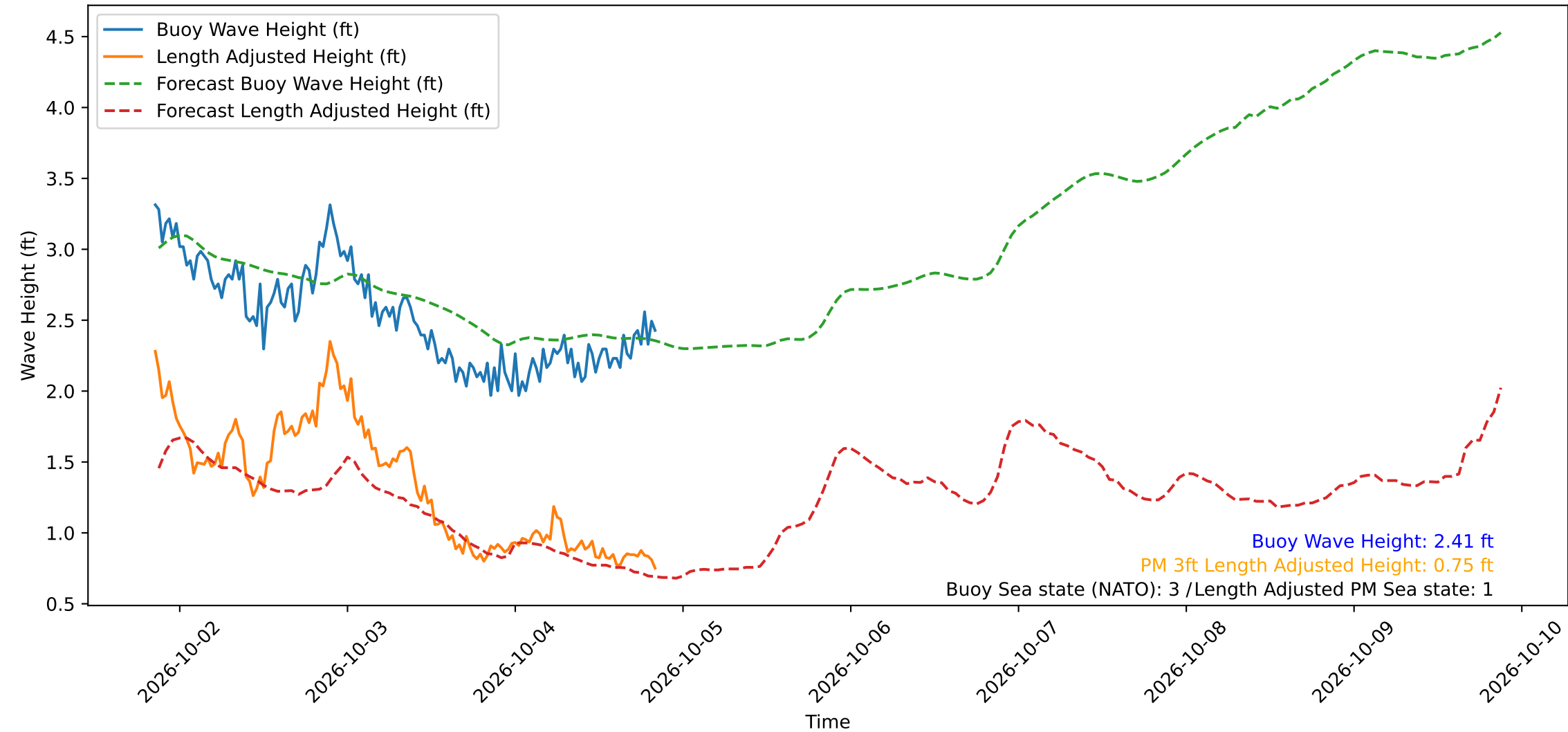
Wave Heights over Time for Oceanside Harbor at 2026-10-04 20:40:29
