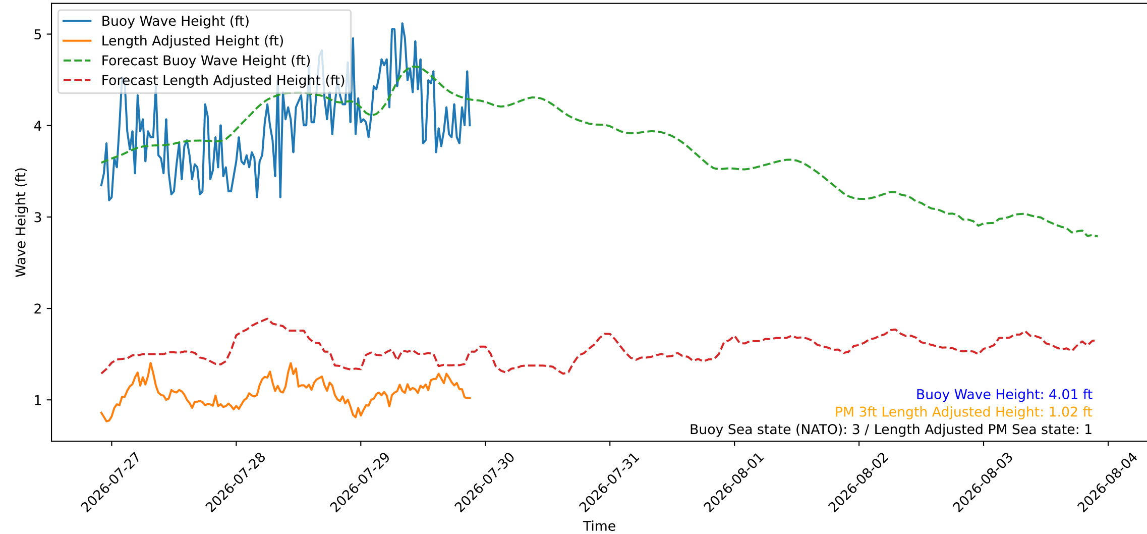
Wave Heights over Time for Red Beach at 2026-07-29 21:40:47
