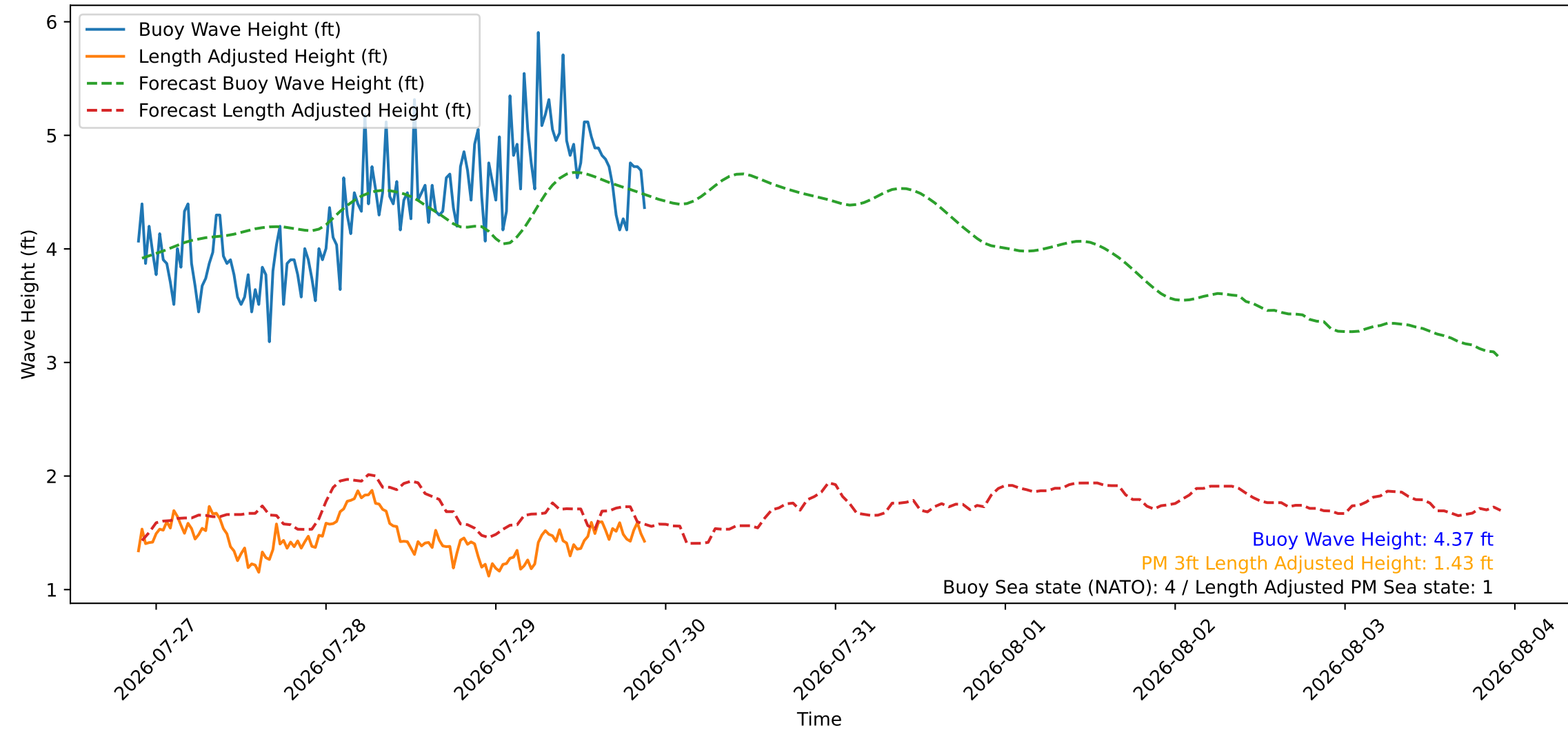
Wave Heights over Time for Oceanside Harbor at 2026-07-29 21:40:26
