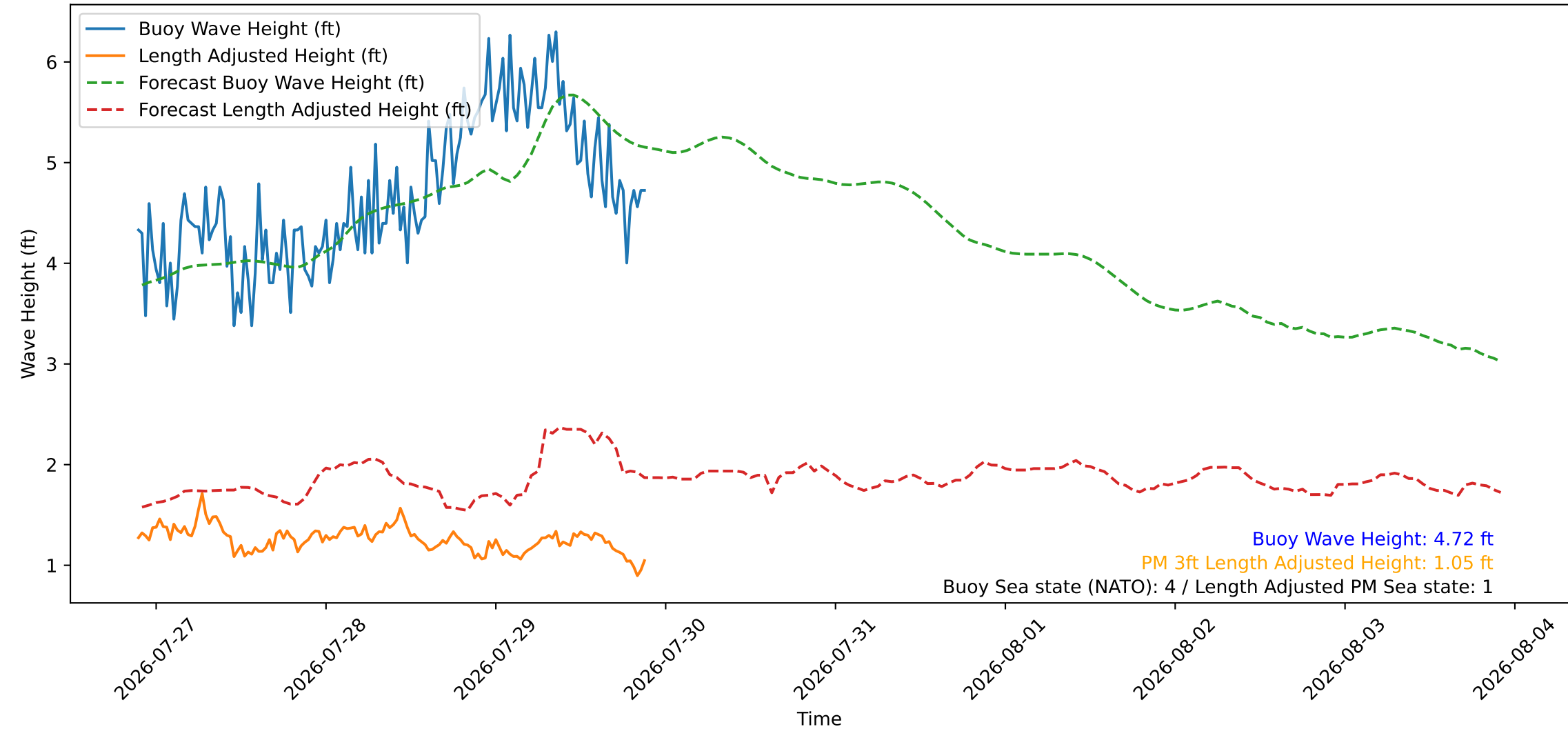
Wave Heights over Time for Green Beach at 2026-07-29 21:41:09
