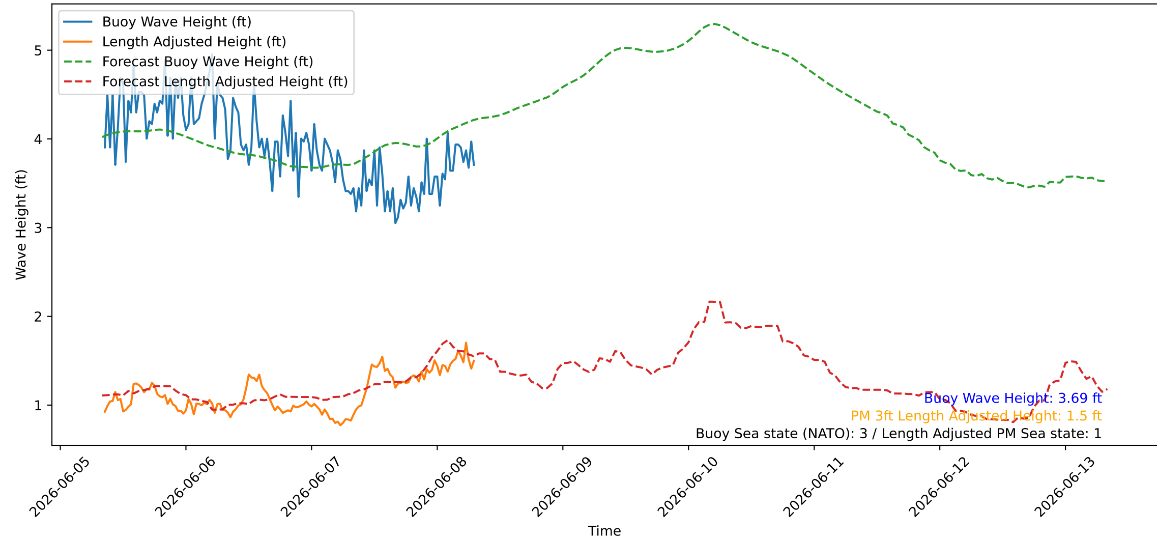
Wave Heights over Time for Red Beach at 2026-06-08 08:00:45
