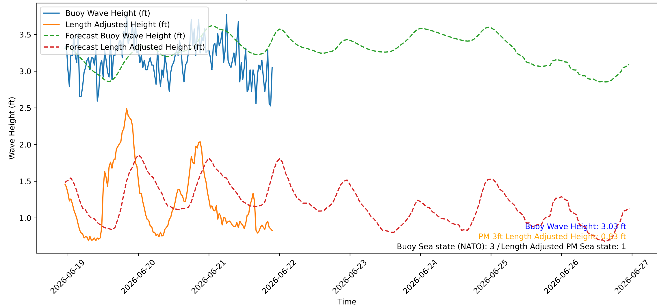
Wave Heights over Time for Red Beach at 2026-06-21 22:30:46
