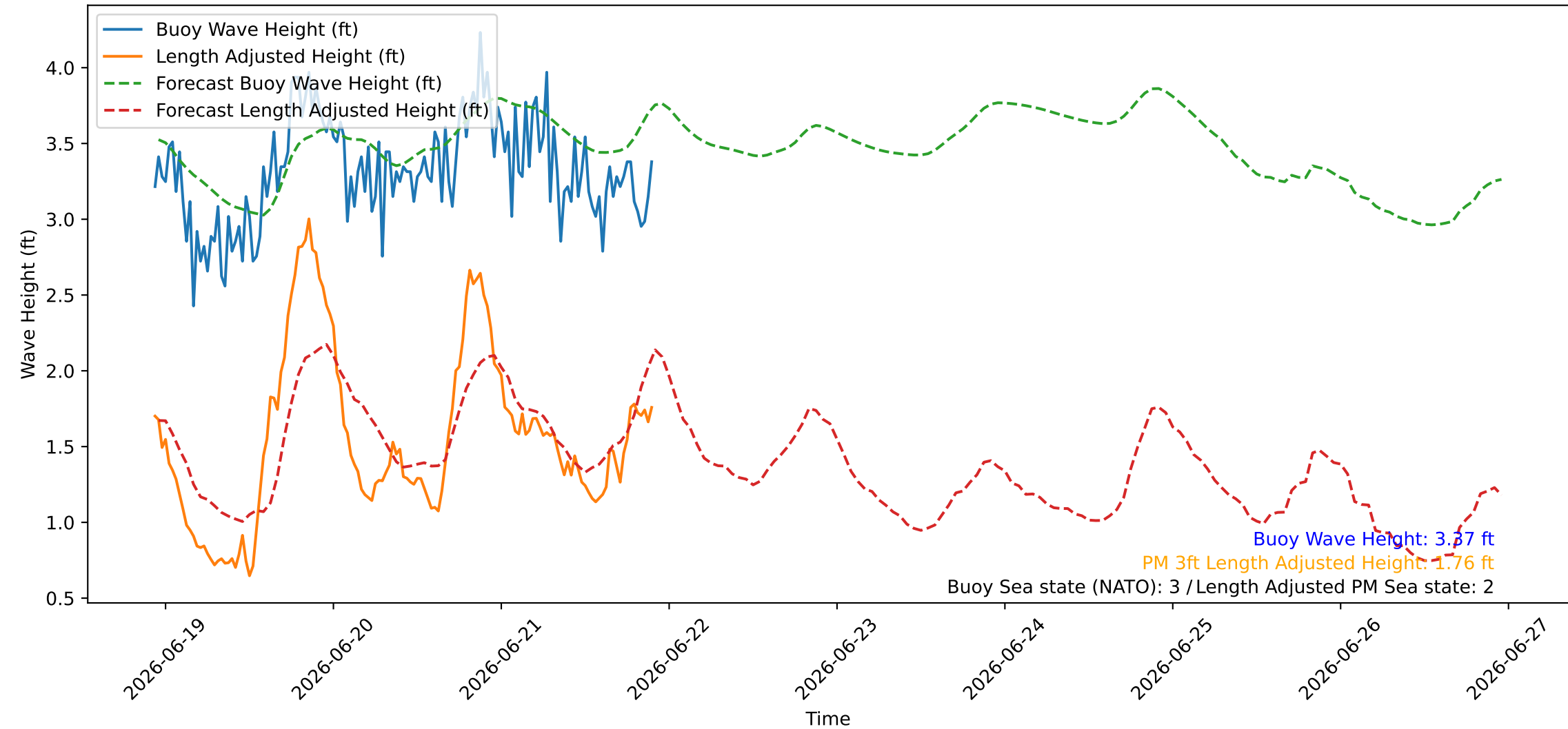
Wave Heights over Time for Green Beach at 2026-06-21 22:31:09
