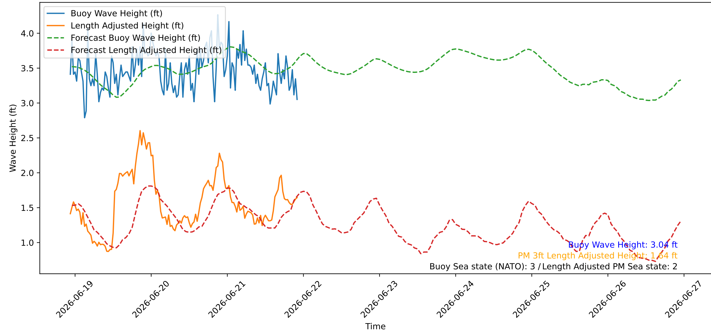
Wave Heights over Time for Oceanside Harbor at 2026-06-21 22:30:27
