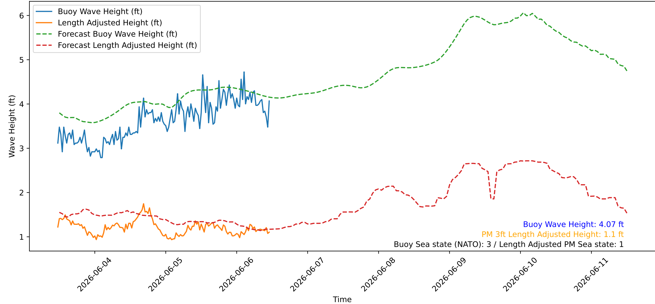
Wave Heights over Time for Green Beach at 2026-06-06 11:41:09
