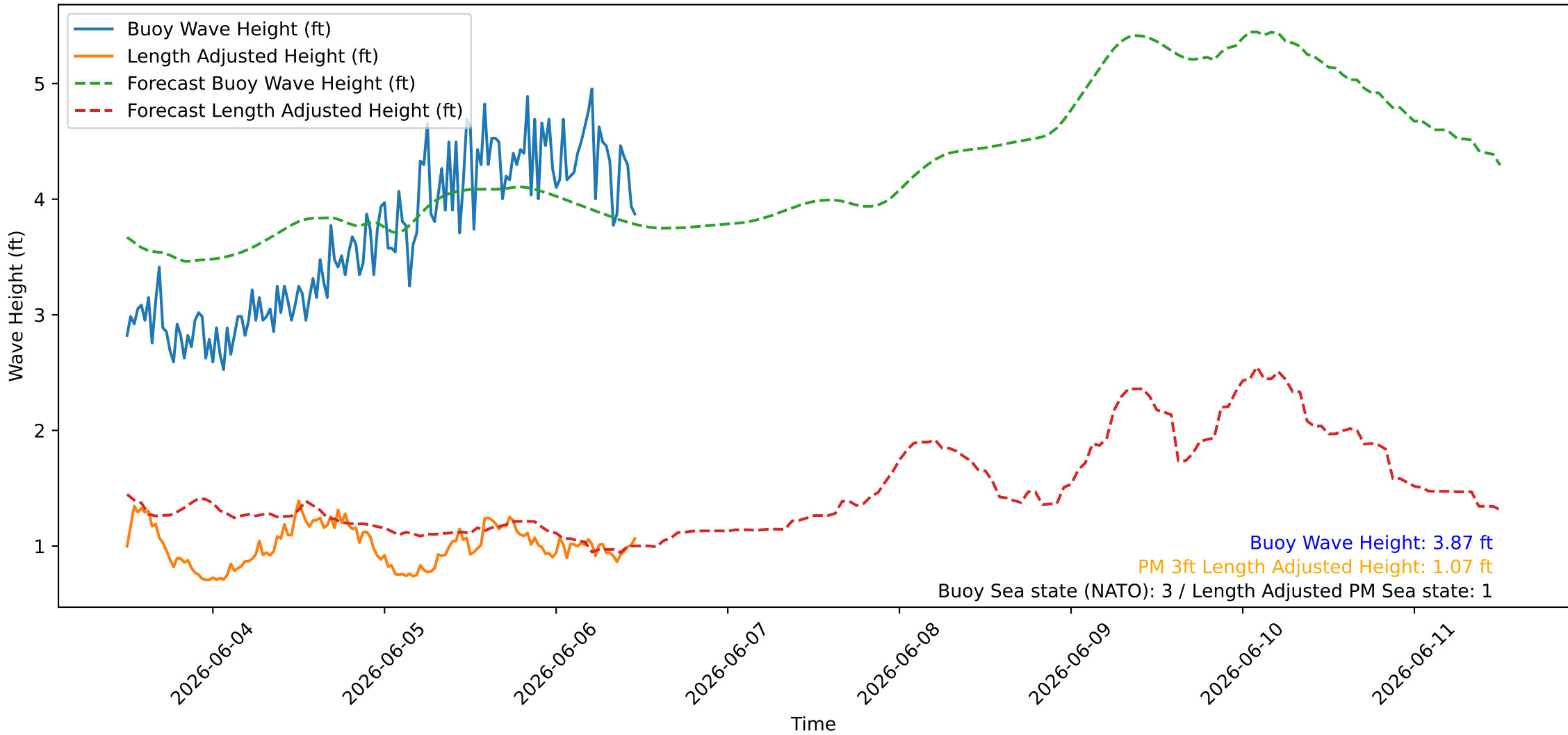
Wave Heights over Time for Red Beach at 2026-06-06 11:40:46
