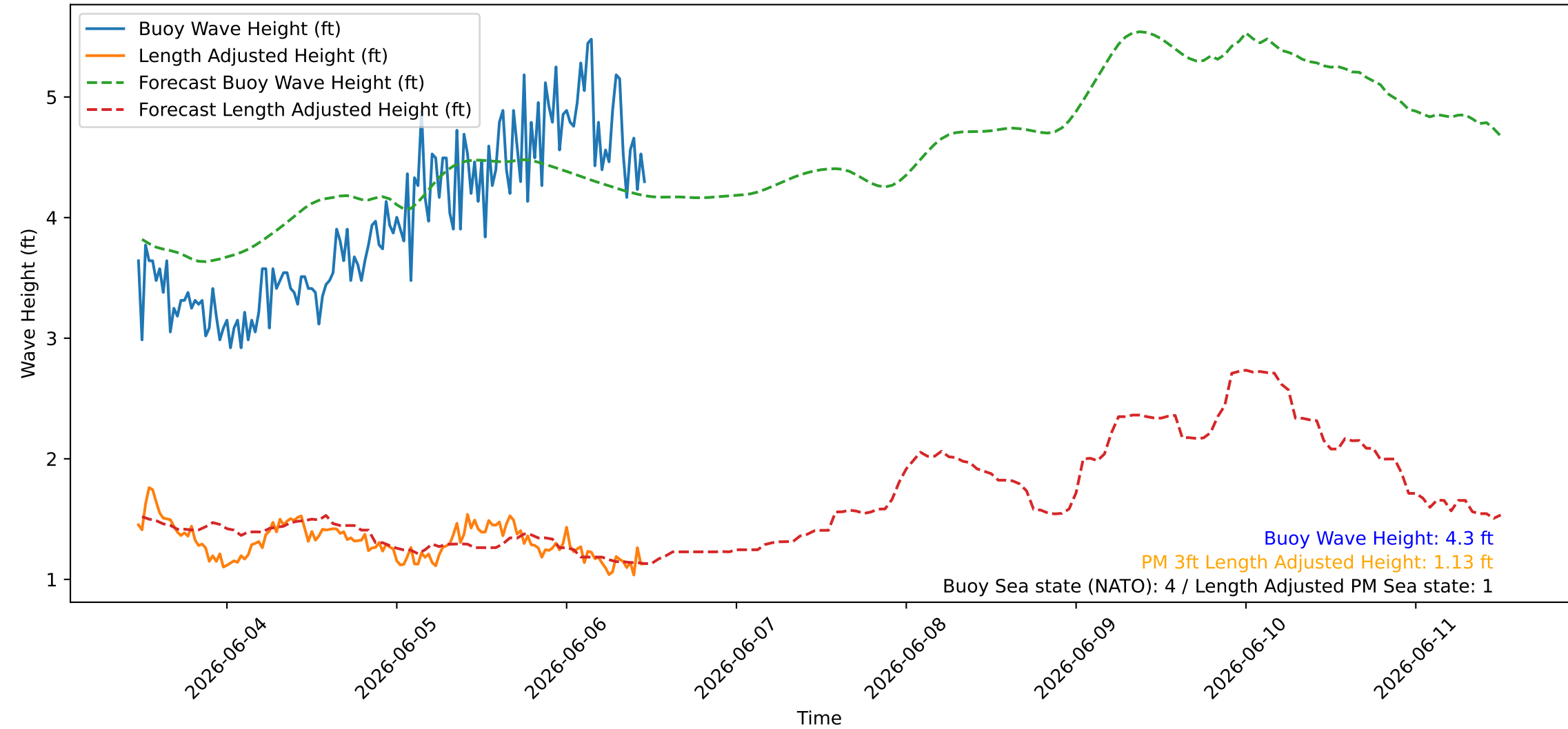
Wave Heights over Time for Oceanside Harbor at 2026-06-06 11:40:26
