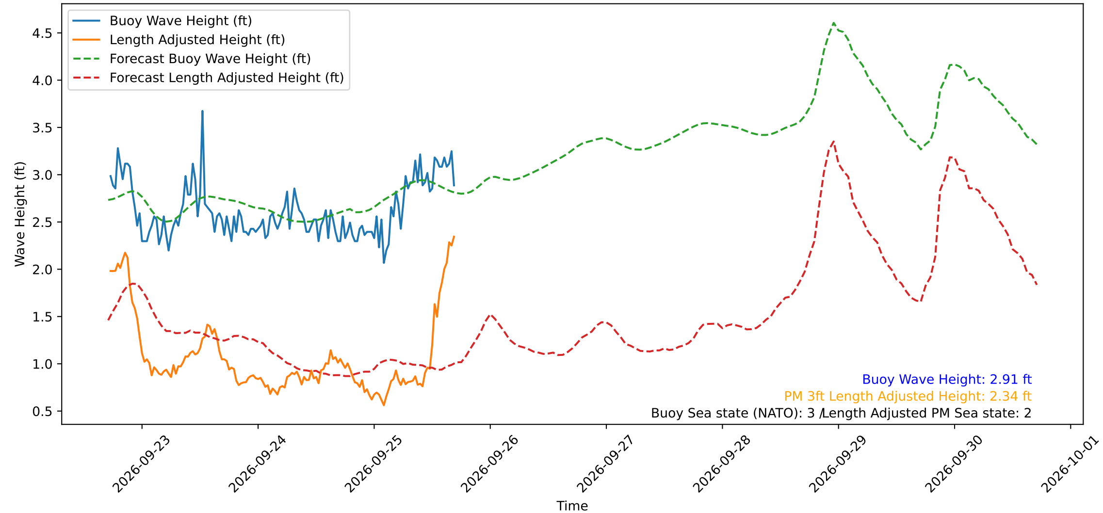
Wave Heights over Time for Red Beach at 2026-09-25 17:10:49
