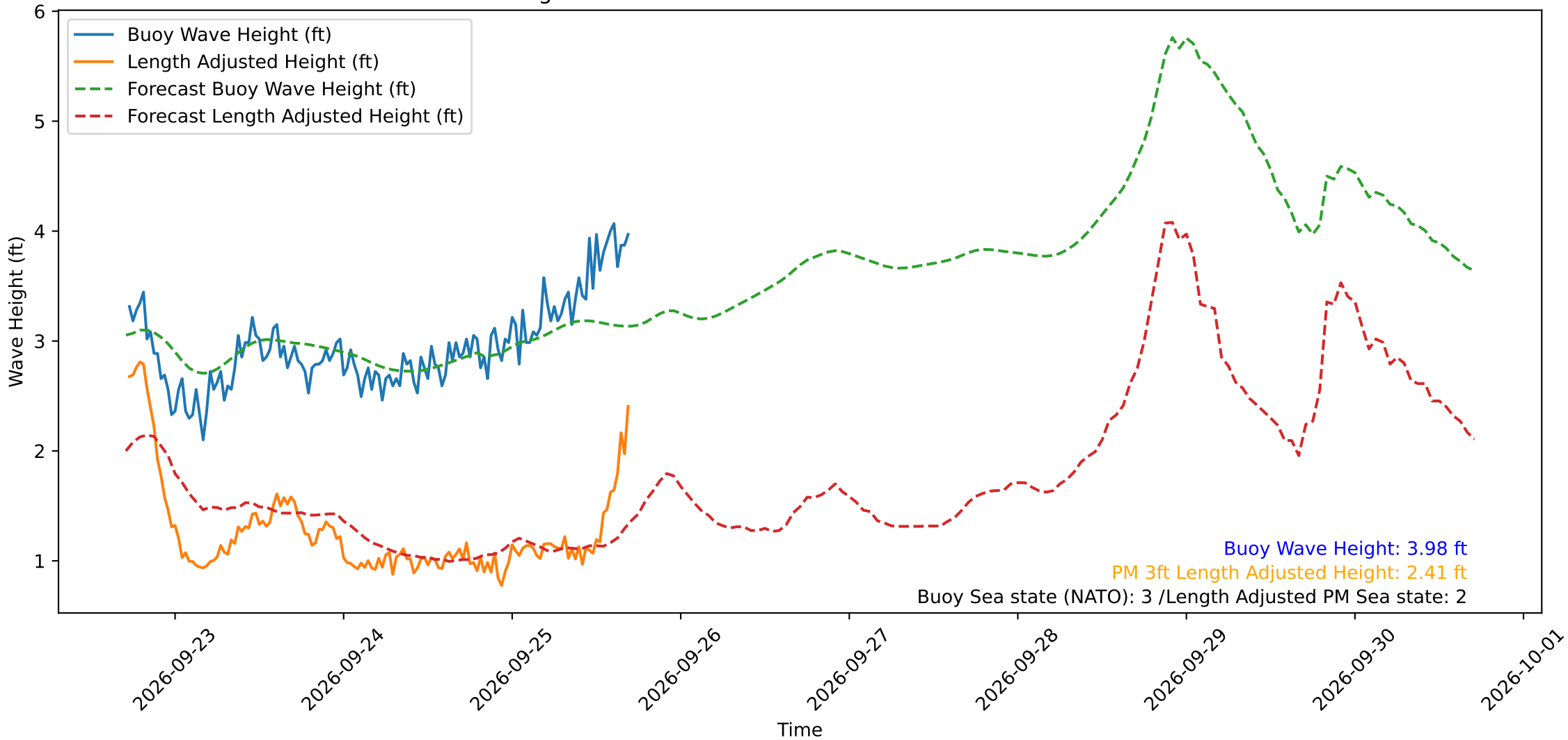
Wave Heights over Time for Green Beach at 2026-09-25 17:11:11
