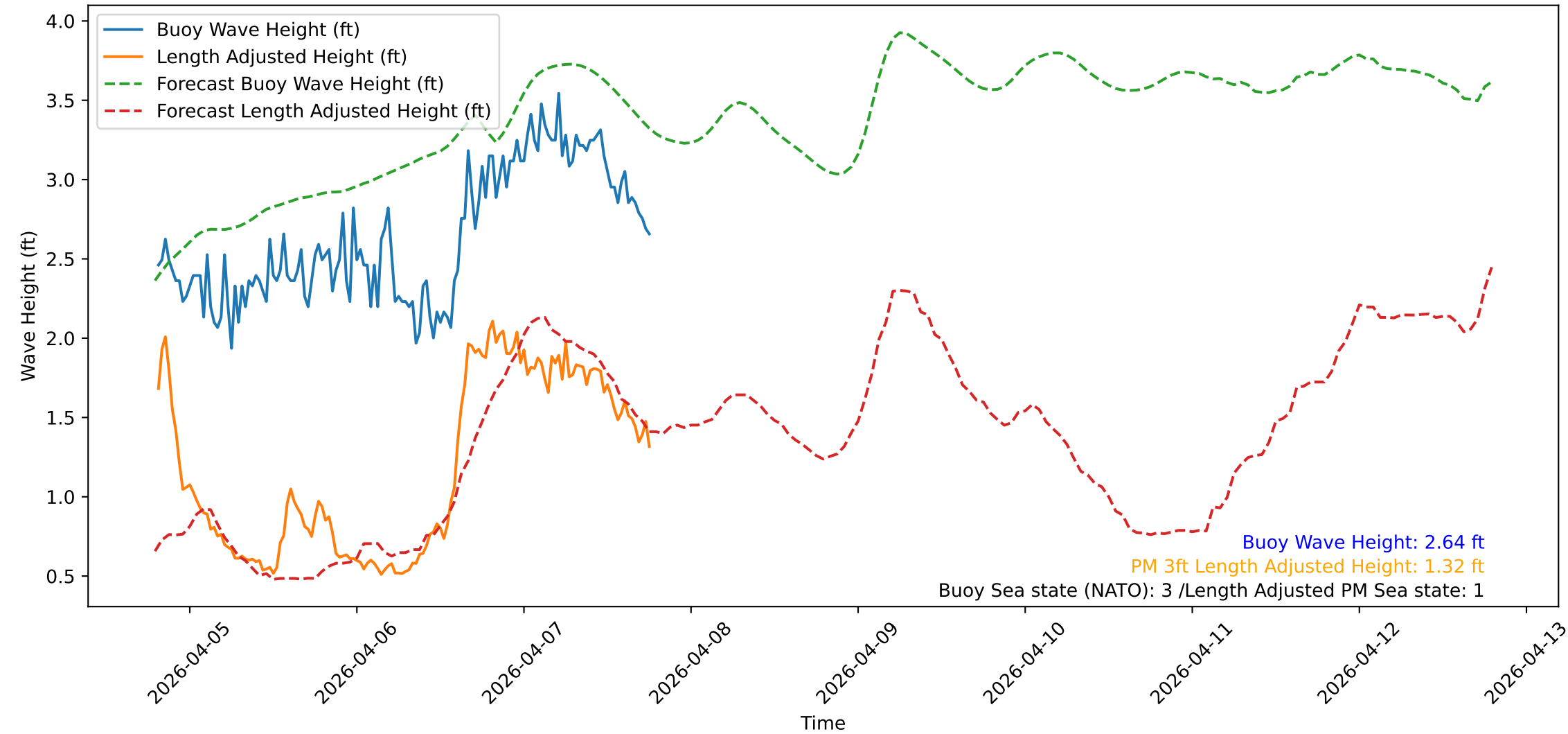
Wave Heights over Time for Red Beach at 2026-04-07 19:00:48
