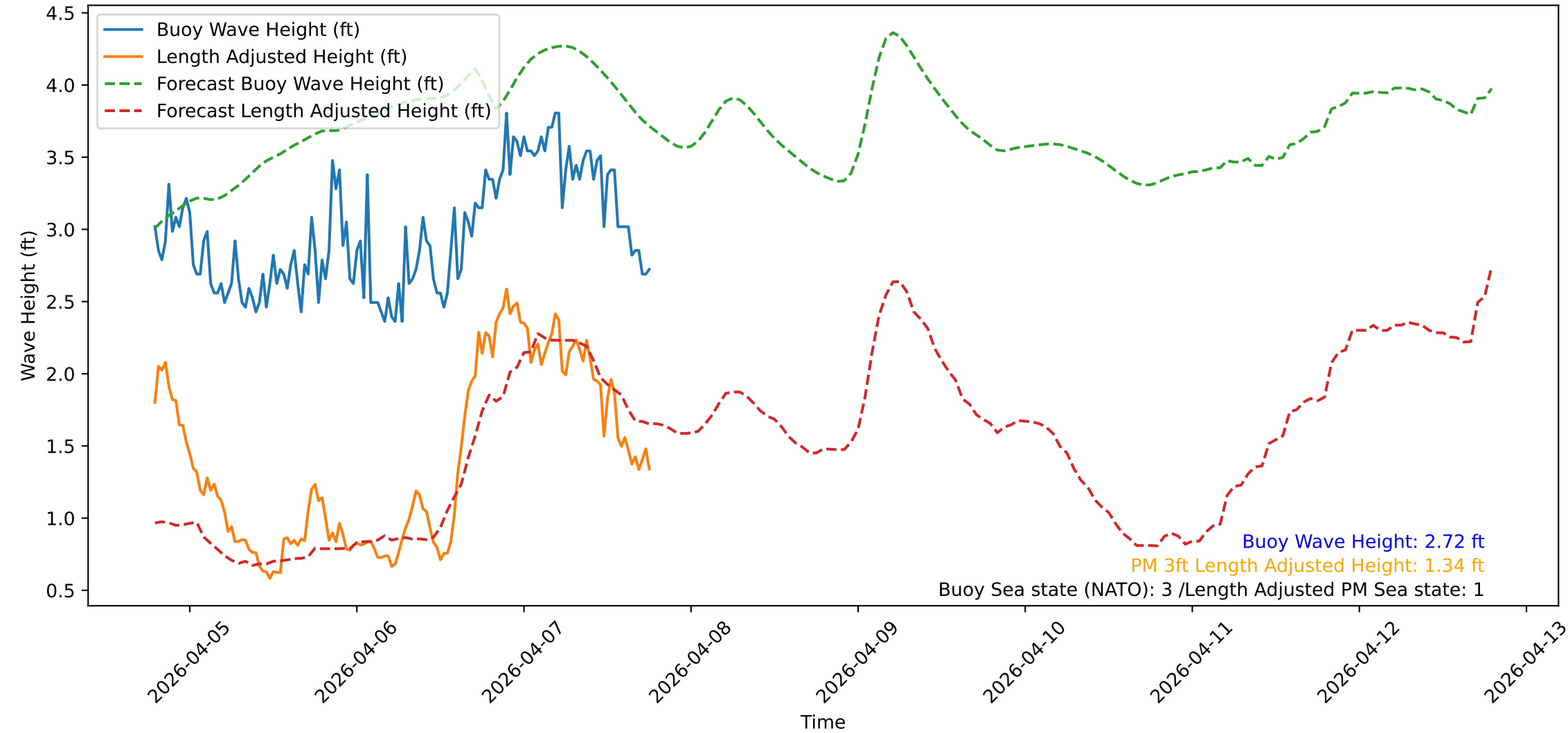
Wave Heights over Time for Green Beach at 2026-04-07 19:01:10
