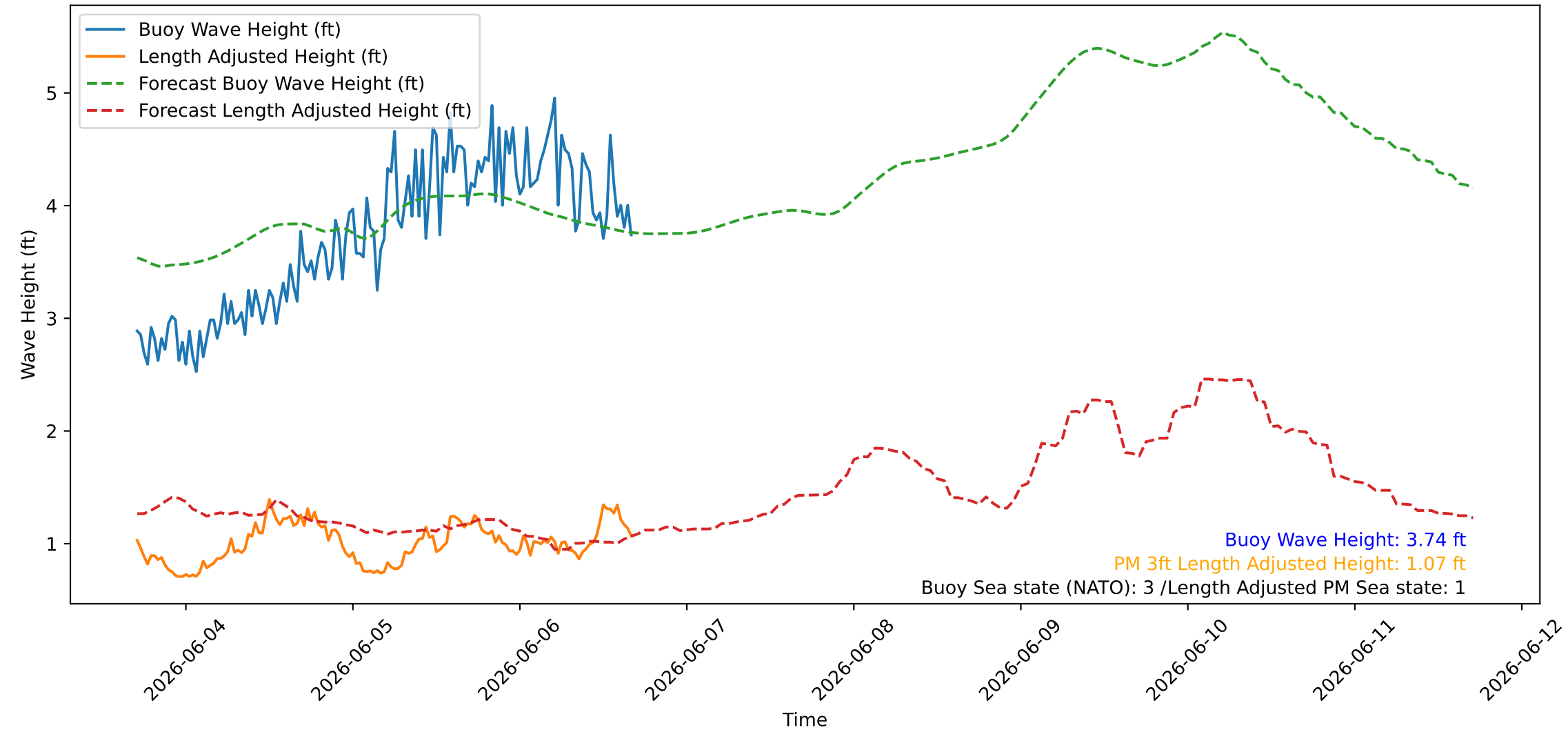
Wave Heights over Time for Red Beach at 2026-06-06 16:50:46
