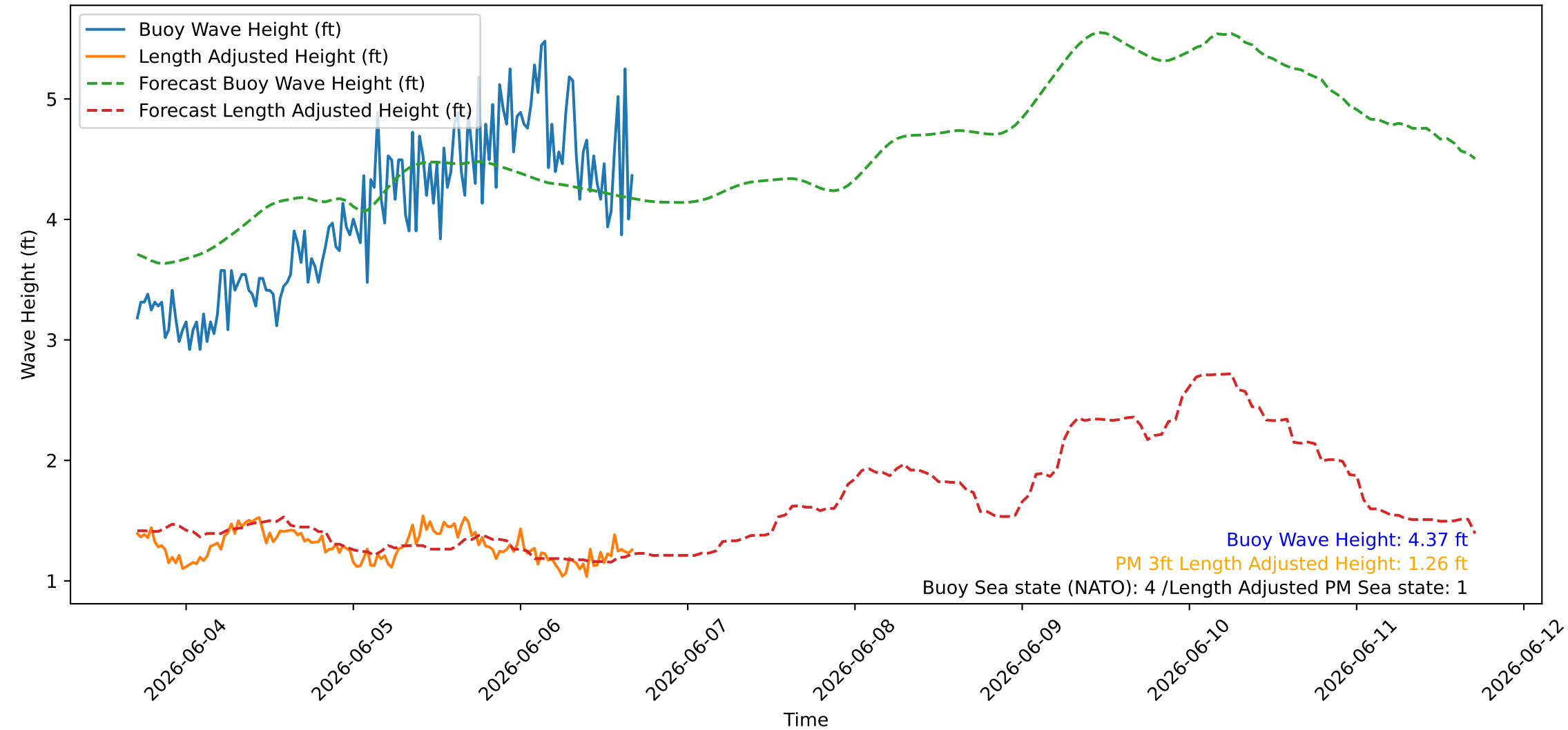
Wave Heights over Time for Oceanside Harbor at 2026-06-06 16:50:25
