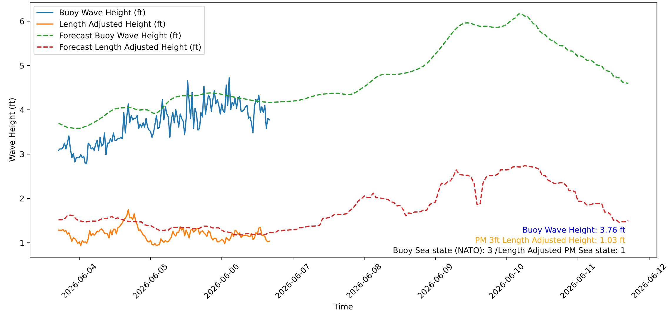
Wave Heights over Time for Green Beach at 2026-06-06 16:51:09
