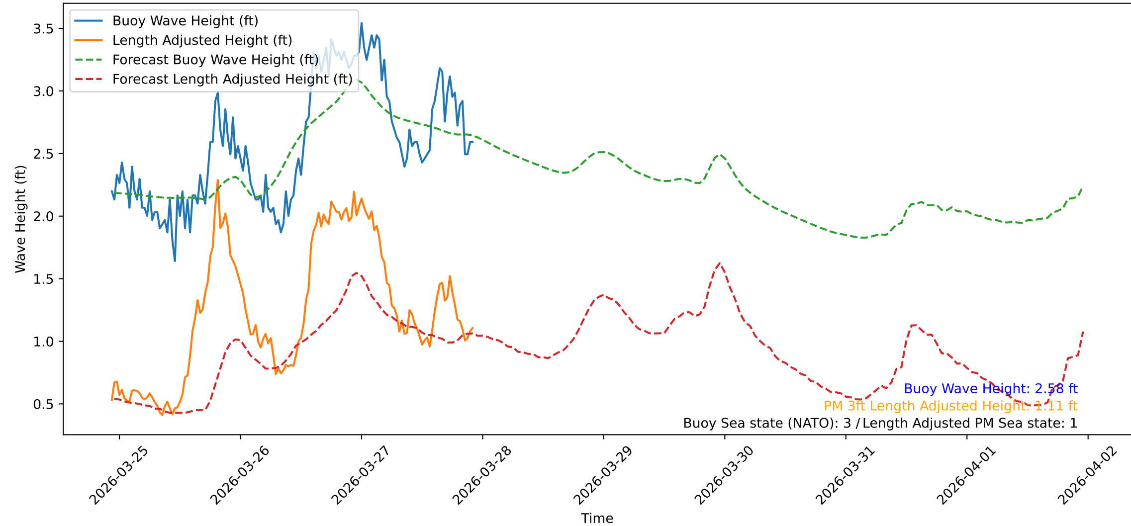
Wave Heights over Time for Green Beach at 2026-03-27 22:41:09
