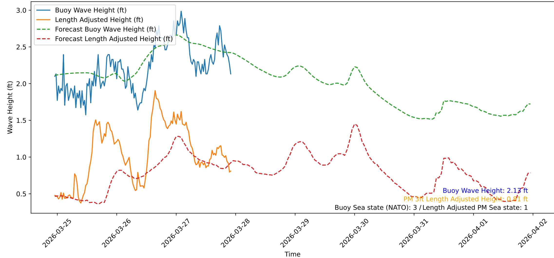
Wave Heights over Time for Red Beach at 2026-03-27 22:40:47
