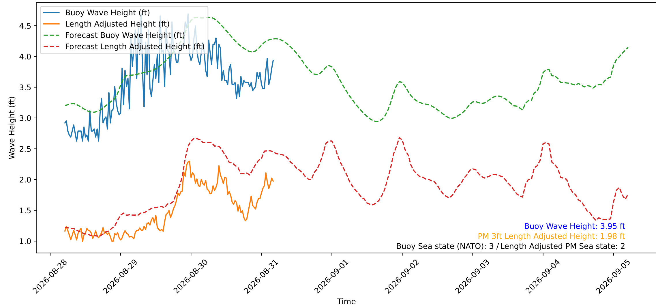
Wave Heights over Time for Red Beach at 2026-08-31 04:50:51
