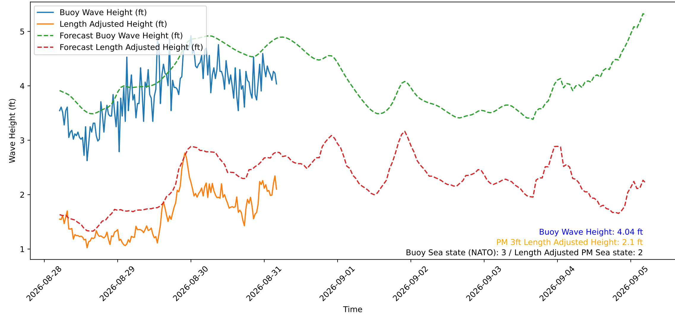
Wave Heights over Time for Green Beach at 2026-08-31 04:51:15
