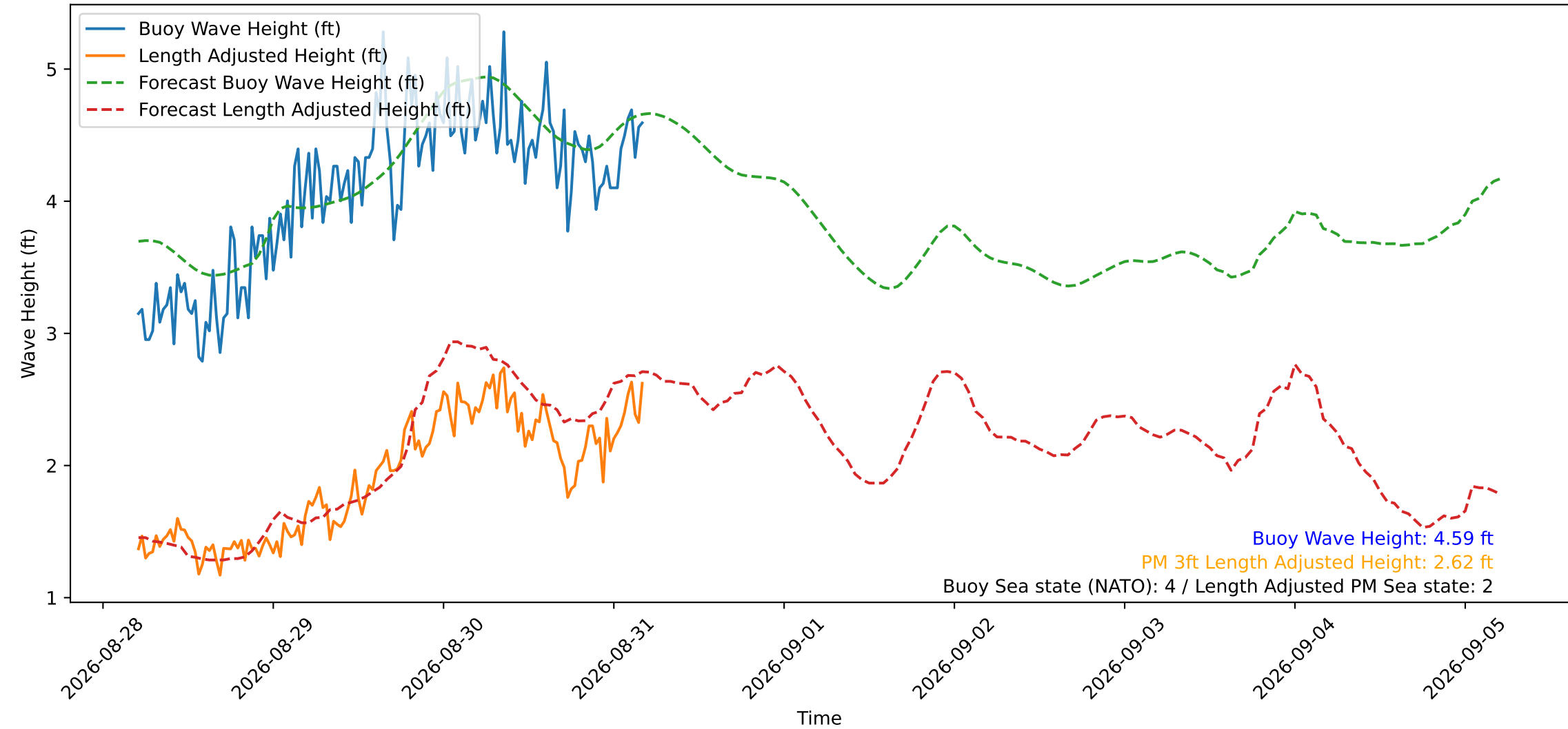
Wave Heights over Time for Oceanside Harbor at 2026-08-31 04:50:30
