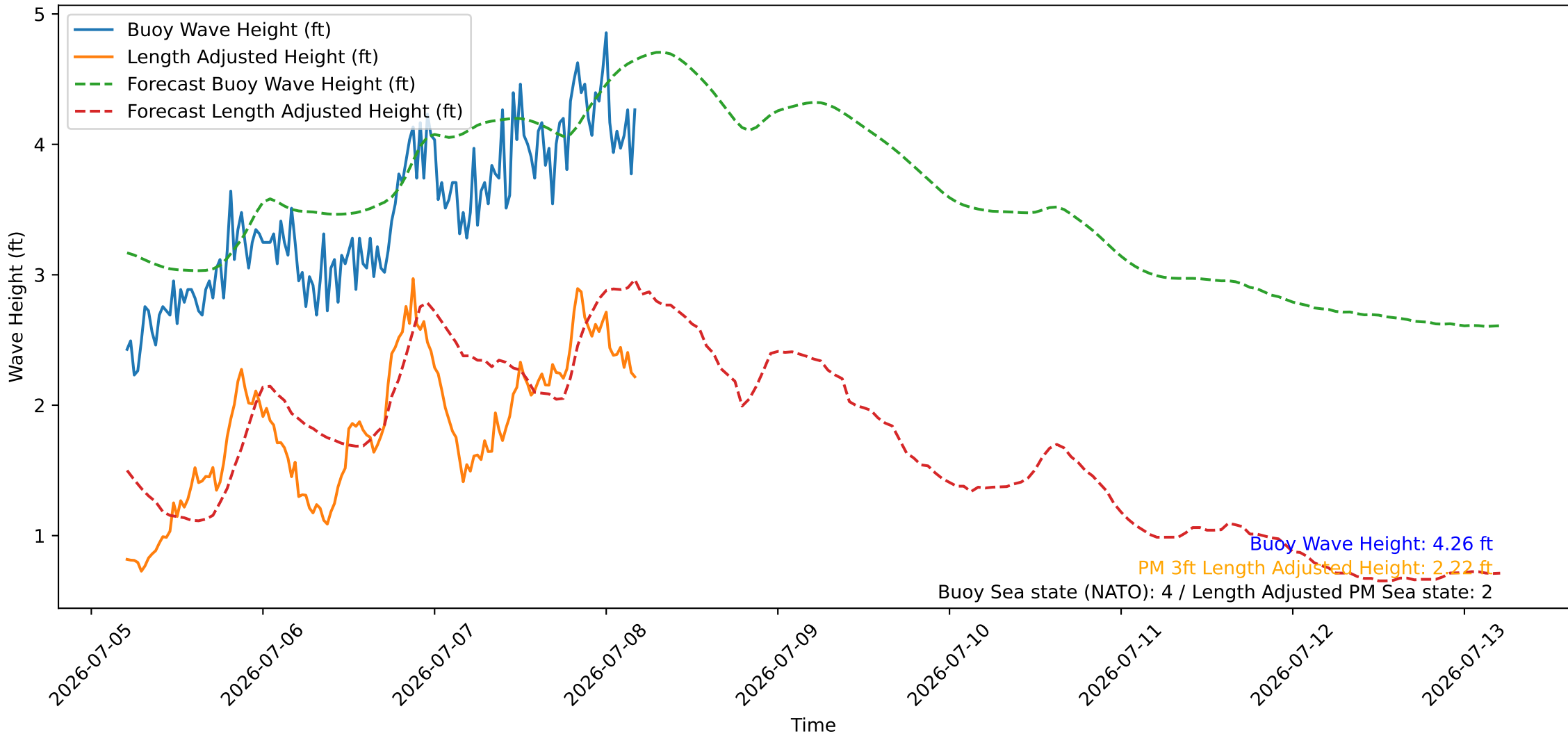
Wave Heights over Time for Red Beach at 2026-07-08 04:50:48
