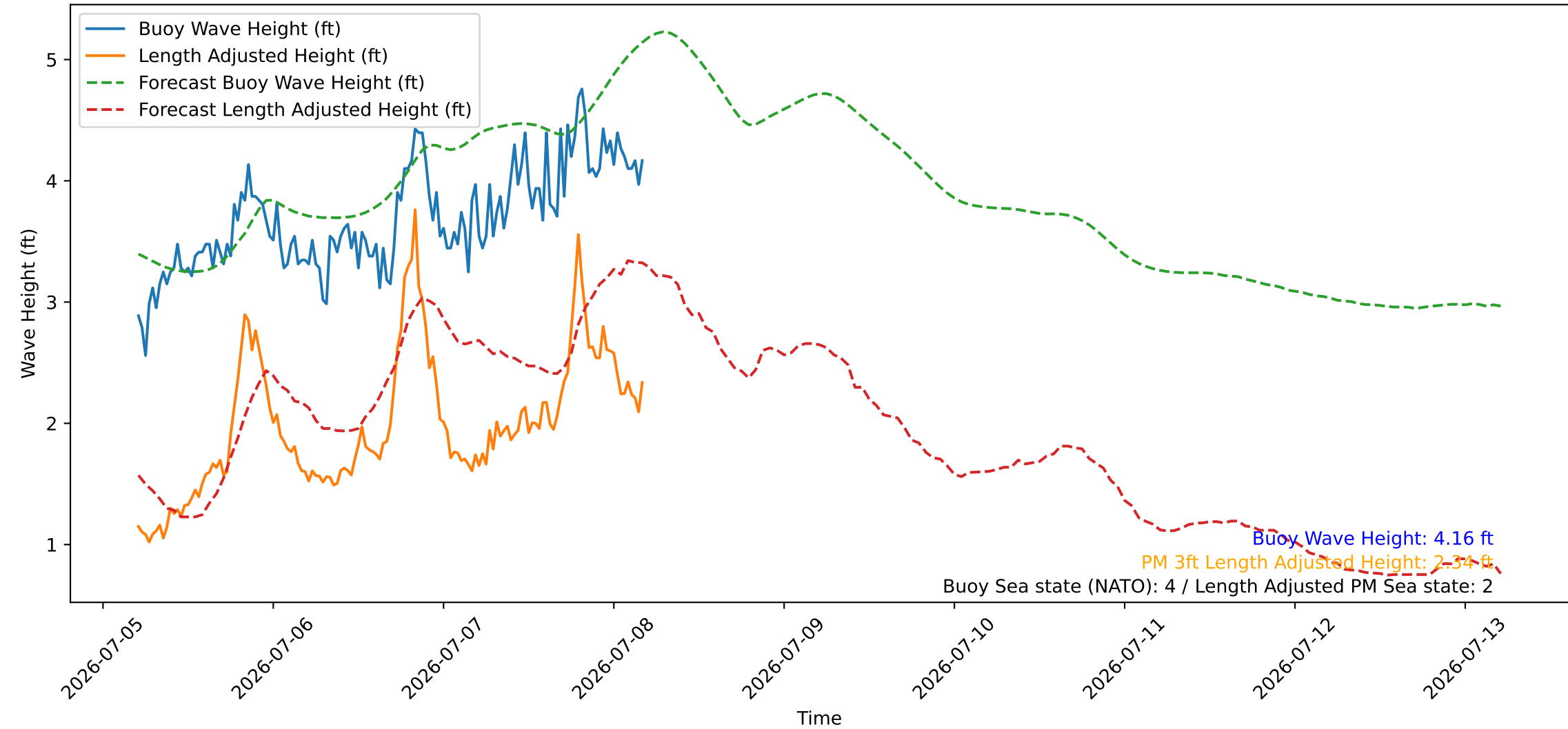
Wave Heights over Time for Green Beach at 2026-07-08 04:51:10
