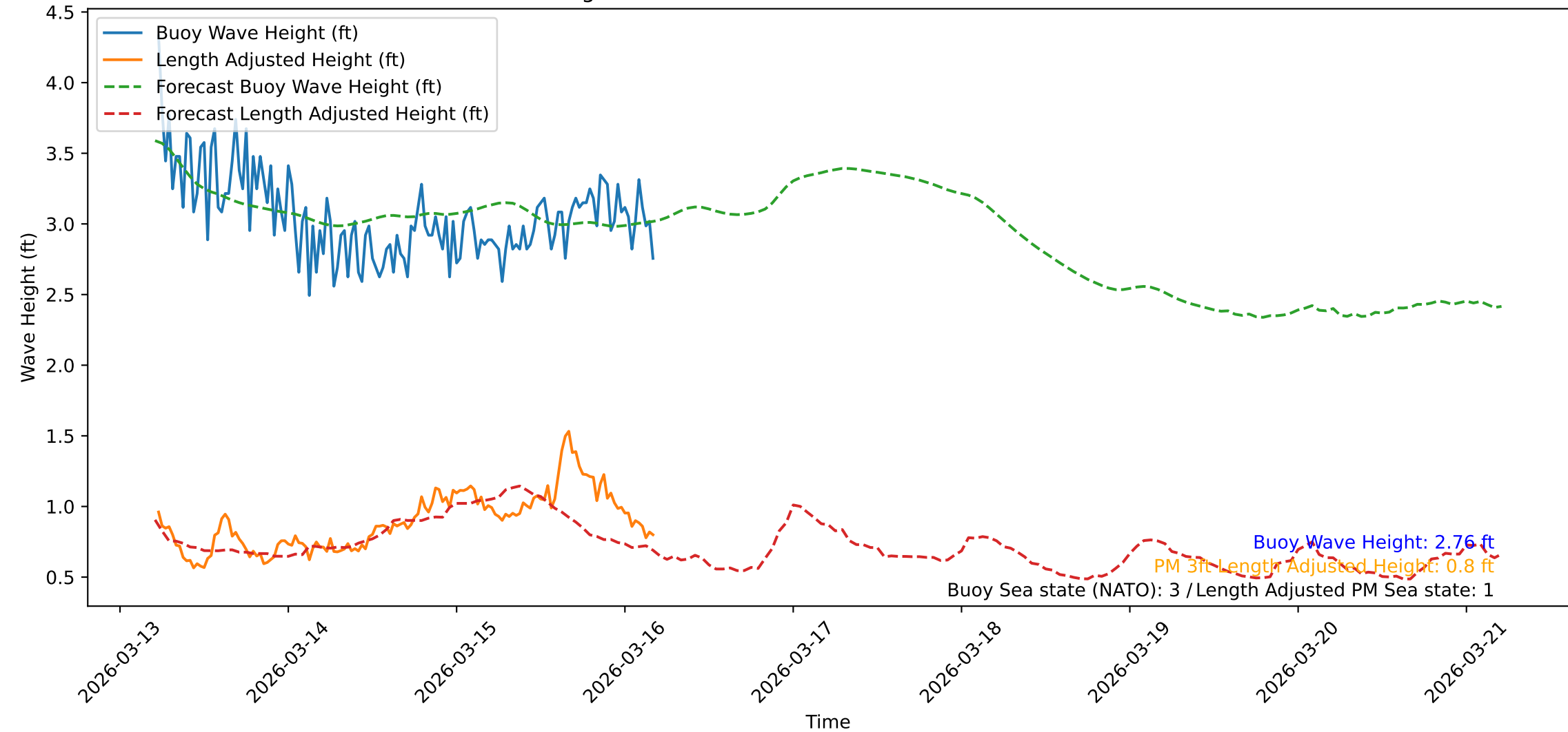
Wave Heights over Time for Red Beach at 2026-03-16 05:01:13
