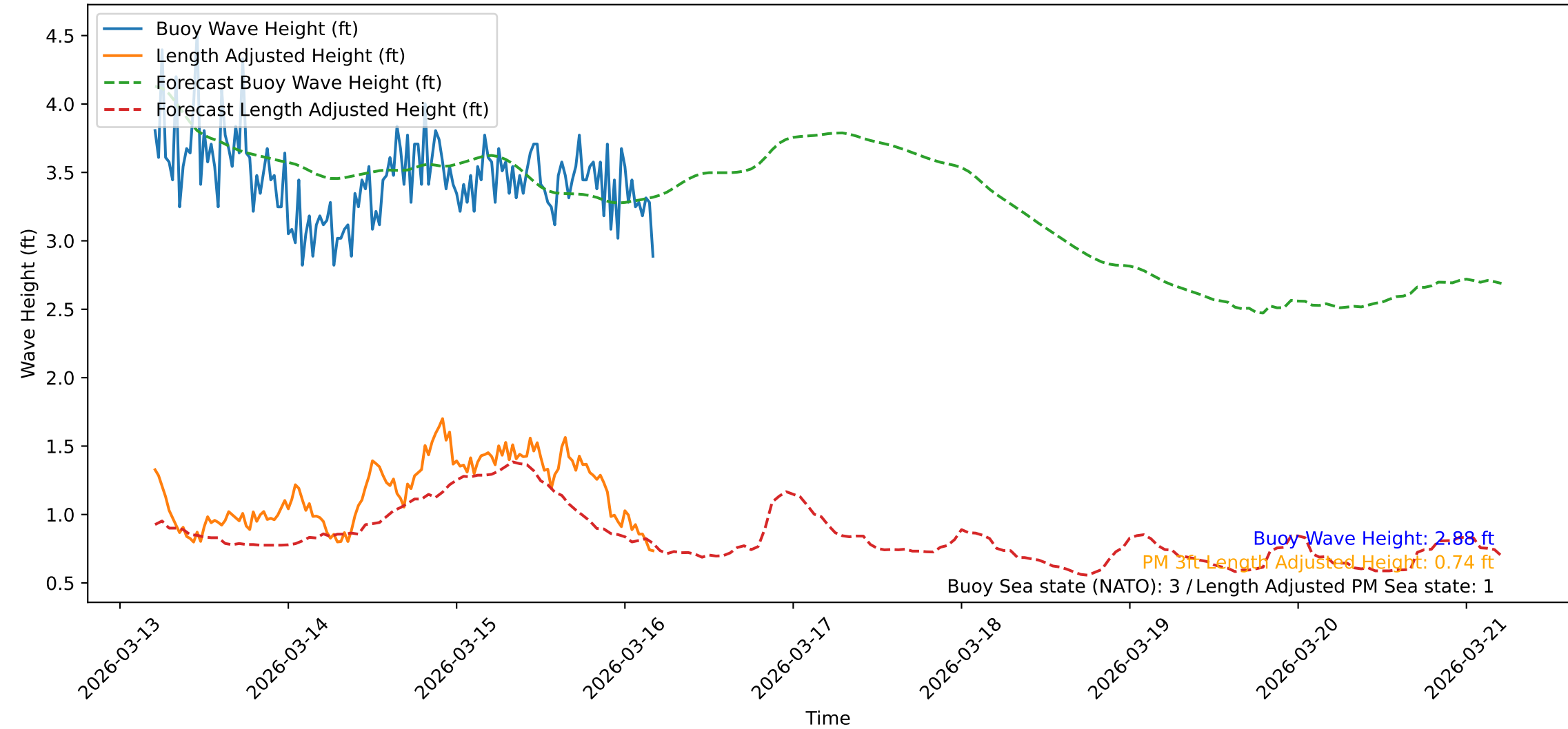
Wave Heights over Time for Green Beach at 2026-03-16 05:01:48
