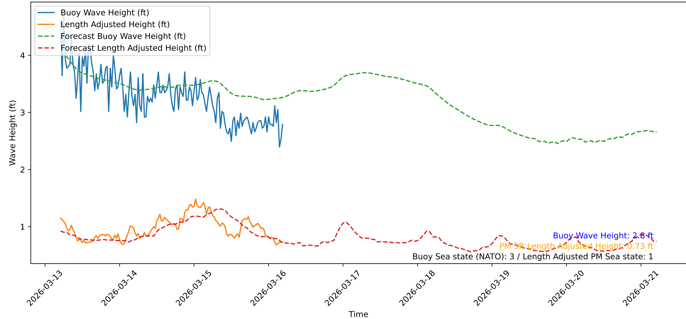
Wave Heights over Time for Oceanside Harbor at 2026-03-16 05:00:46
