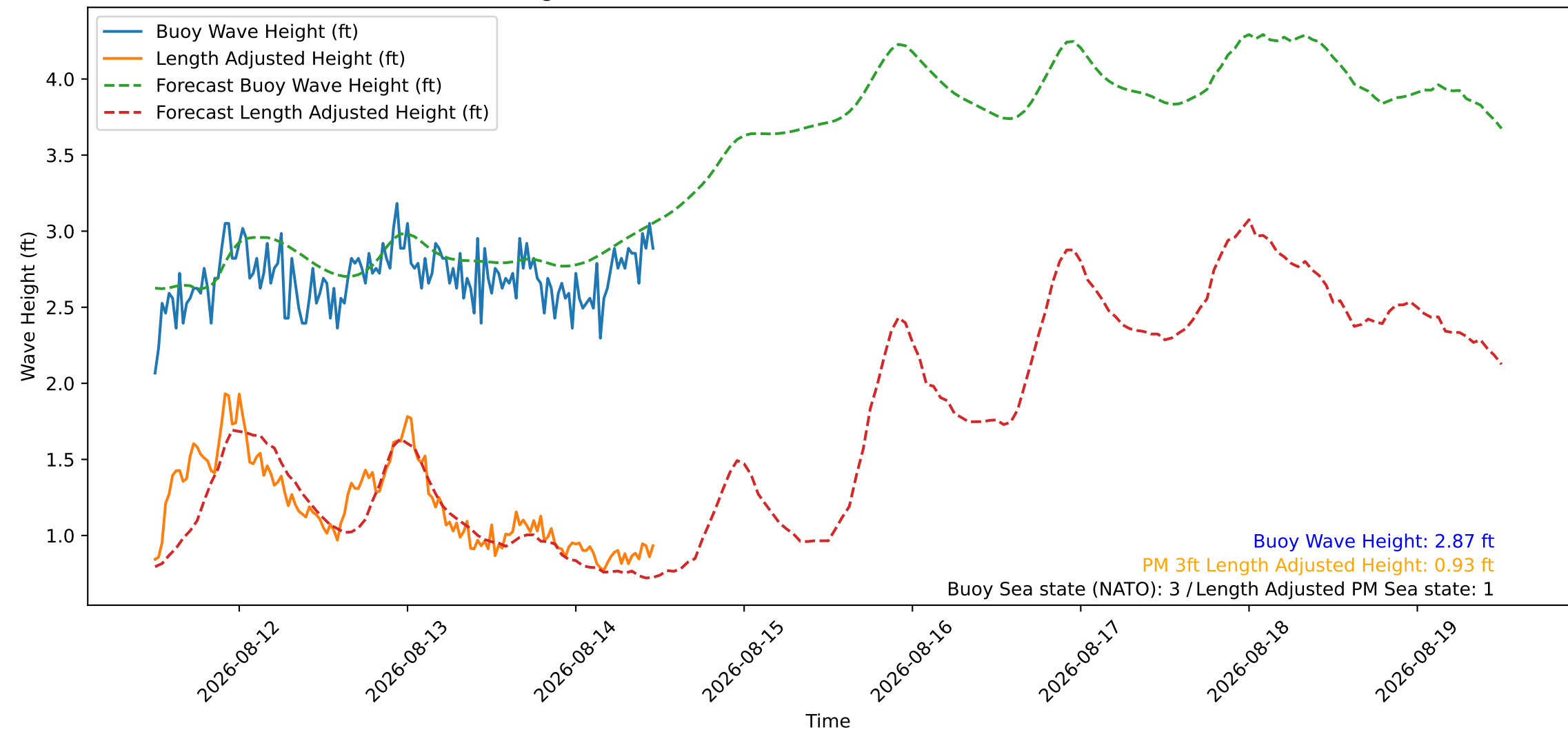
Wave Heights over Time for Oceanside Harbor at 2026-08-14 11:50:27
