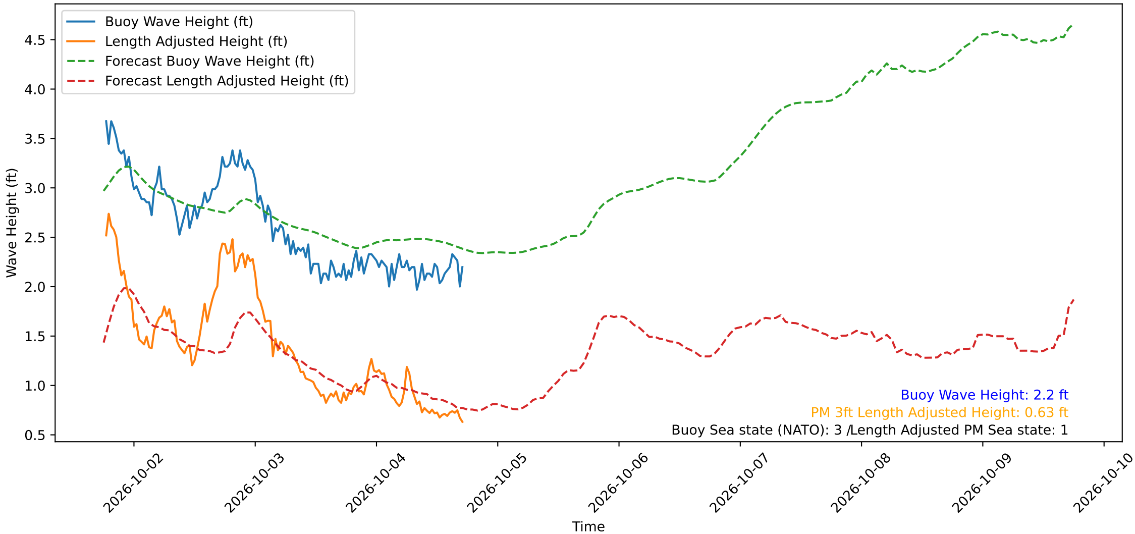
Wave Heights over Time for Green Beach at 2026-10-04 18:01:12
