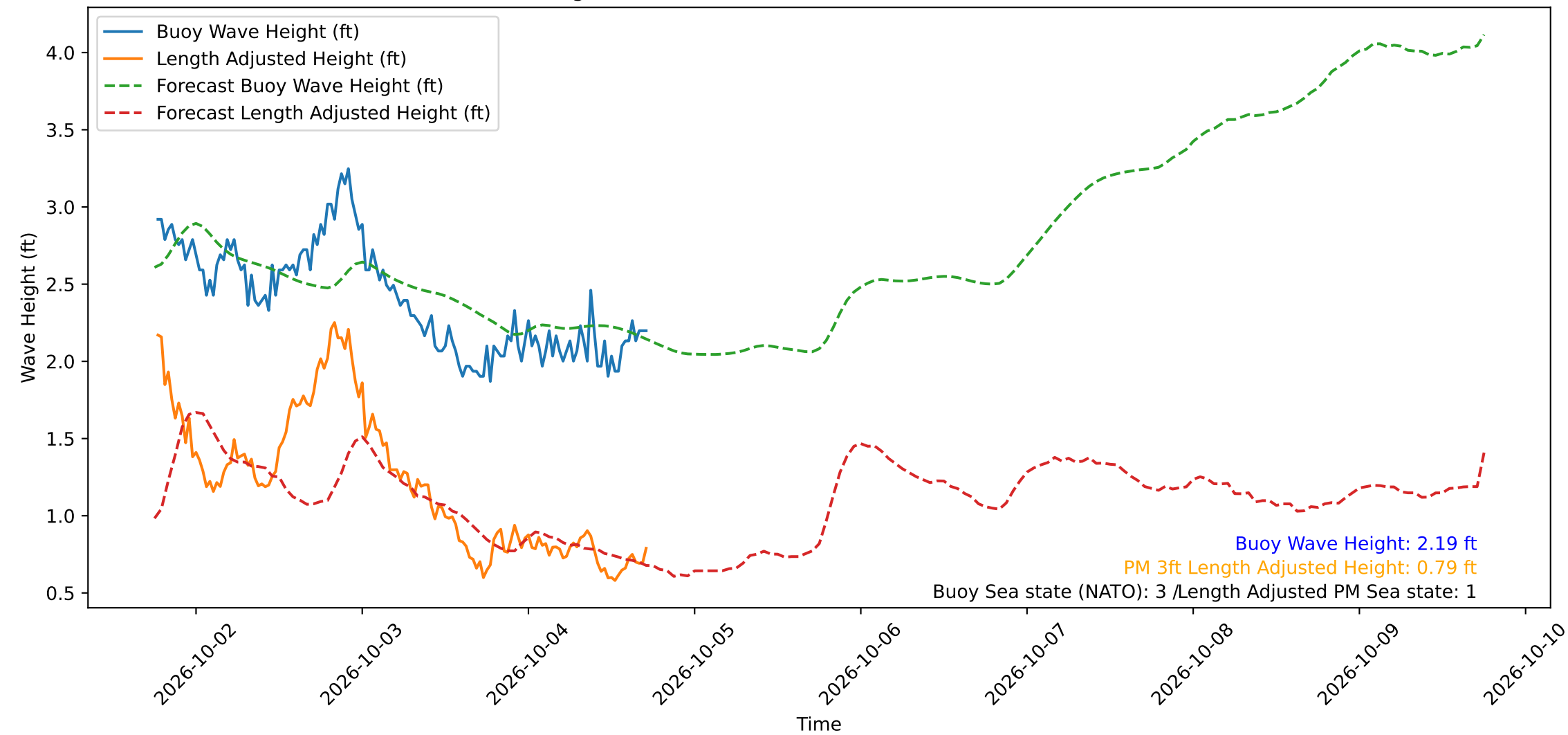
Wave Heights over Time for Red Beach at 2026-10-04 18:00:49
