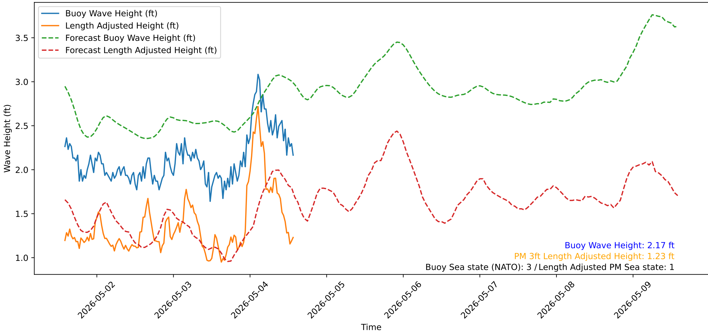
Wave Heights over Time for Oceanside Harbor at 2026-05-04 14:10:32
