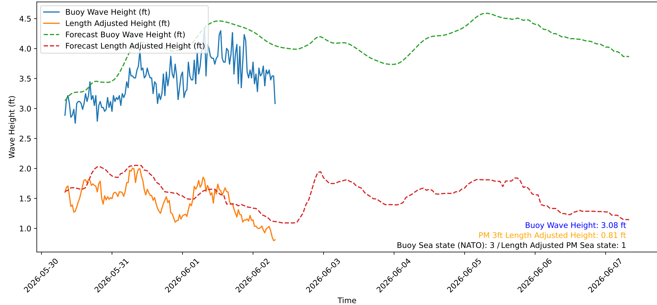
Wave Heights over Time for Green Beach at 2026-06-02 08:11:09
