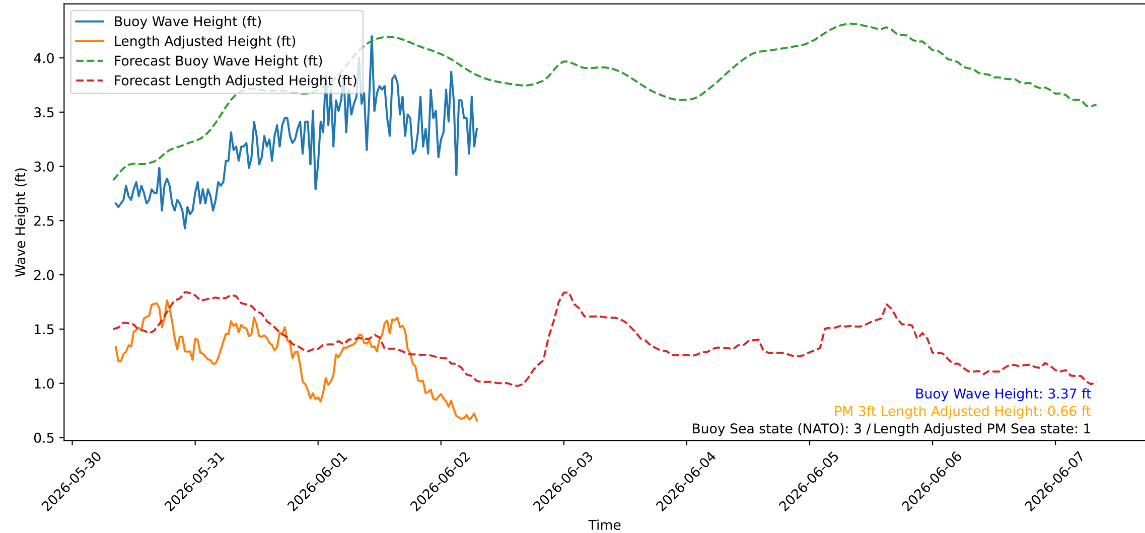
Wave Heights over Time for Red Beach at 2026-06-02 08:10:46
