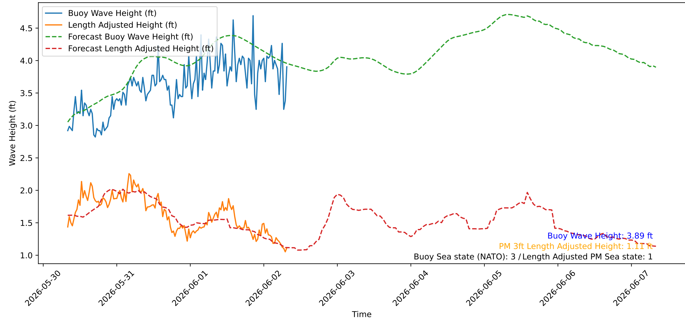
Wave Heights over Time for Oceanside Harbor at 2026-06-02 08:10:27
