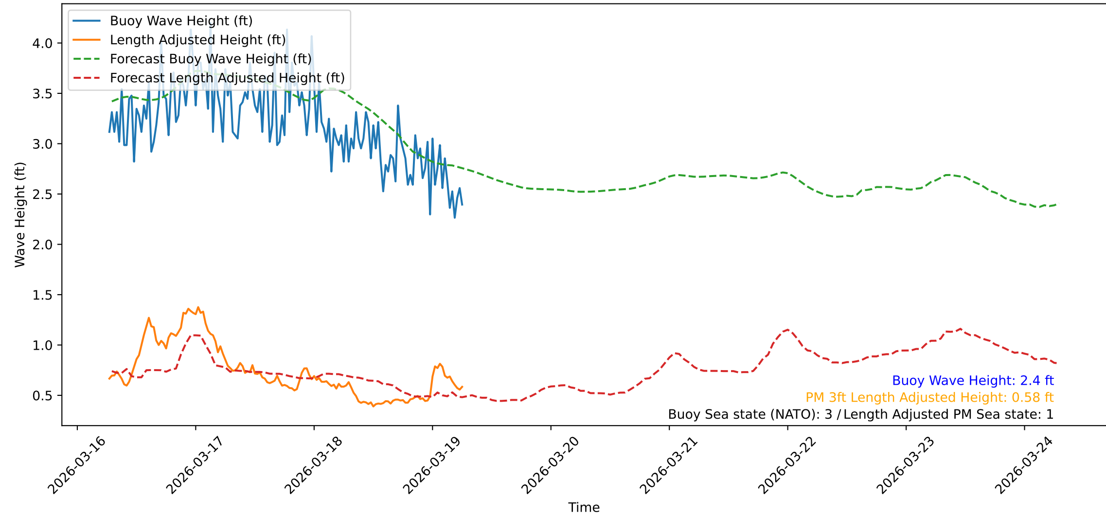
Wave Heights over Time for Green Beach at 2026-03-19 06:41:10
