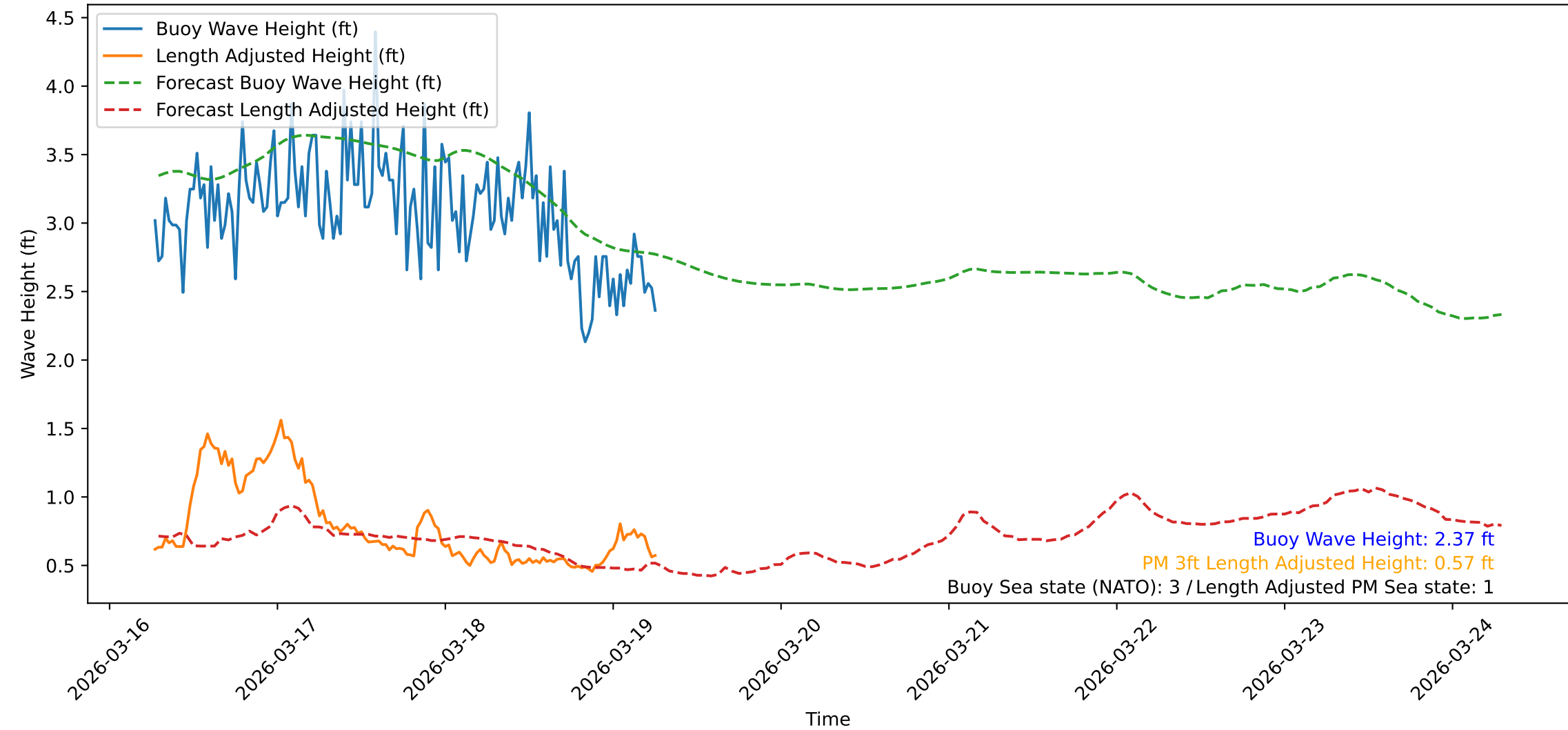
Wave Heights over Time for Oceanside Harbor at 2026-03-19 06:40:31
