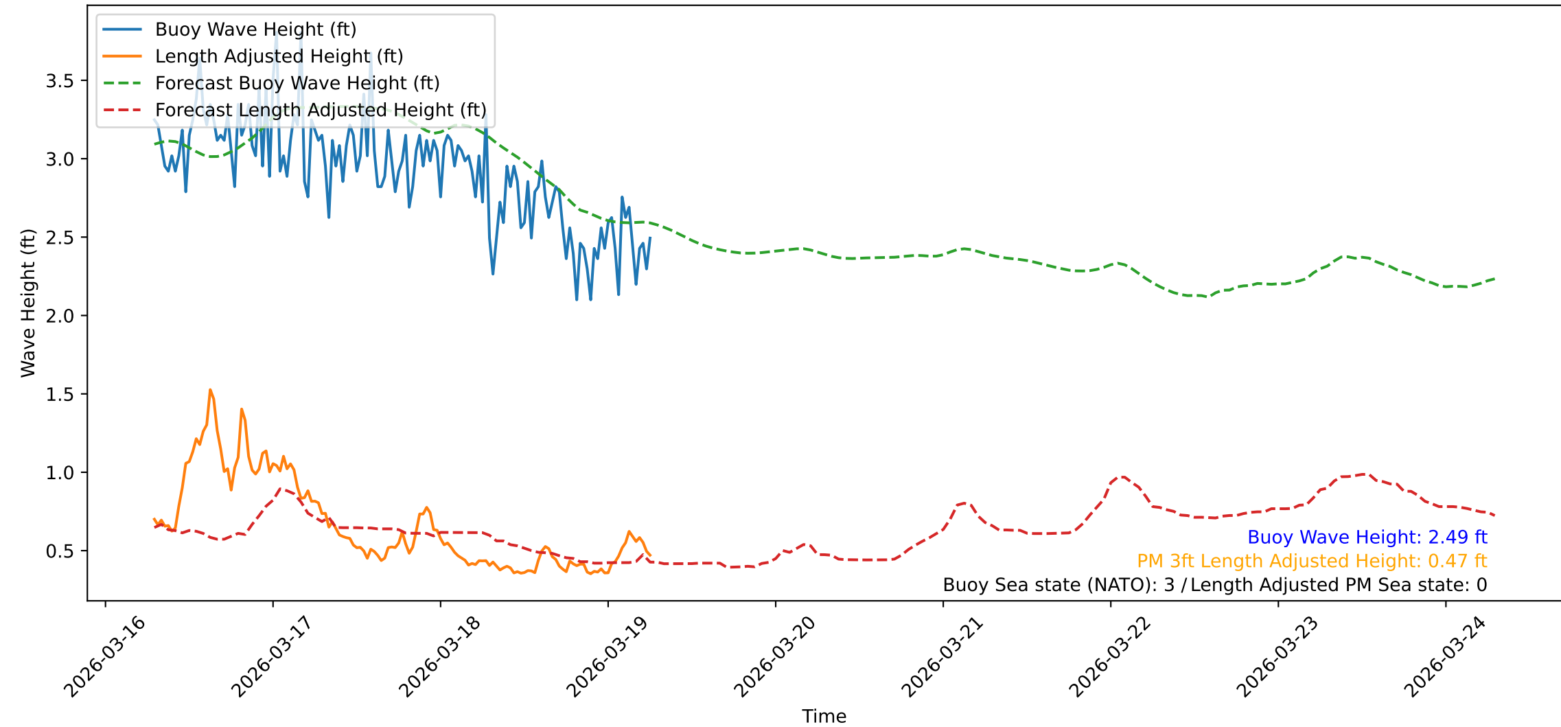
Wave Heights over Time for Red Beach at 2026-03-19 06:40:47
