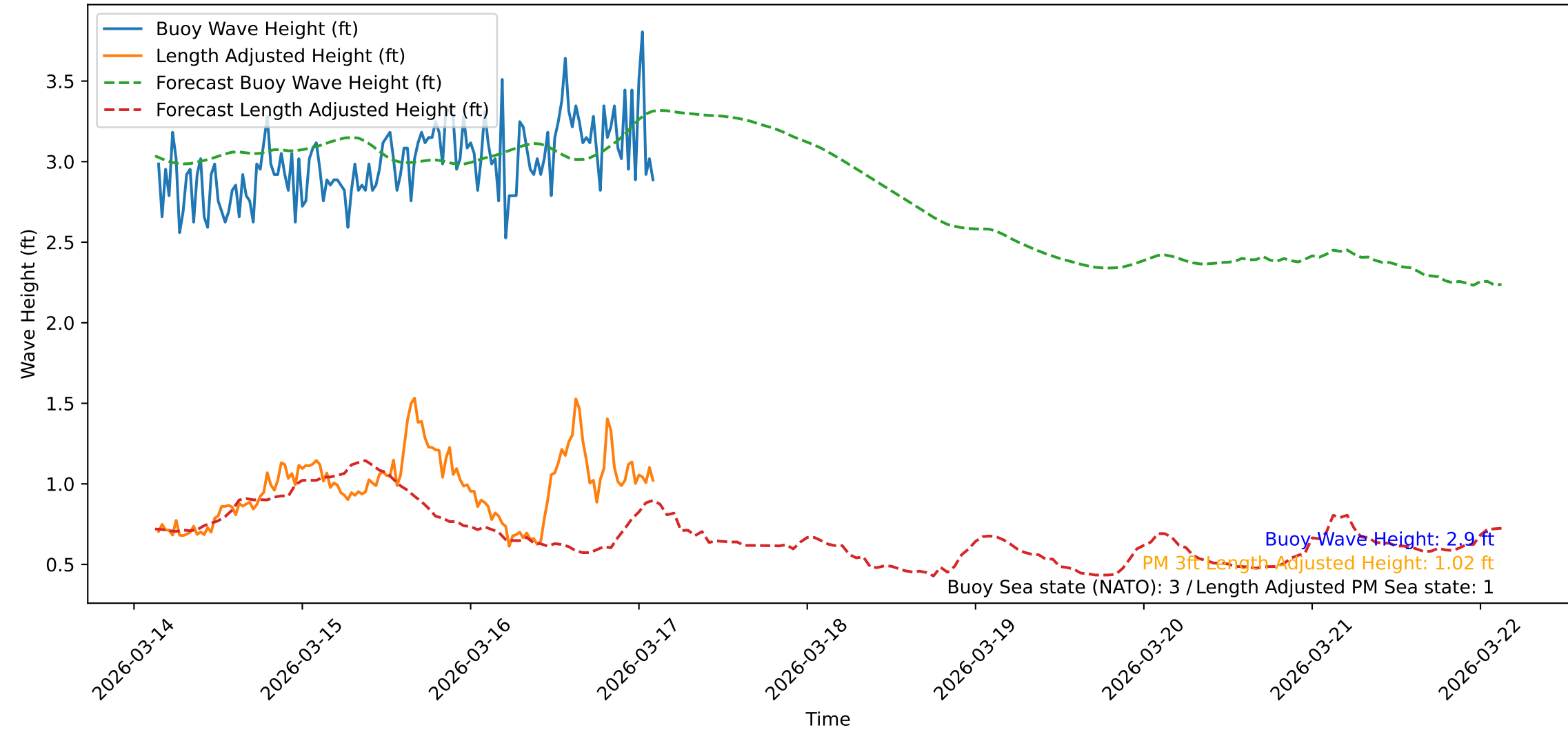
Wave Heights over Time for Red Beach at 2026-03-17 03:11:07
