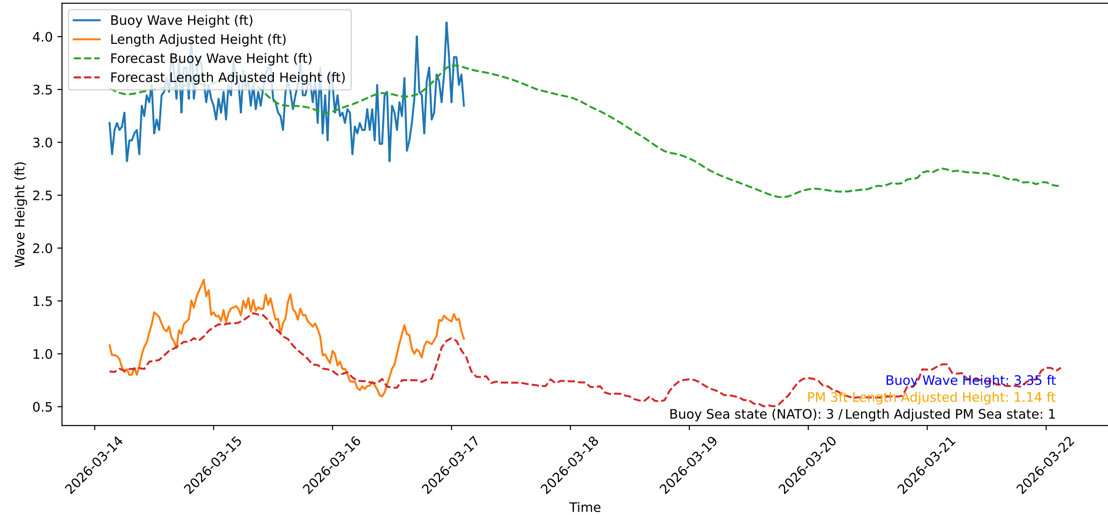
Wave Heights over Time for Green Beach at 2026-03-17 03:11:43
