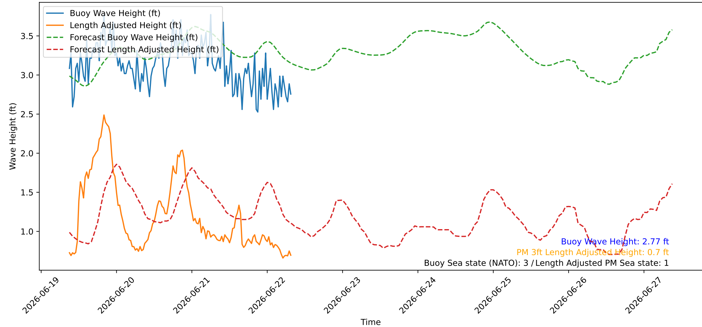
Wave Heights over Time for Red Beach at 2026-06-22 08:40:45
