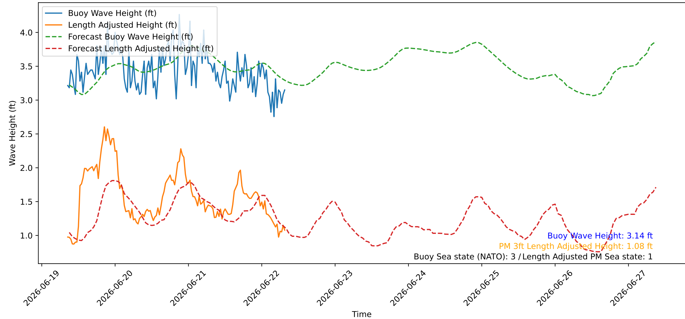
Wave Heights over Time for Oceanside Harbor at 2026-06-22 08:40:25
