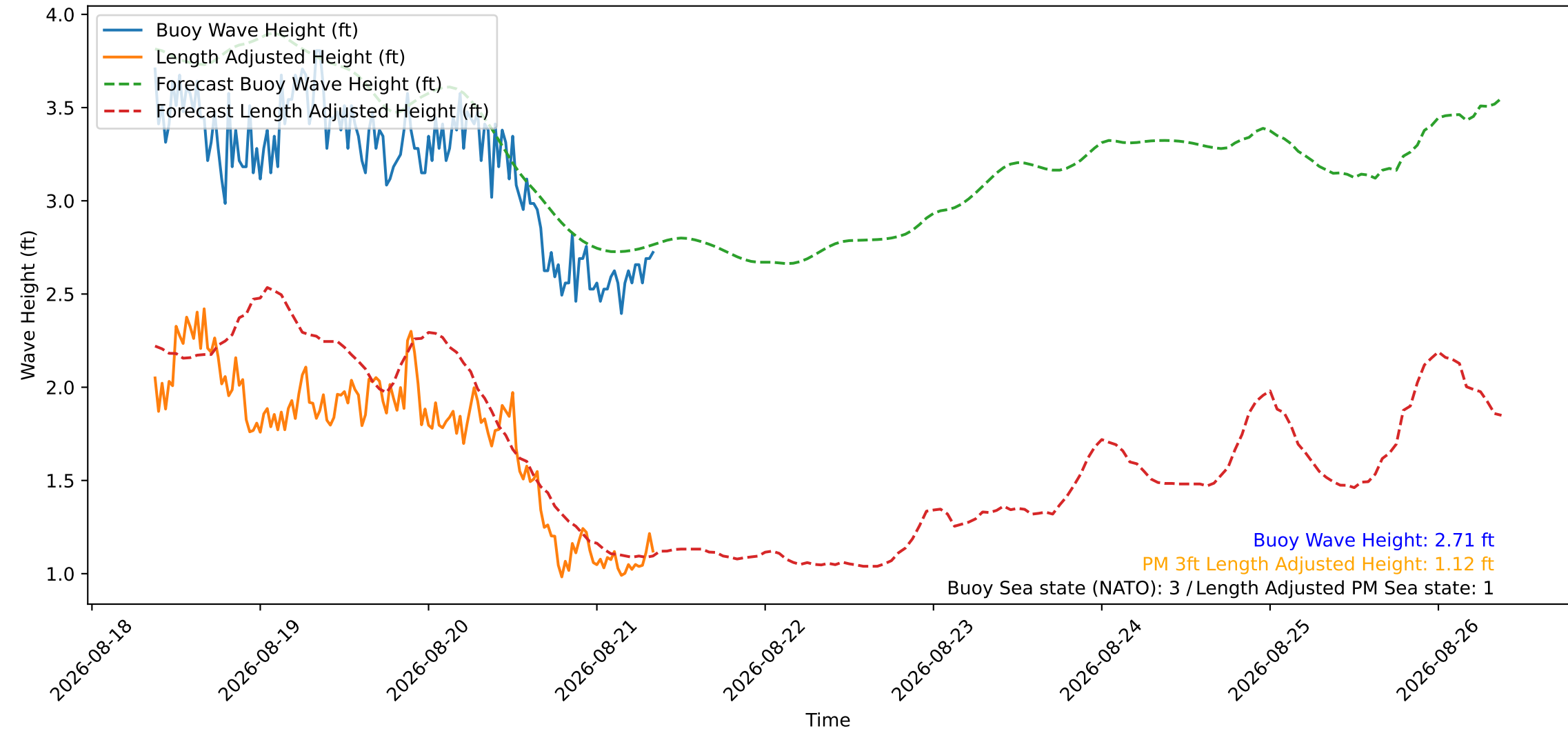
Wave Heights over Time for Oceanside Harbor at 2026-08-21 08:50:27
