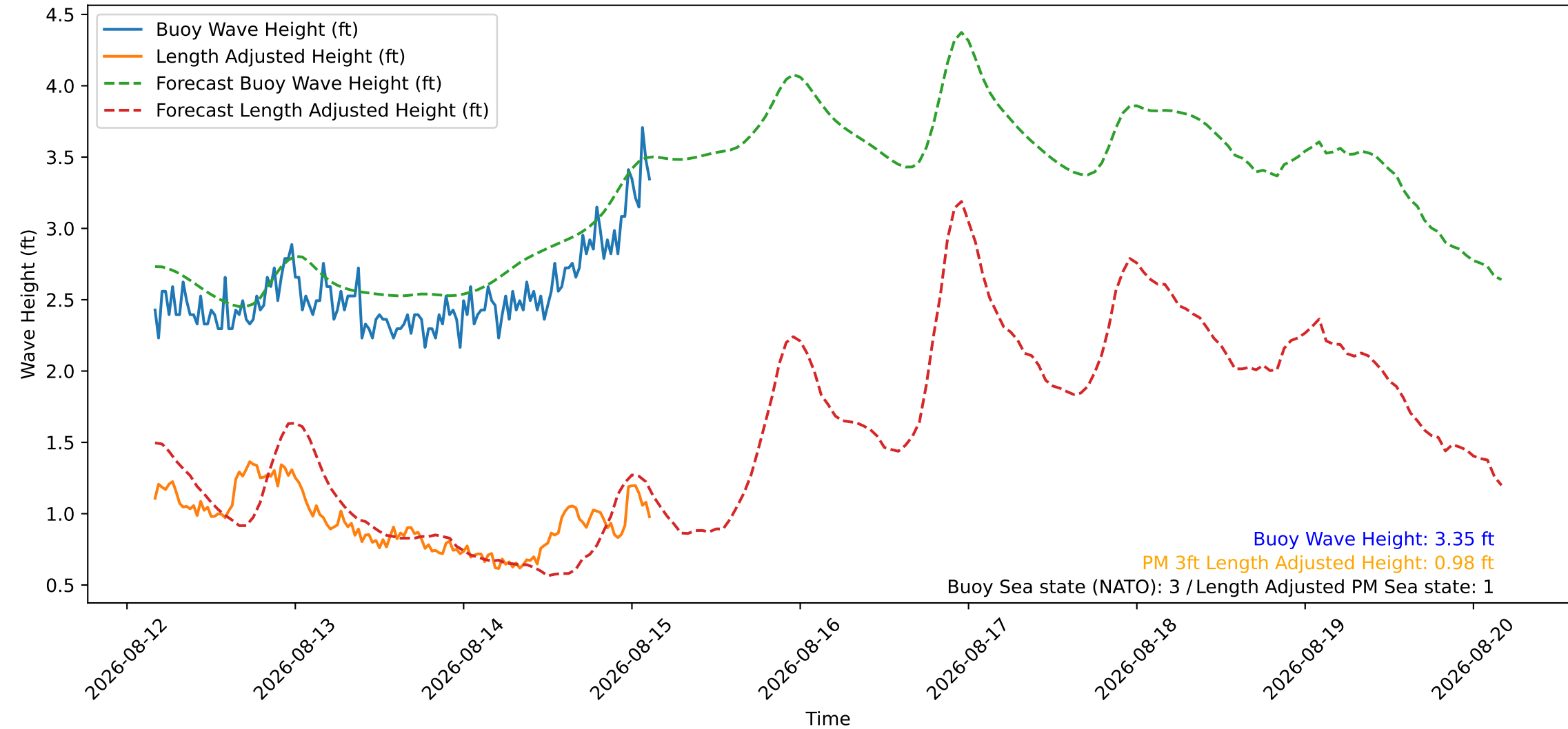
Wave Heights over Time for Red Beach at 2026-08-15 03:30:47
