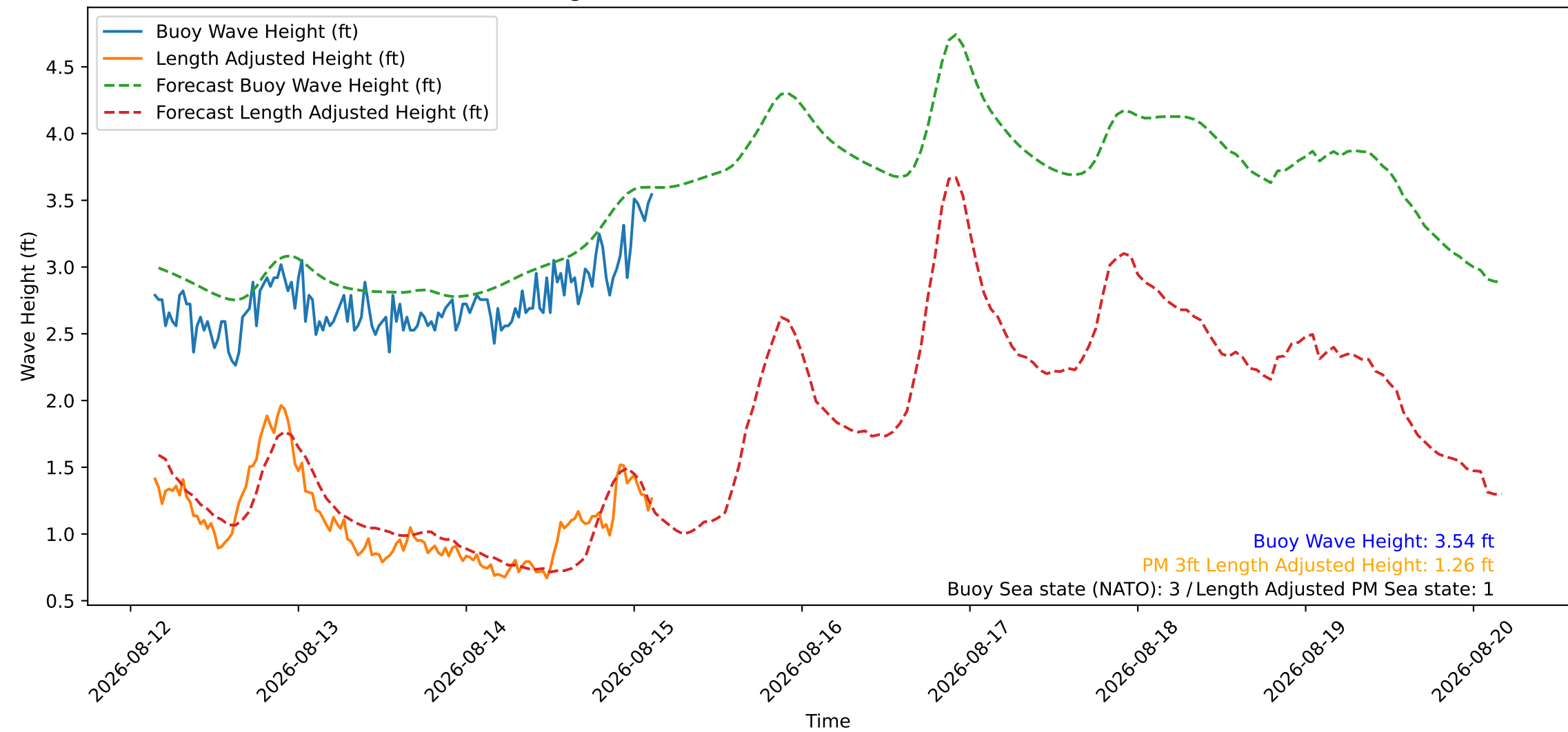
Wave Heights over Time for Green Beach at 2026-08-15 03:31:09
