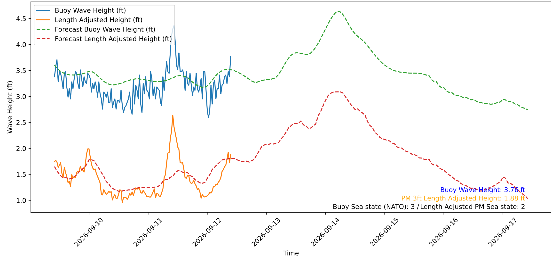
Wave Heights over Time for Oceanside Harbor at 2026-09-12 10:10:30
