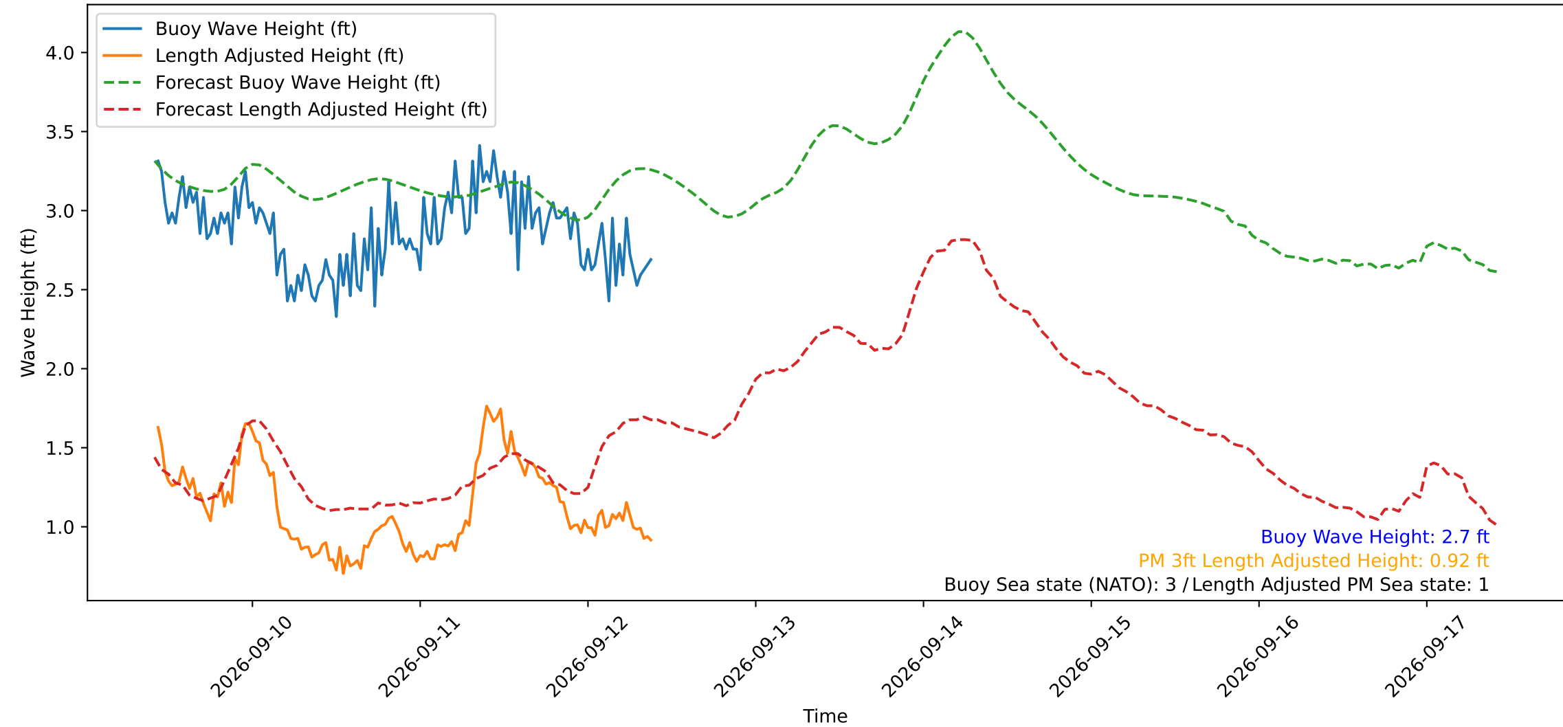
Wave Heights over Time for Red Beach at 2026-09-12 10:10:50
