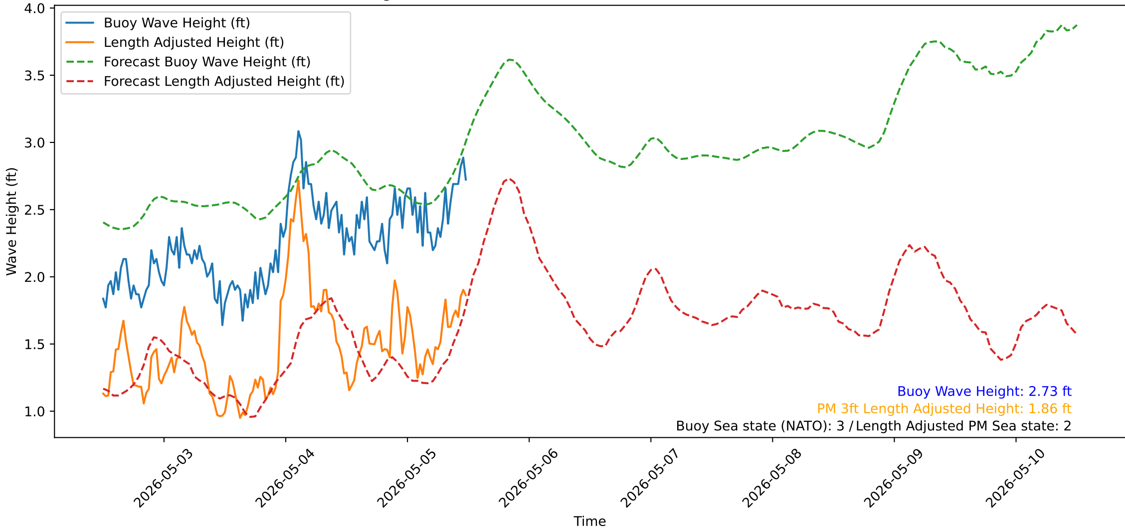
Wave Heights over Time for Oceanside Harbor at 2026-05-05 12:10:32
