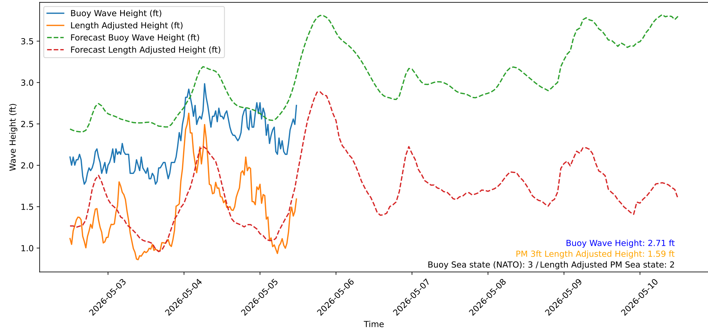
Wave Heights over Time for Green Beach at 2026-05-05 12:11:13
