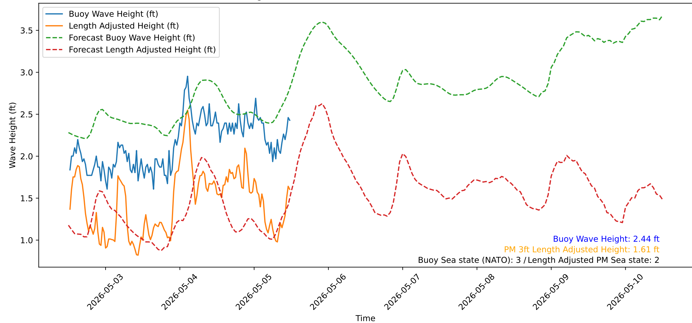
Wave Heights over Time for Red Beach at 2026-05-05 12:10:51
