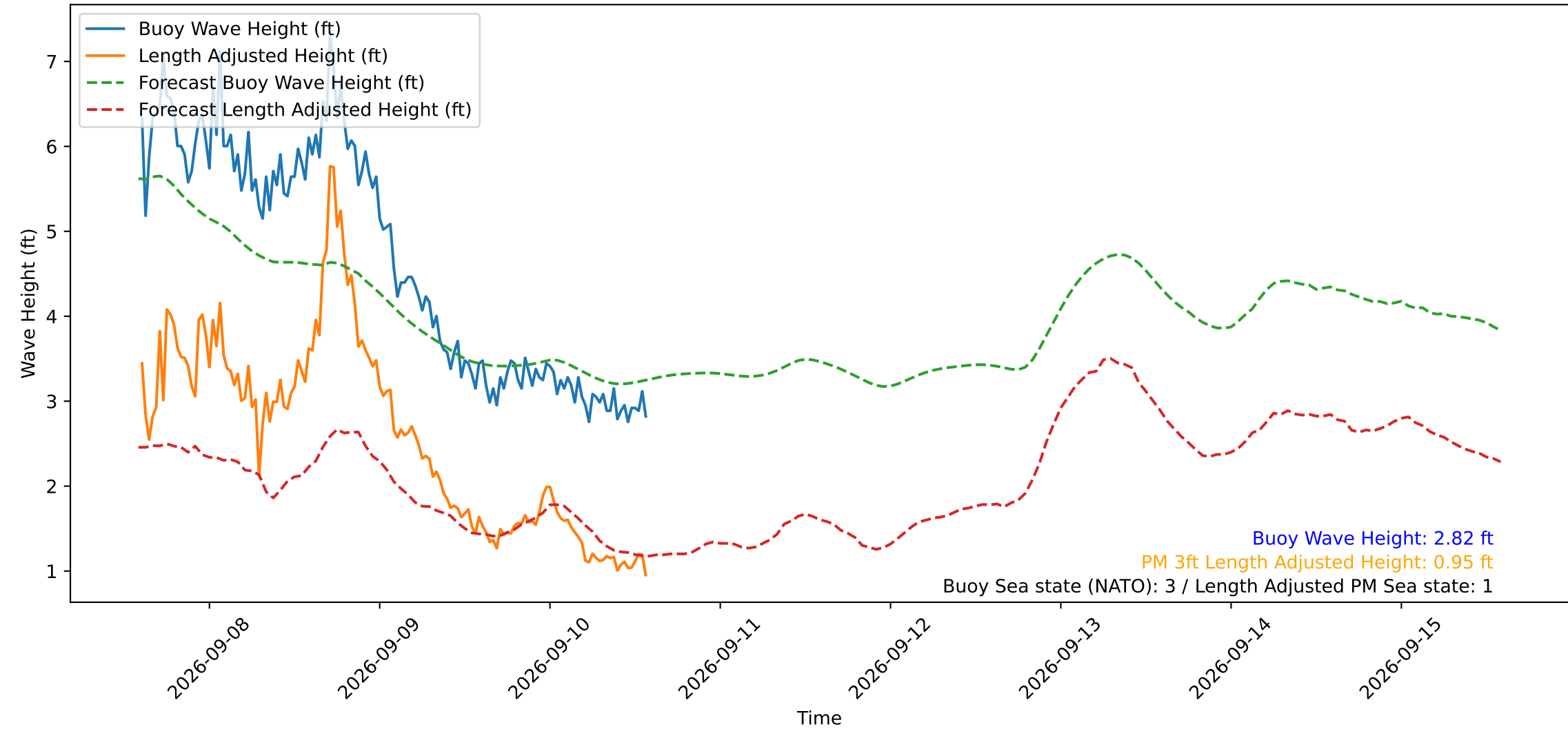
Wave Heights over Time for Oceanside Harbor at 2026-09-10 14:20:30
