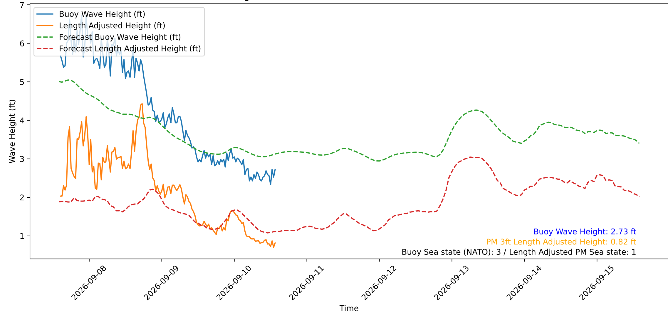
Wave Heights over Time for Red Beach at 2026-09-10 14:20:50
