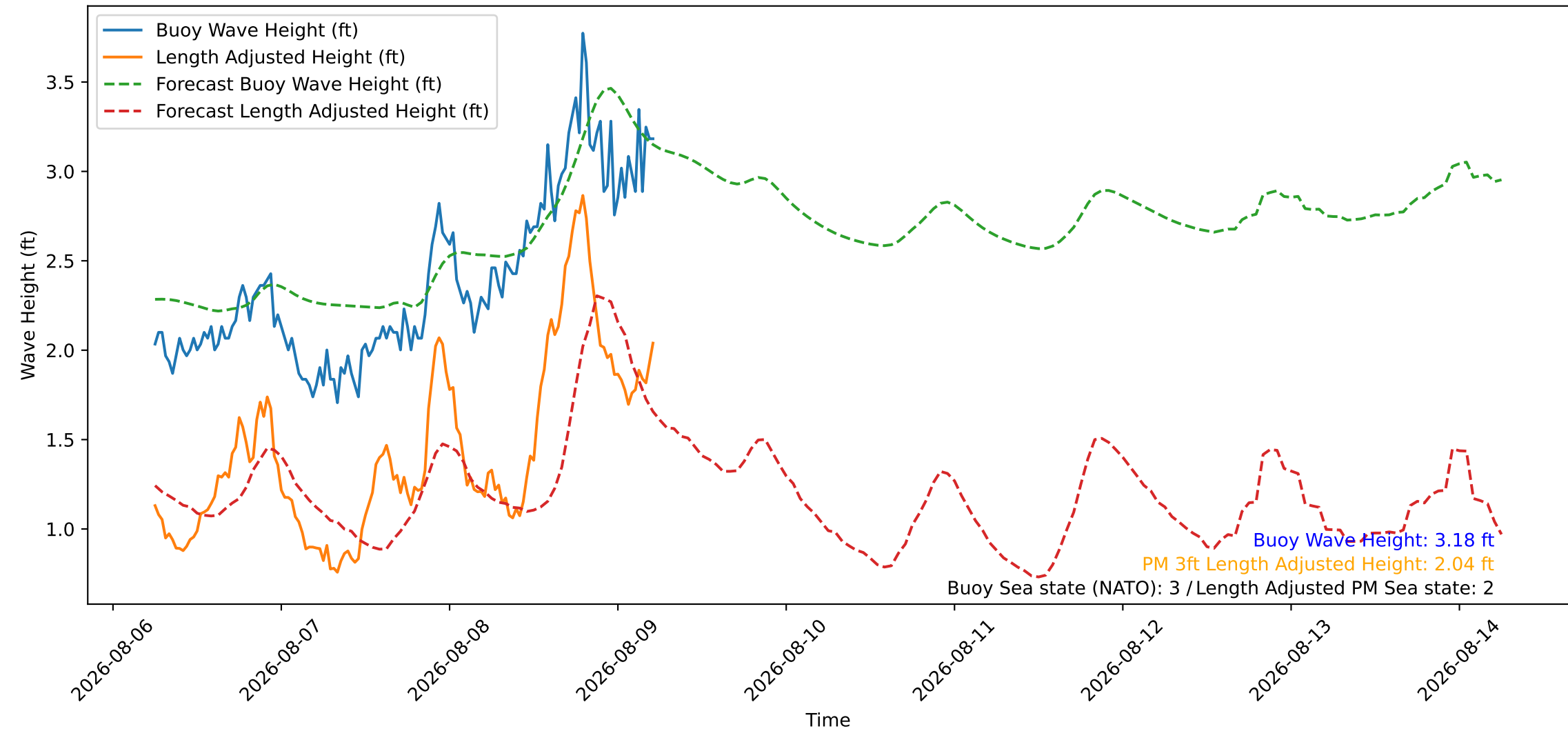
Wave Heights over Time for Green Beach at 2026-08-09 06:01:08
