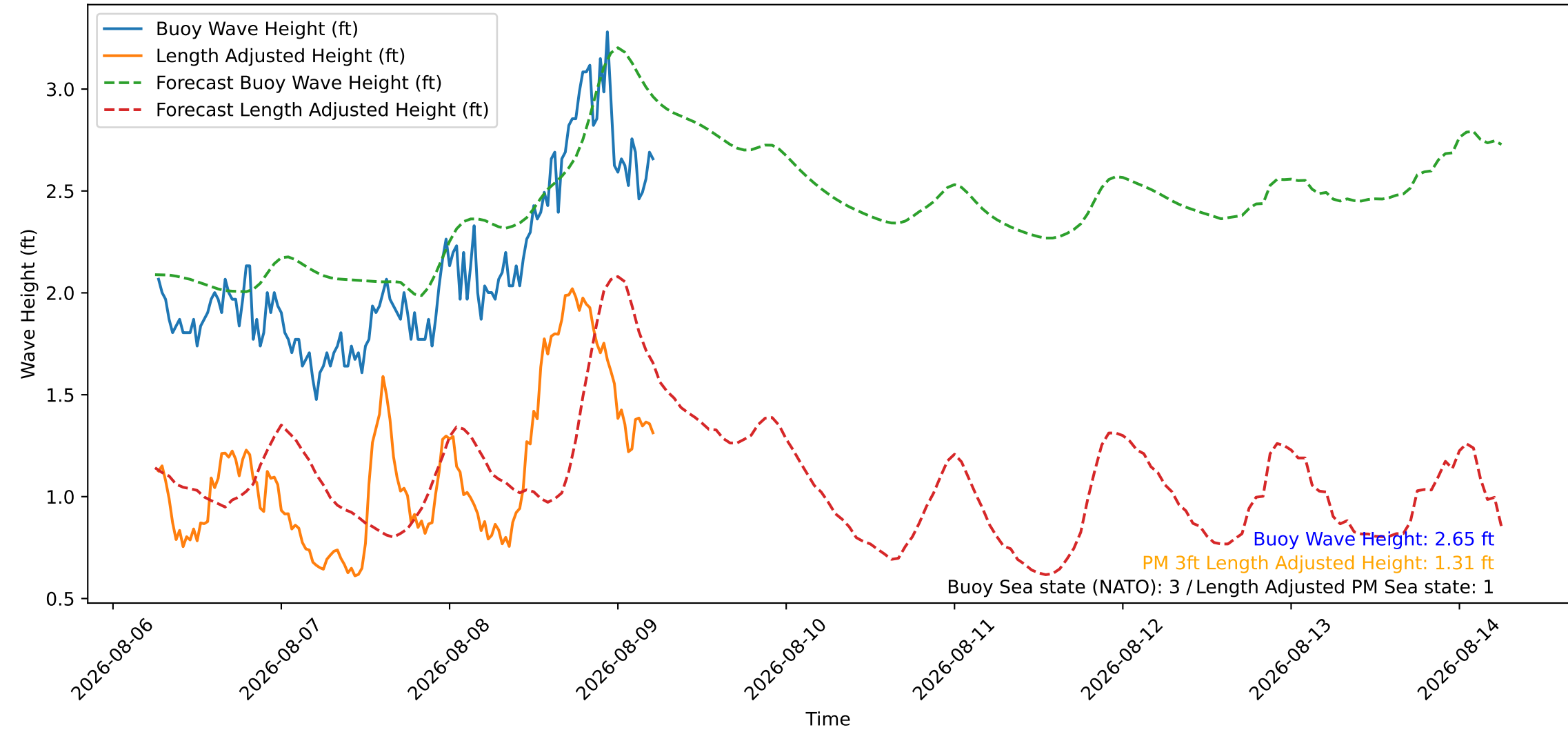
Wave Heights over Time for Red Beach at 2026-08-09 06:00:46
