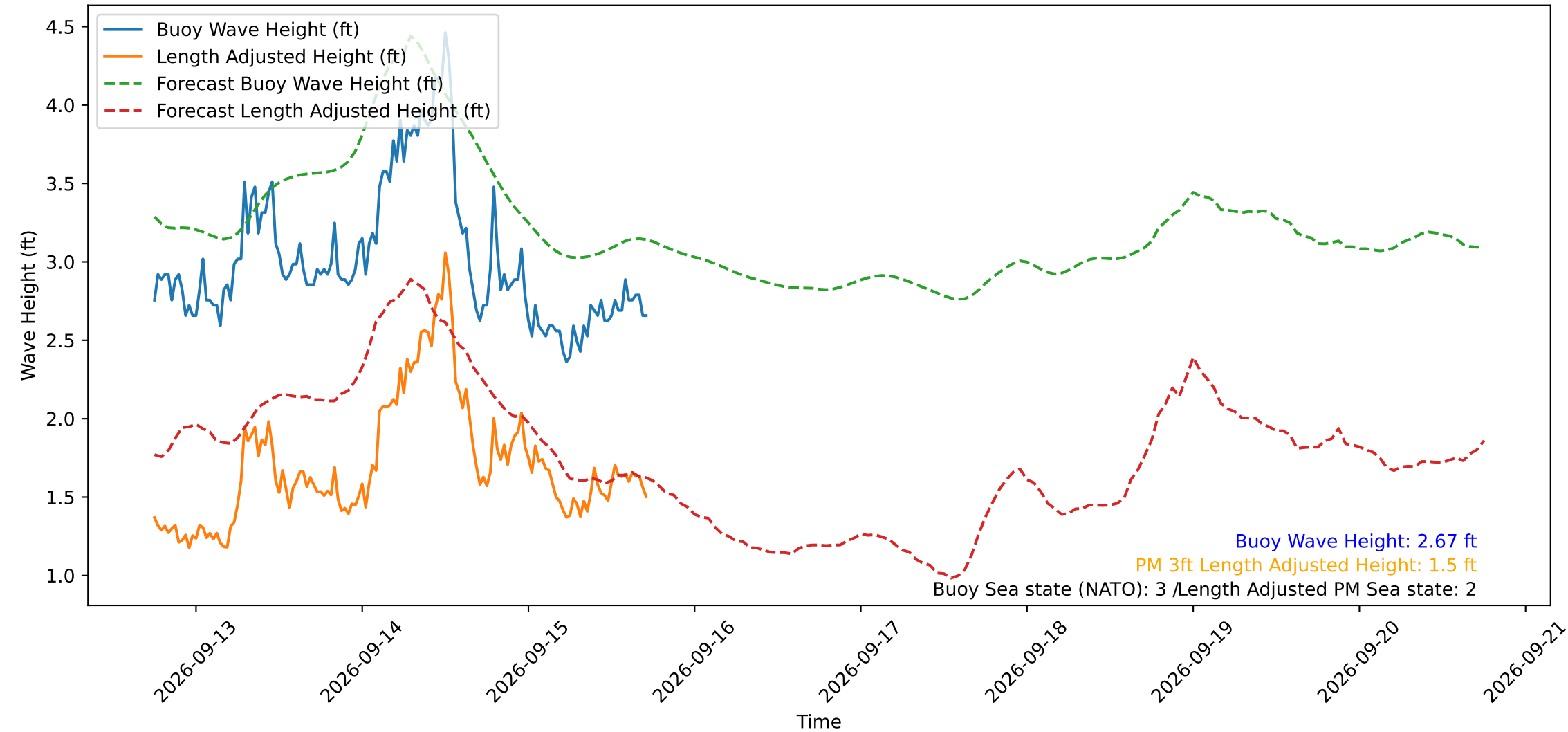
Wave Heights over Time for Oceanside Harbor at 2026-09-15 17:50:29
