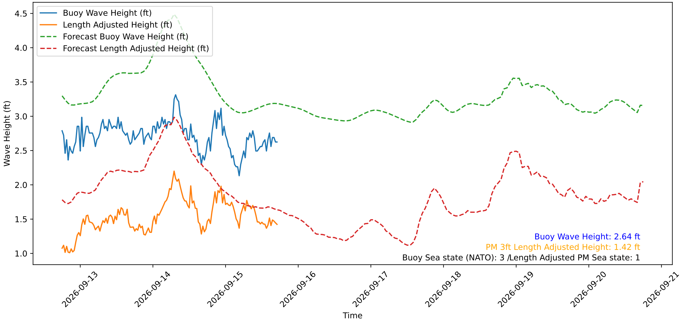
Wave Heights over Time for Green Beach at 2026-09-15 17:51:14
