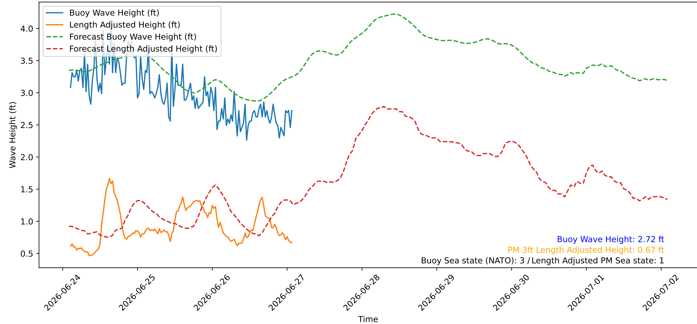
Wave Heights over Time for Red Beach at 2026-06-27 02:10:46
