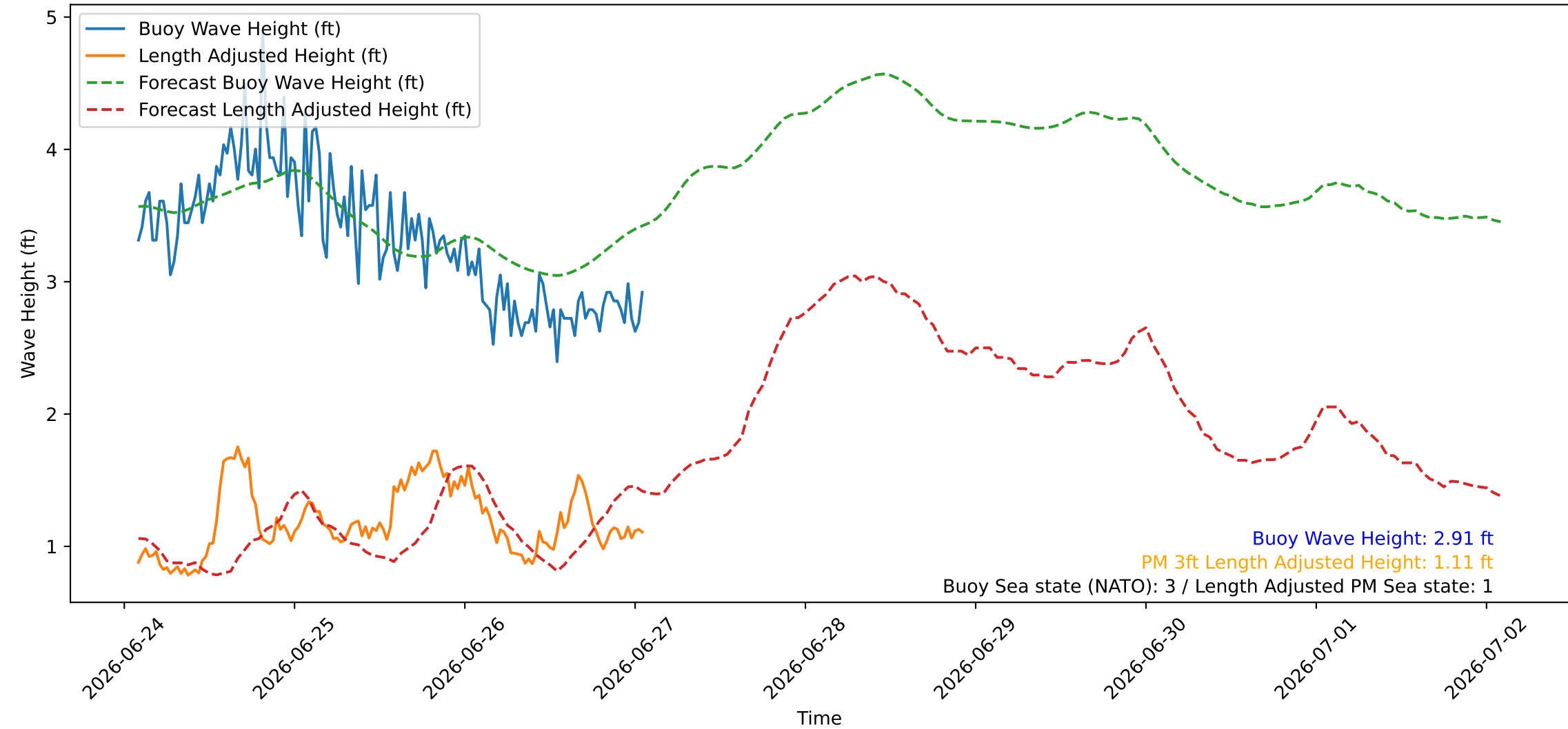
Wave Heights over Time for Oceanside Harbor at 2026-06-27 02:10:26
