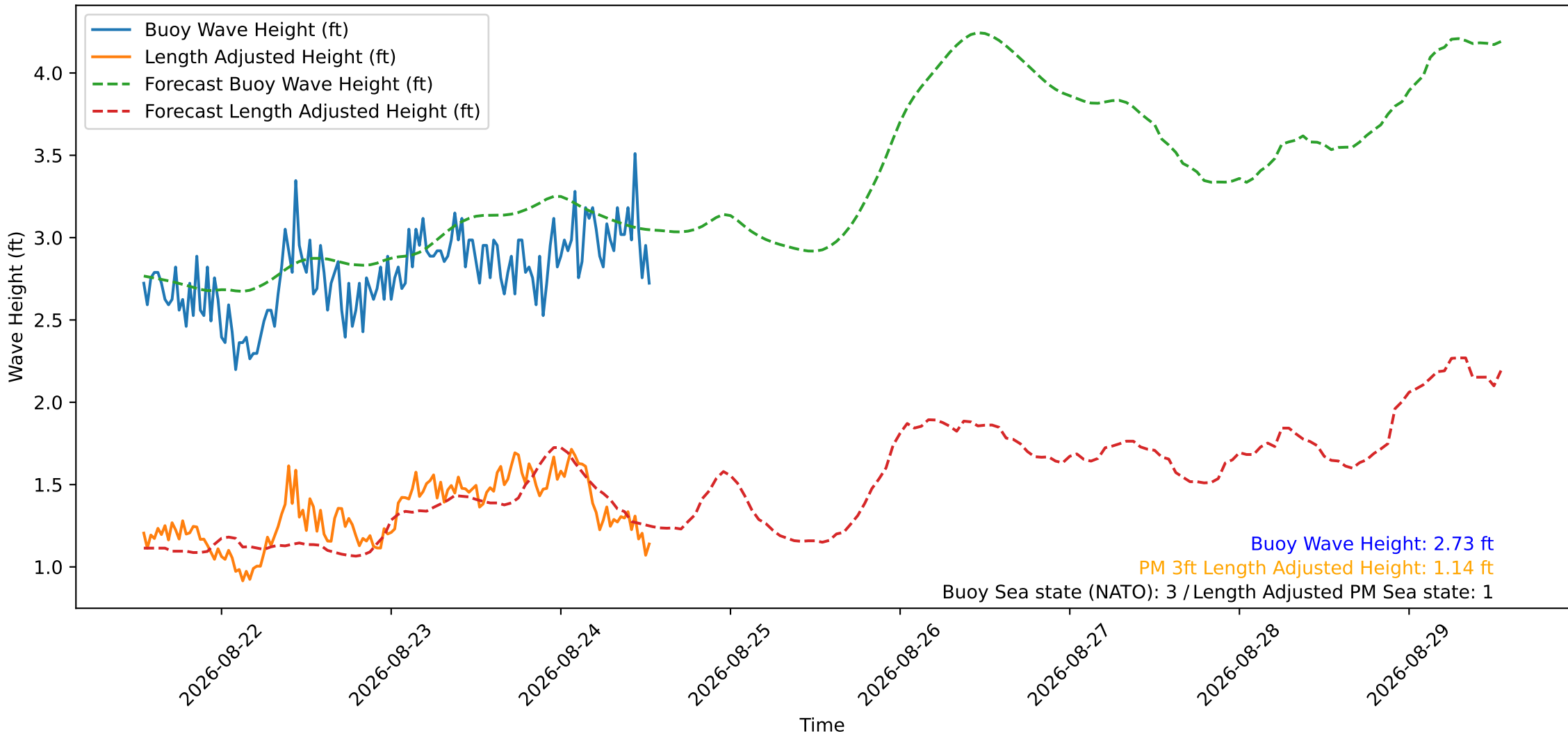
Wave Heights over Time for Oceanside Harbor at 2026-08-24 13:10:29
