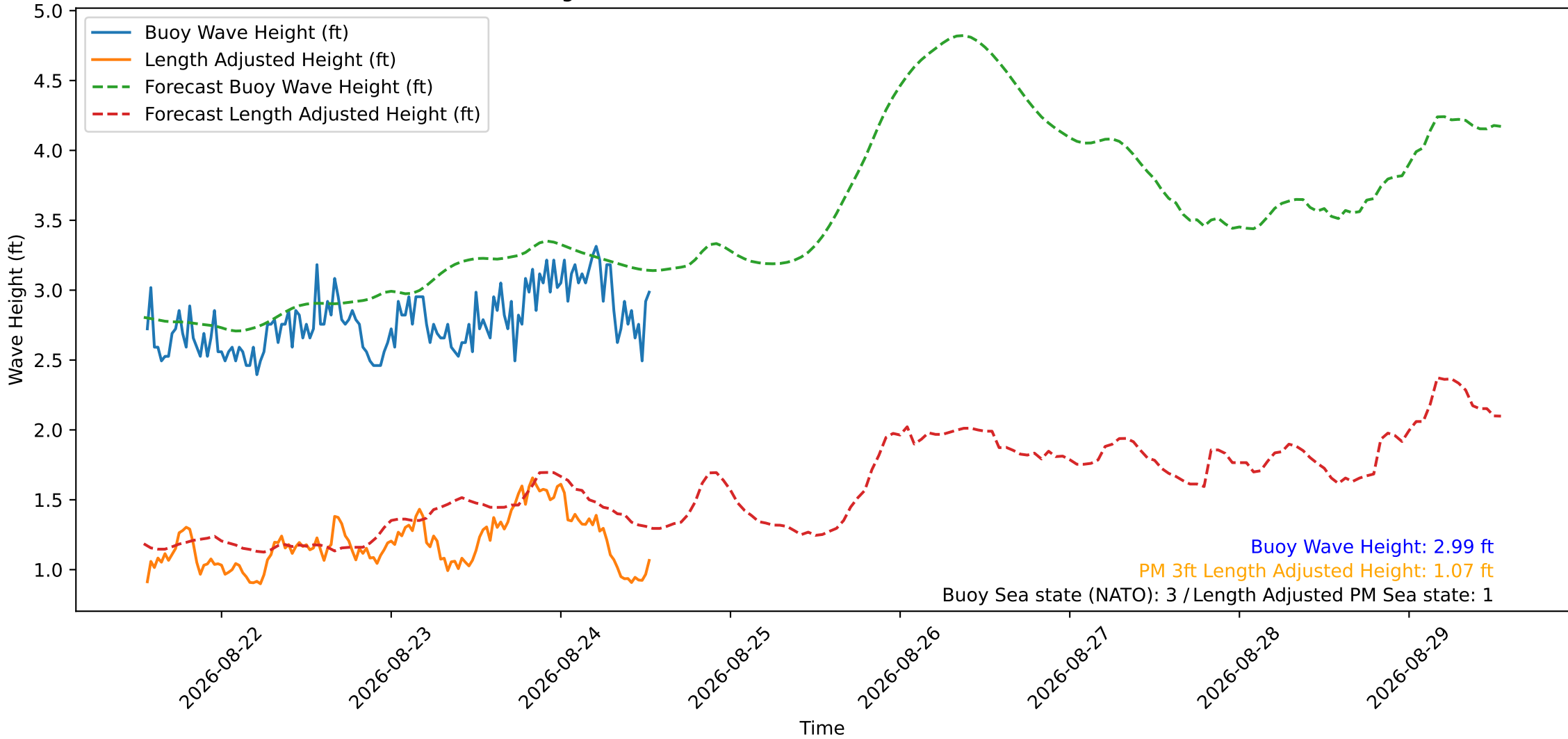
Wave Heights over Time for Green Beach at 2026-08-24 13:11:11
