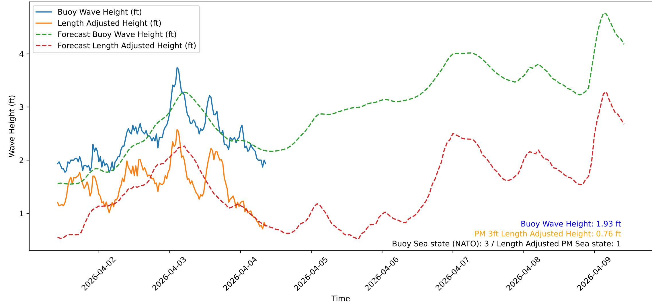
Wave Heights over Time for Red Beach at 2026-04-04 09:30:47
