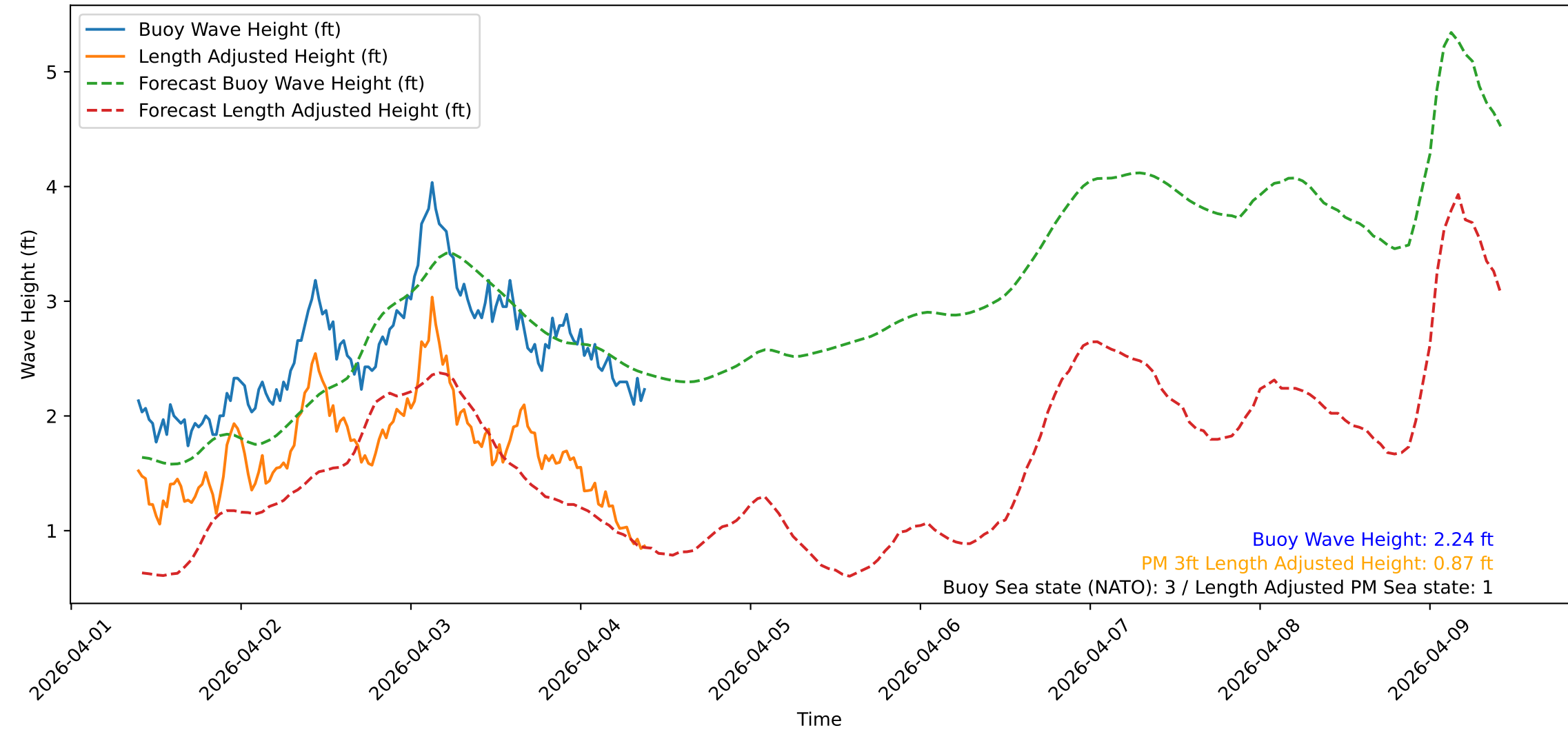
Wave Heights over Time for Oceanside Harbor at 2026-04-04 09:30:31
