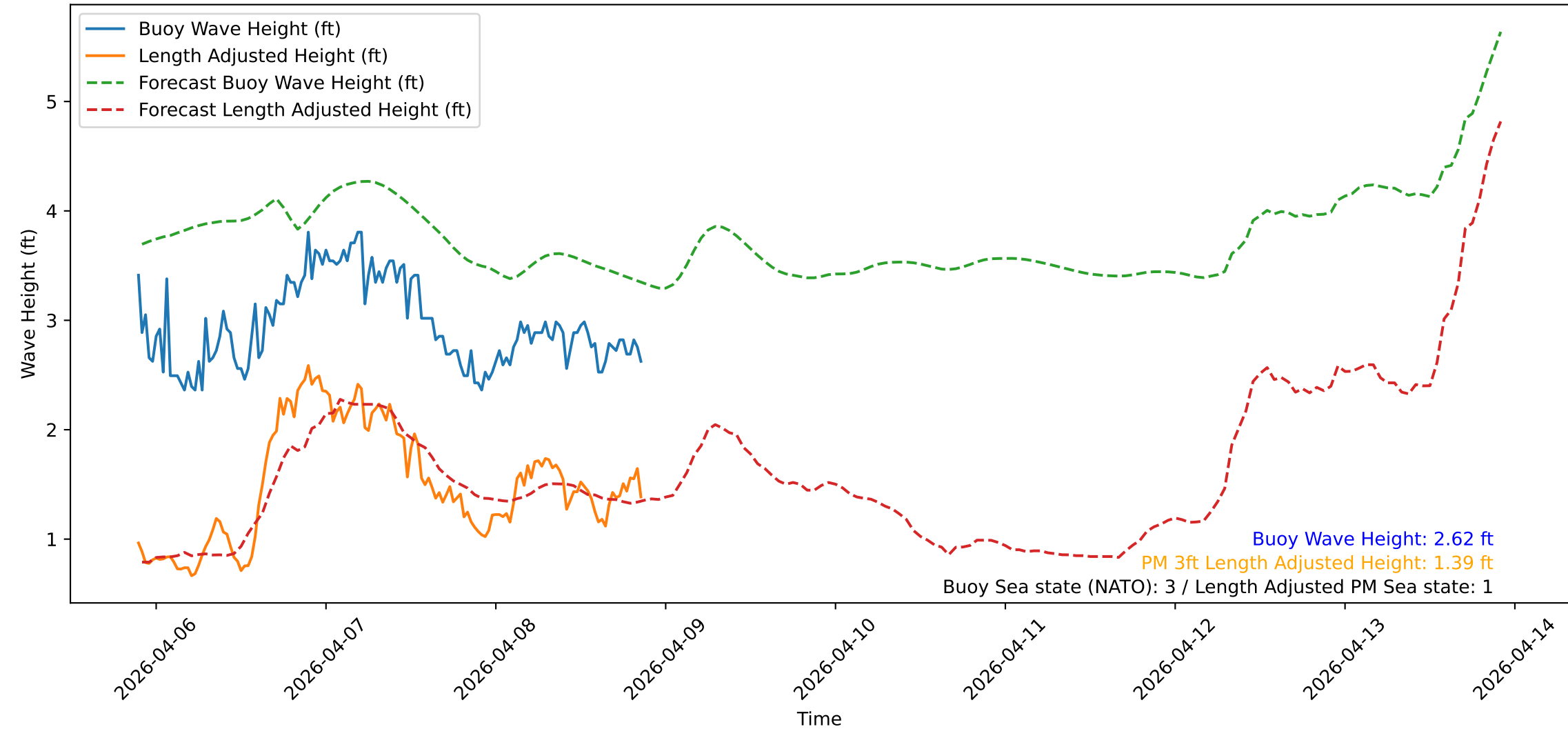
Wave Heights over Time for Green Beach at 2026-04-08 21:31:09
