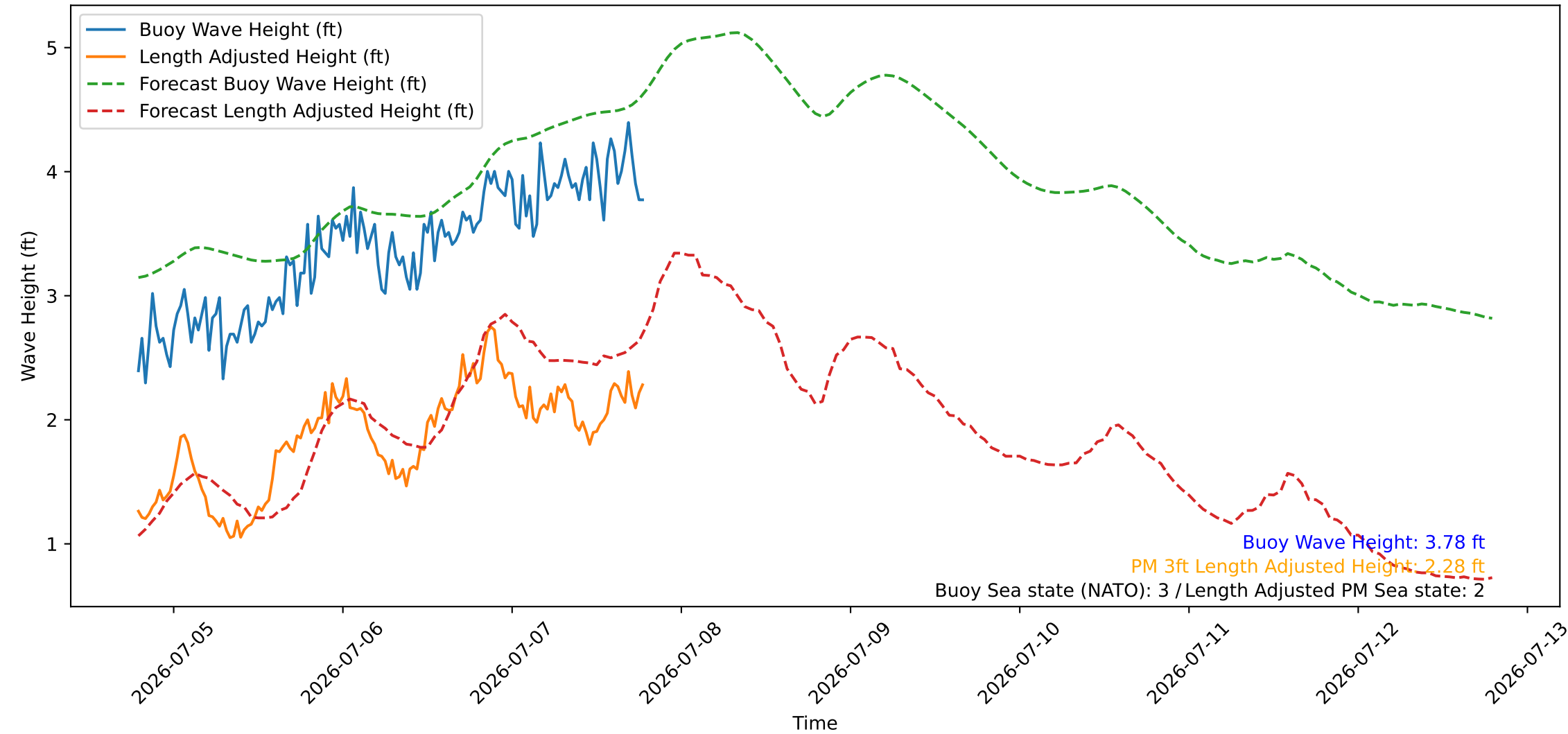
Wave Heights over Time for Oceanside Harbor at 2026-07-07 19:10:25
