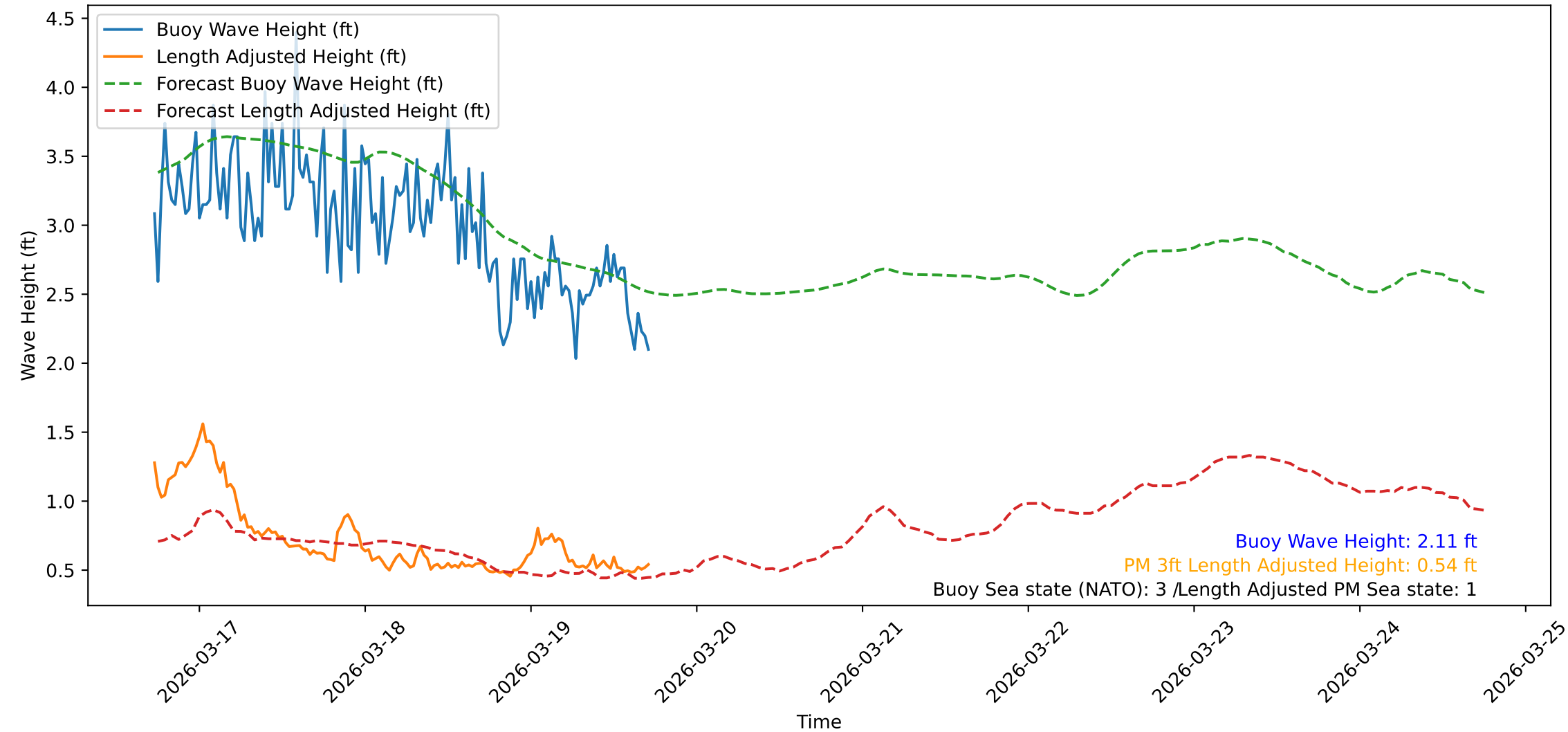
Wave Heights over Time for Oceanside Harbor at 2026-03-19 17:30:32
