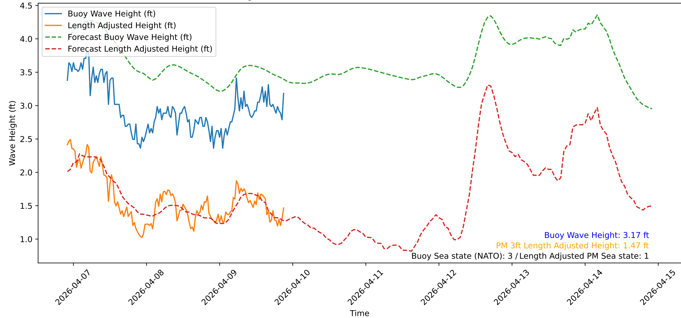
Wave Heights over Time for Green Beach at 2026-04-09 21:51:09
