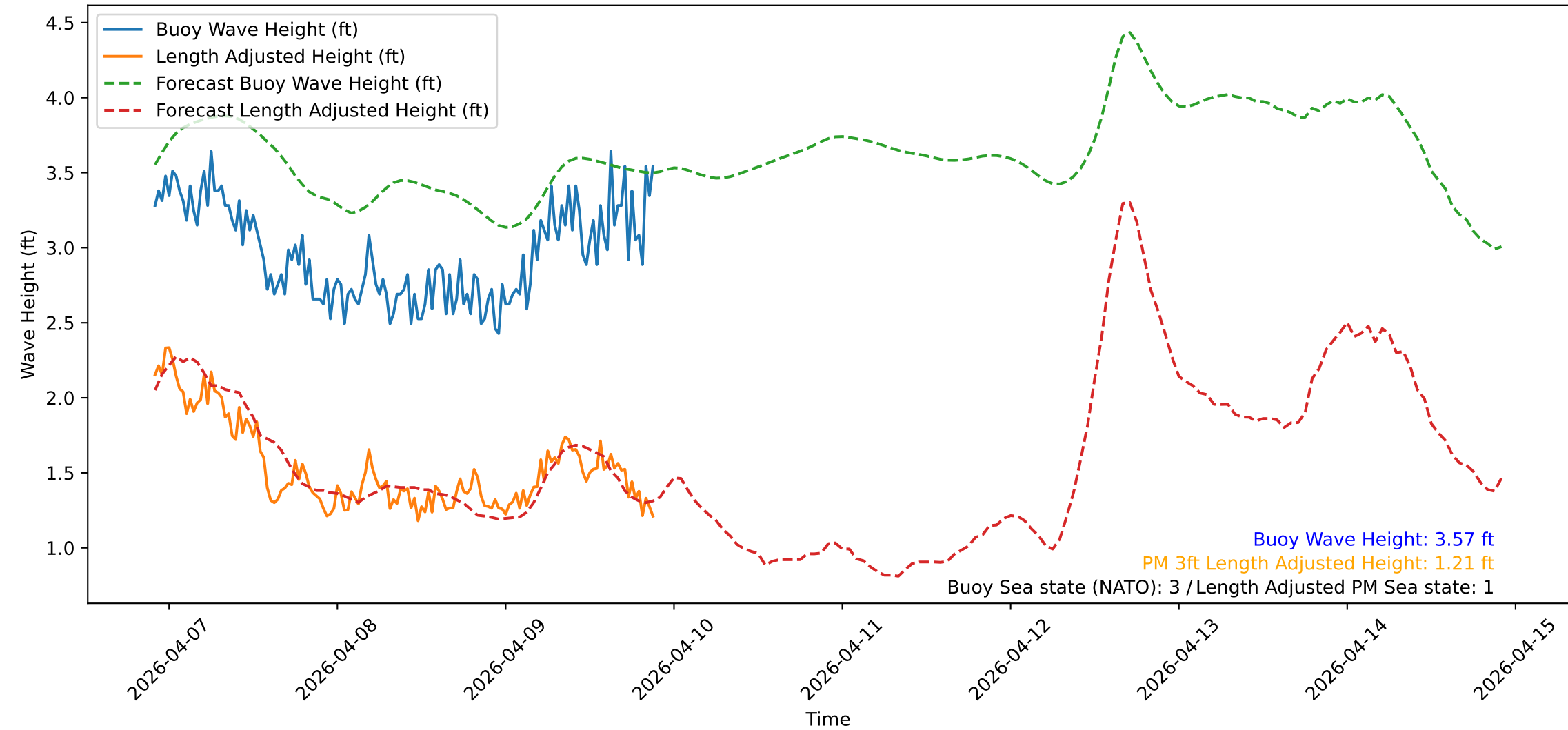
Wave Heights over Time for Oceanside Harbor at 2026-04-09 21:50:31
