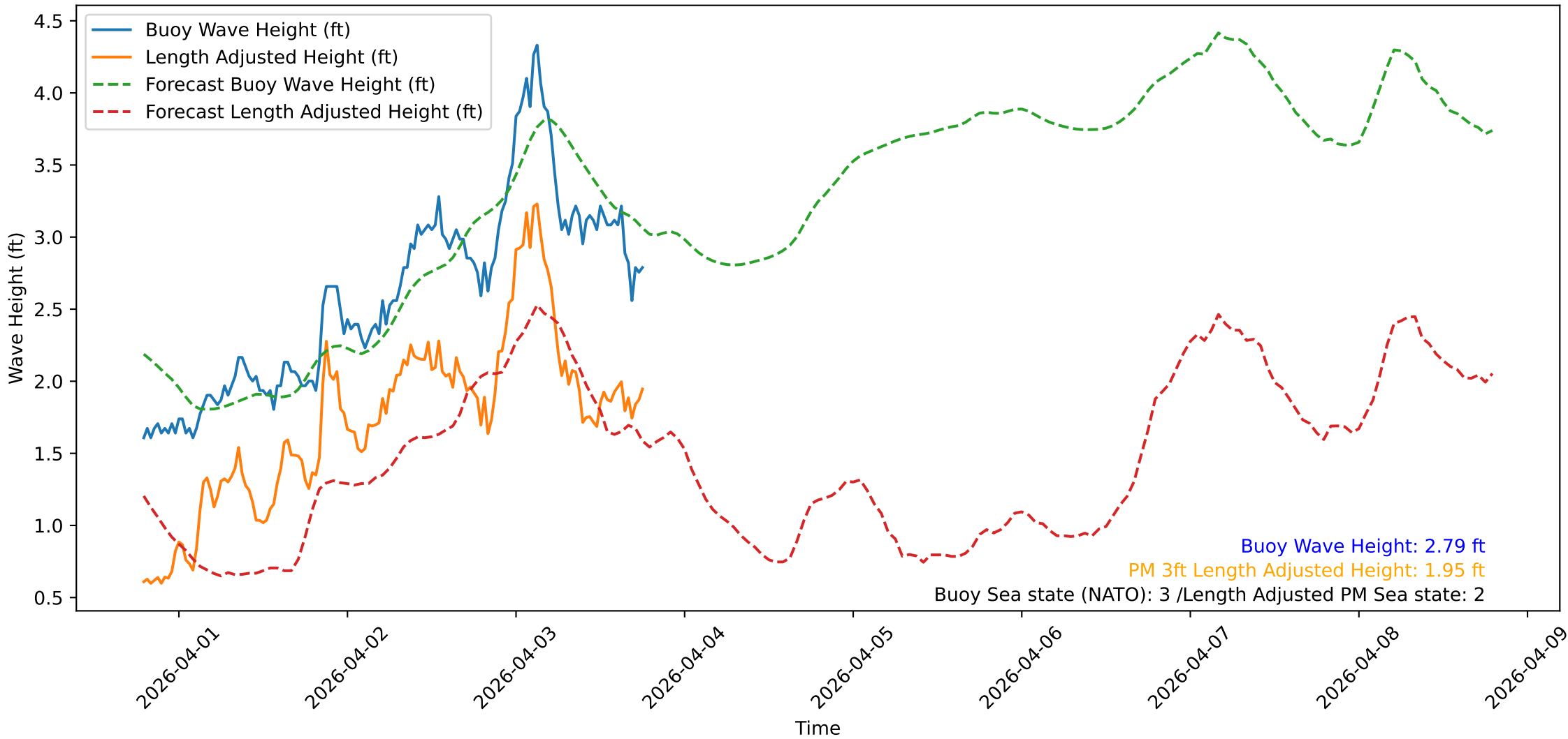
Wave Heights over Time for Green Beach at 2026-04-03 18:51:15
