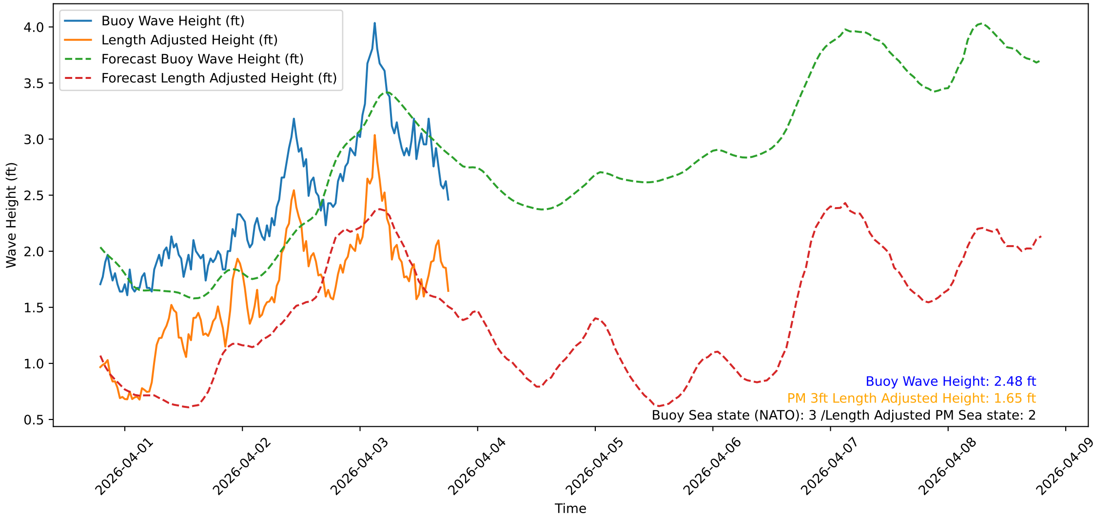
Wave Heights over Time for Oceanside Harbor at 2026-04-03 18:50:33
