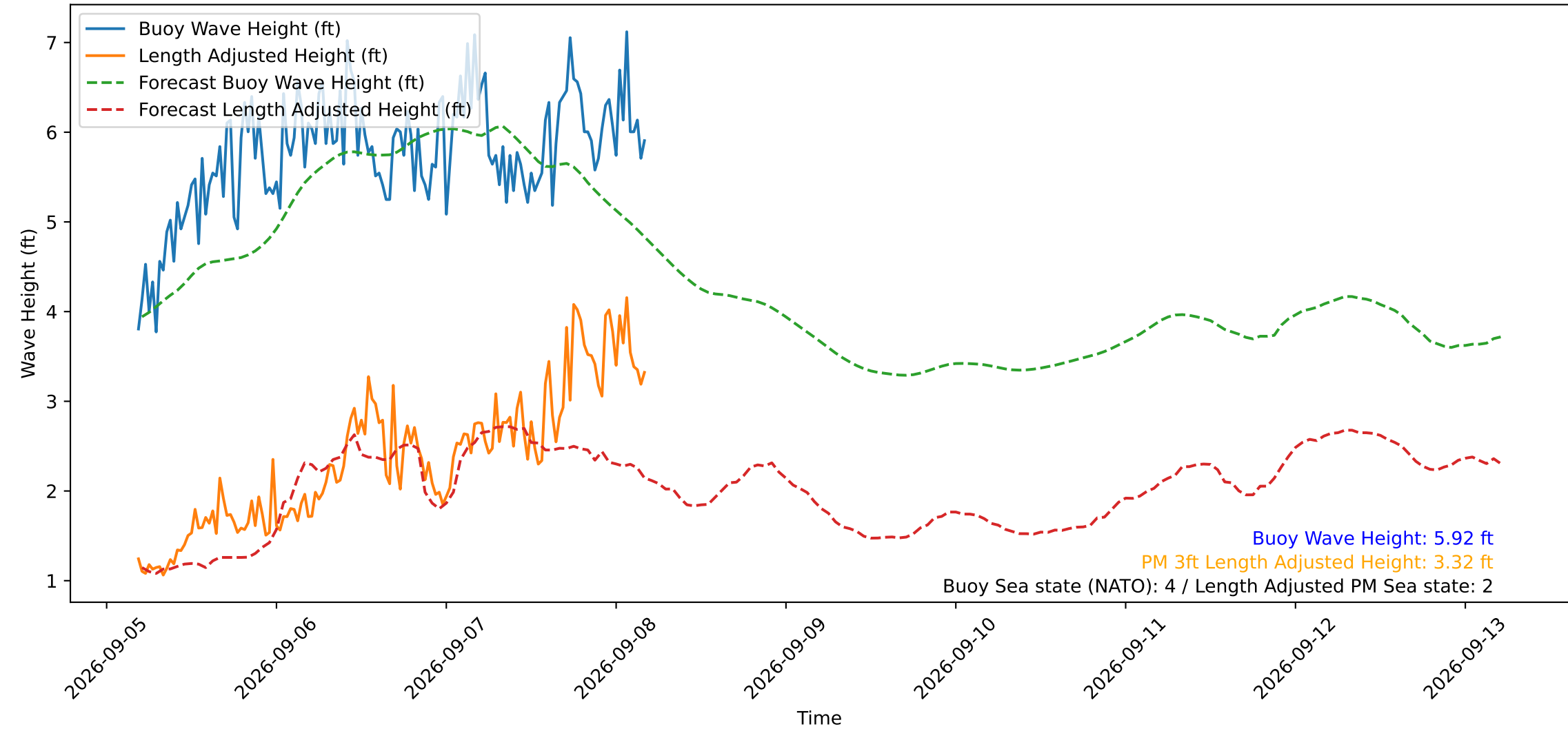
Wave Heights over Time for Oceanside Harbor at 2026-09-08 04:30:30
