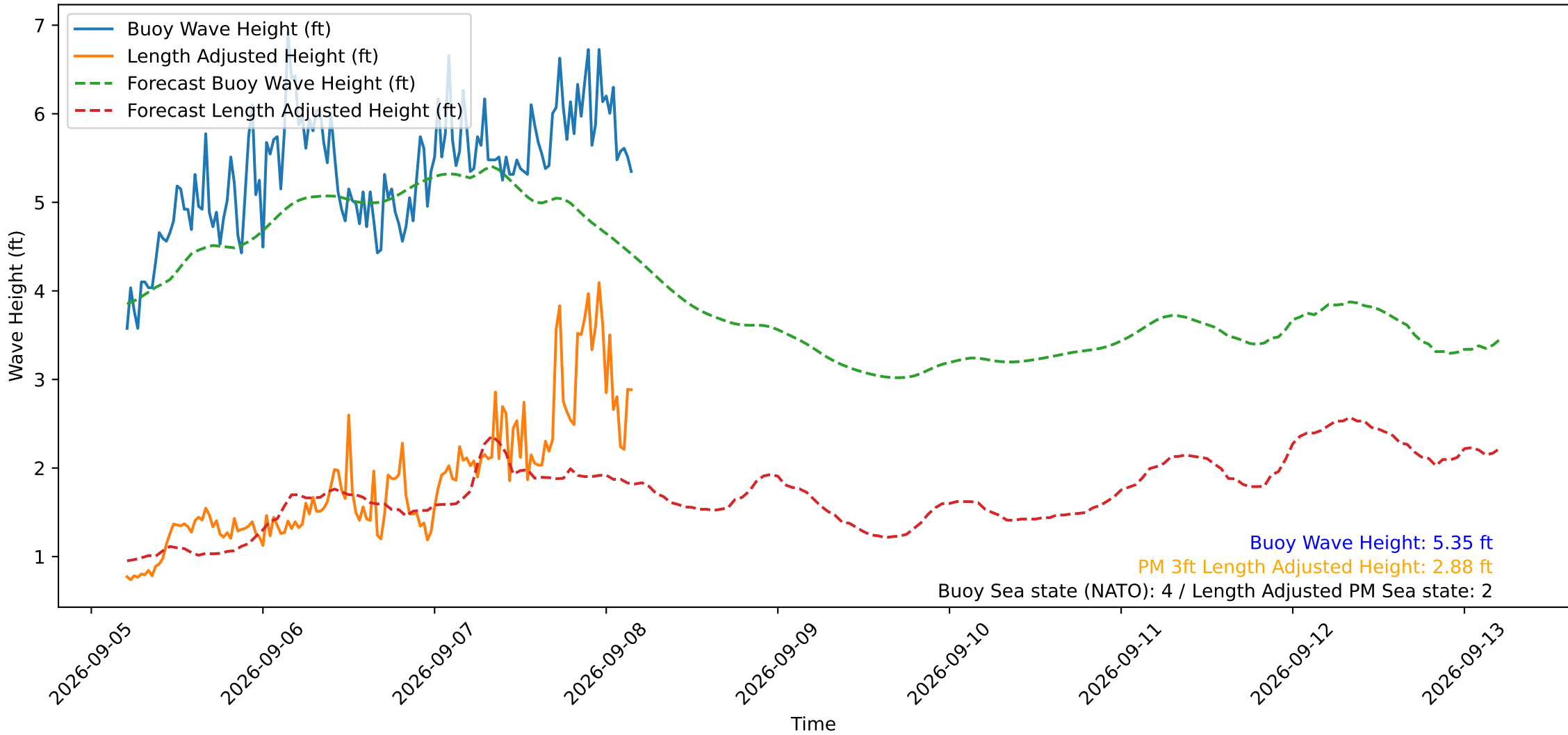
Wave Heights over Time for Red Beach at 2026-09-08 04:30:49
